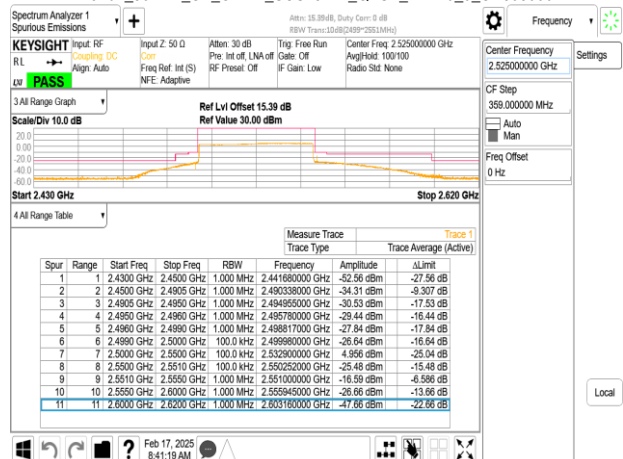
Band7_50MHz_CP_OFDM_SCS15kHz_QPSK_RB270_0_CH505000
