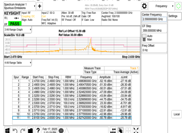
Band7_40MHz_CP_OFDM_SCS30kHz_QPSK_RB1_105_CH510000
