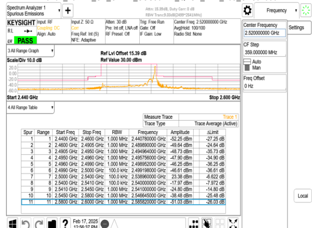
Band7 40MHz_CP_OFDM_SCS30kHz_QPSK_RB1_105_CH504000
