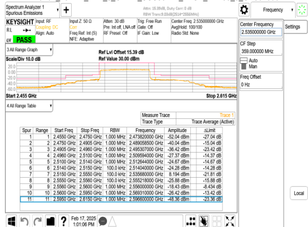
Band7_40MHz_DFT_s_OFDM_SCS30kHz_BPSK_RB1_0_CH507000
