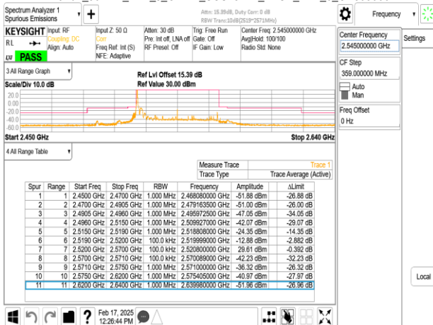
Band7_50MHz_DFT_s_OFDM_SCS15kHz_BPSK_RB1_269_CH509000
