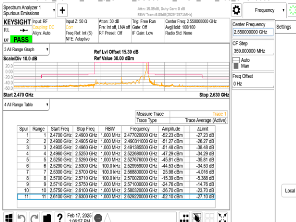
Band7 40MHz_DFT_s_OFDM_SCS30kHz_BPSK_RB1_105_CH510000
