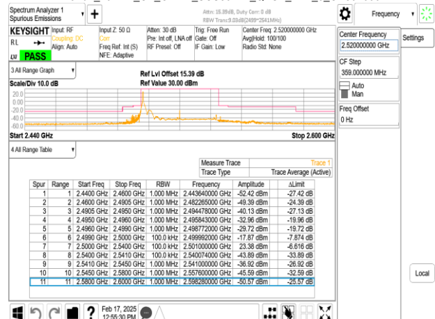
Band7 40MHz_CP_OFDM_SCS30kHz_QPSK_RB1_105_CH504000
