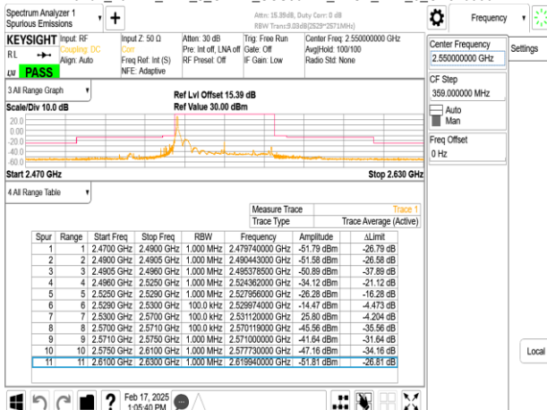
Band7 40MHz_DFT_s_OFDM_SCS30kHz_BPSK_RB1_105_CH510000
