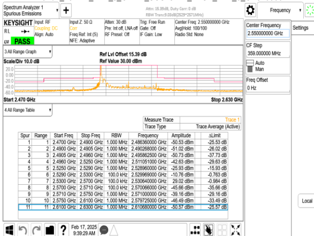
Band7_40MHz_DFT_s_OFDM_SCS15kHz_BPSK_RB1_215_CH510000
