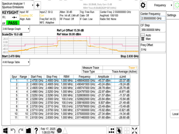
Band7 40MHz_DFT_s_OFDM_SCS30kHz_BPSK_RB1_0_CH510000
