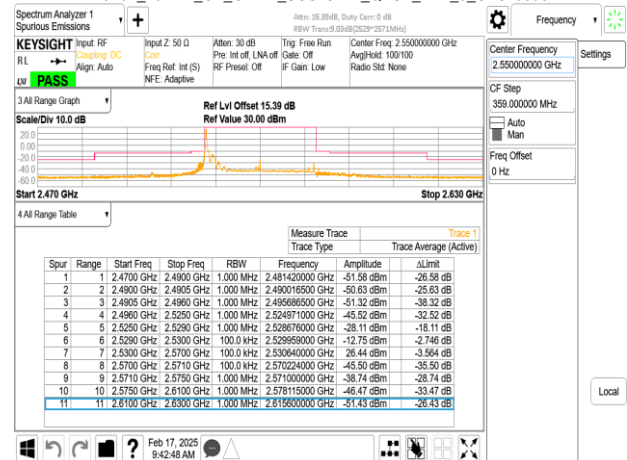
Band7_40MHz_CP_OFDM_SCS15kHz_QPSK_RB1_215_CH510000
