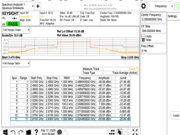
Band7_40MHz_DFT_s_OFDM_SCS15kHz_BPSK_RB216_0_CH510000
