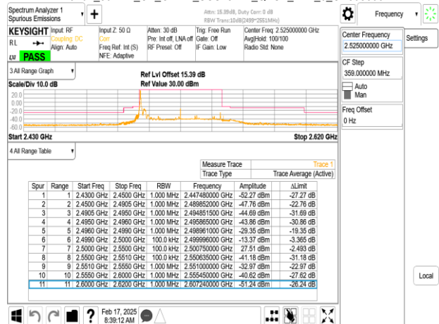
Band7_50MHz_CP_OFDM_SCS15kHz_QPSK_RB1_269_CH505000
