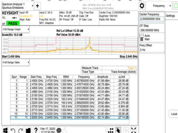
Band7_50MHz_DFT_s_OFDM_SCS15kHz_BPSK_RB270_0_CH509000
