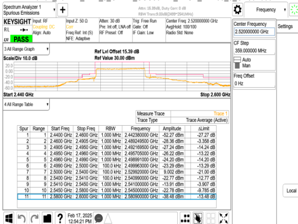
Band7_40MHz_DFT_s_OFDM_SCS30kHz_BPSK_RB1_0_CH504000
