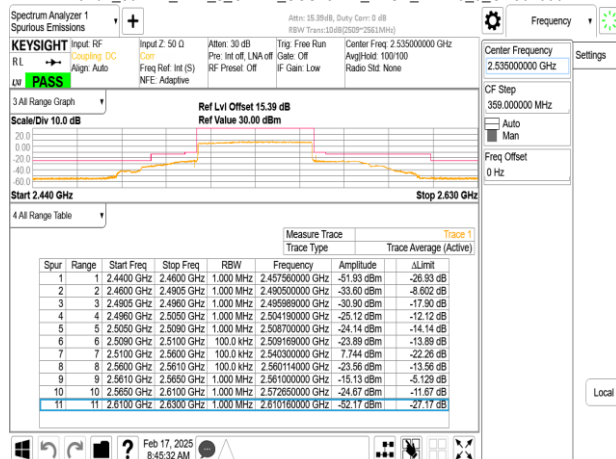
Band7_50MHz_DFT_s_OFDM_SCS15kHz_BPSK_RB270_0_CH507000
