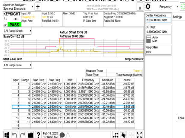
Band7_50MHz_DFT_s_OFDM_SCS15kHz_BPSK_RB1_269_CH507000
