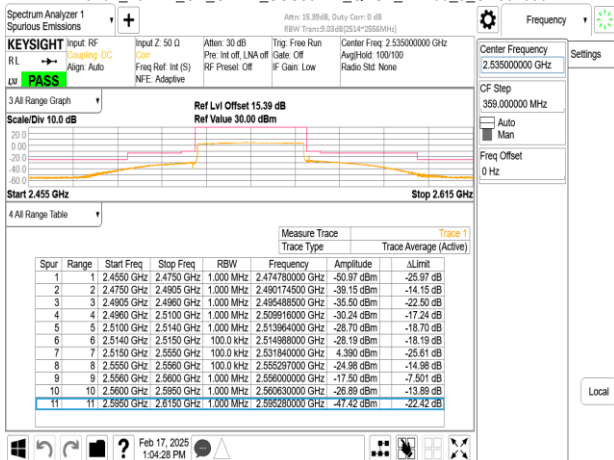
Band7_40MHz_CP_OFDM_SCS30kHz_QPSK_RB1_0_CH507000
