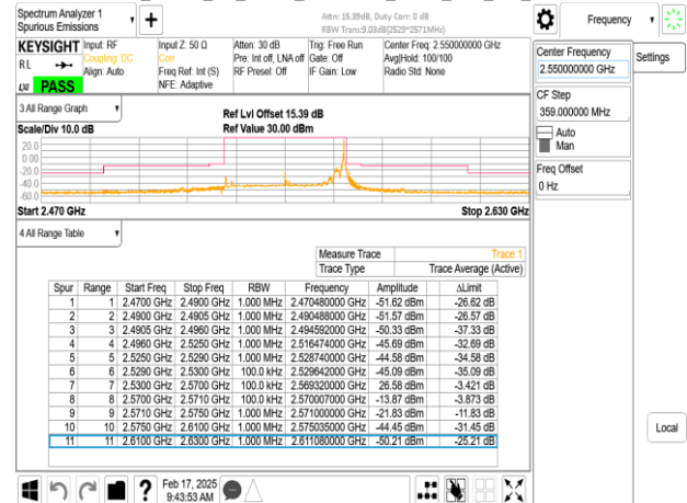
Band7_40MHz_CP_OFDM_SCS15kHz_QPSK_RB216_0_CH510000
