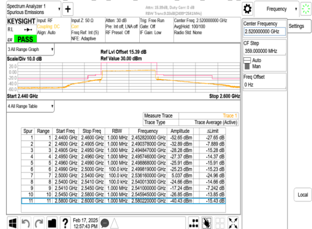
Band7 40MHz_CP_OFDM_SCS30kHz_QPSK_RB1_0_CH504000
