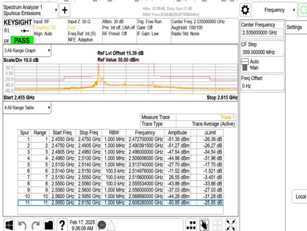
Band7_40MHz_CP_OFDM_SCS15kHz_QPSK_RB1_215_CH507000
