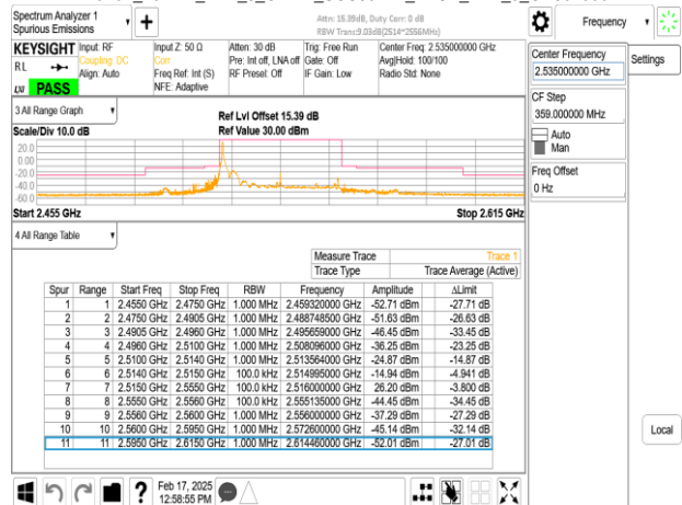
Band7_40MHz_DFT_s_OFDM_SCS30kHz_BPSK_RB1_105_CH507000
