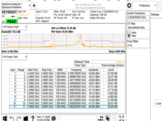
Band7_40MHz_DFT_s_OFDM_SCS30kHz_BPSK_RB1_105_CH504000
