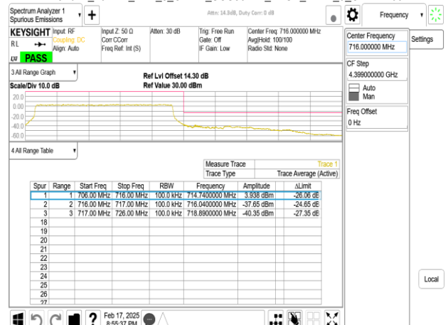
Band12_10MHz_DFT_s_OFDM_SCS30kHz_BPSK_RB24_0_CH142200
