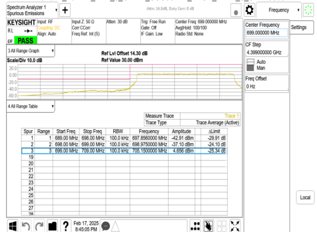
Band12_10MHz_DFT_s_OFDM_SCS30kHz_BPSK_RB1_23_CH142200
