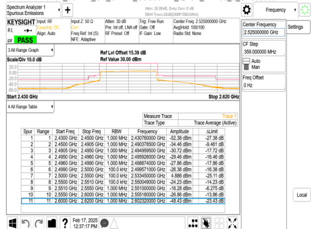
Band7_50MHz_CP_OFDM_SCS30kHz_QPSK_RB1_0_CH505000
