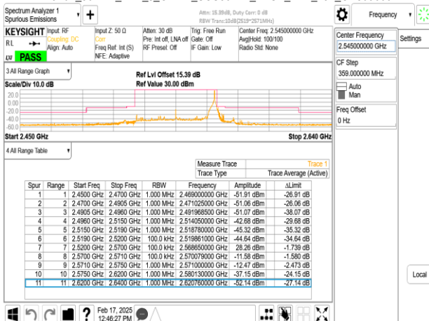
Band7_50MHz_DFT_s_OFDM_SCS30kHz_BPSK_RB1_132_CH509000
