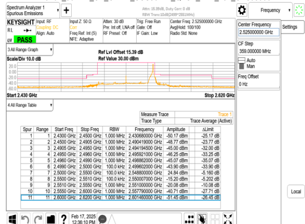
Band7_50MHz_CP_OFDM_SCS30kHz_QPSK_RB1_132_CH505000
