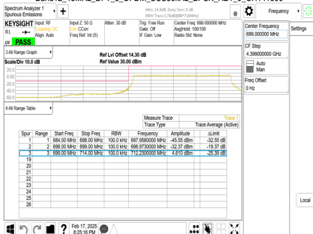
Band12_15MHz_DFT_s_OFDM_SCS30kHz_BPSK_RB36_0_CH141300
