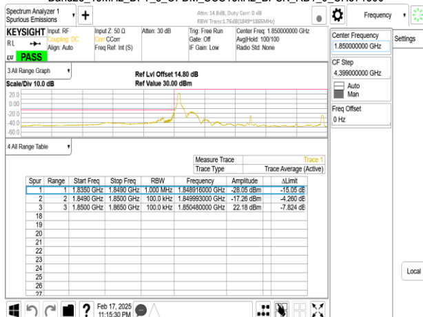
Band25_15MHz_DFT_s_OFDM_SCS15kHz_BPSK_RB75_0_CH371500
