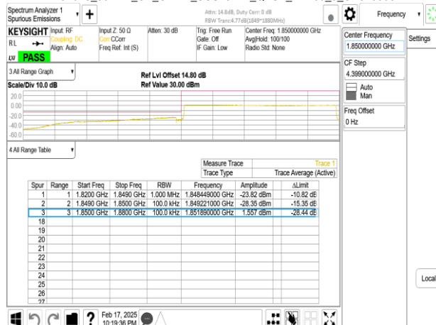
Band25_30MHz_CP_OFDM_SCS15kHz_QPSK_RB1_0_CH373000
