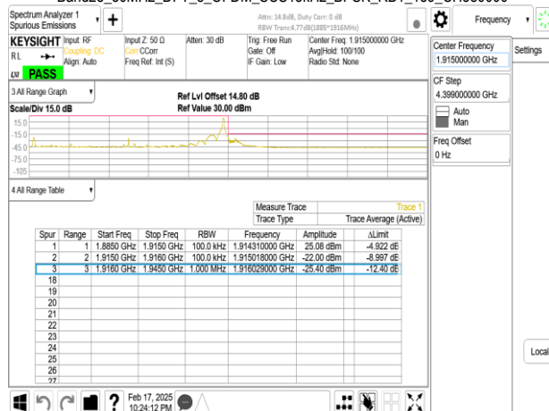
Band25_30MHz_CP_OFDM_SCS15kHz_QPSK_RB160_0_CH373000
