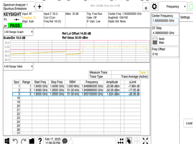
Band25_5MHz_CP_OFDM_SCS15kHz_QPSK_RB25_0_CH370500
