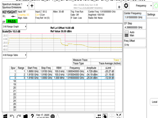
Band25_20MHz_DFT_s_OFDM_SCS15kHz_BPSK_RB1_105_CH381000
