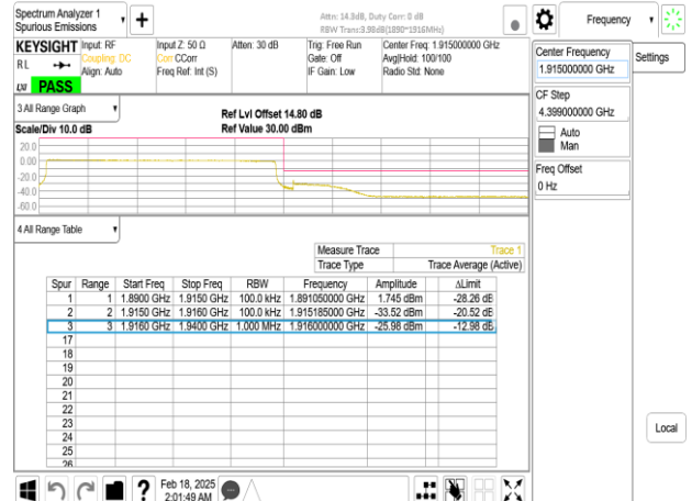
Band25_25MHz_CP_OFDM_SCS30kHz_QPSK_RB65_0_CH380500
