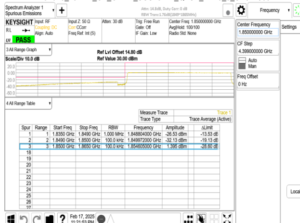
Band25_15MHz_CP_OFDM_SCS15kHz_QPSK_RB79_0_CH371500
