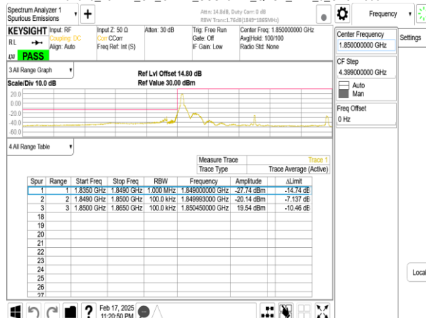
Band25_15MHz_CP_OFDM_SCS15kHz_QPSK_RB79_0_CH371500
