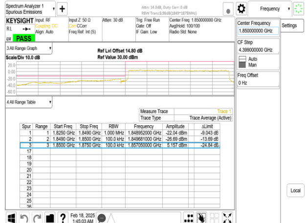
Band25_25MHz_DFT_s_OFDM_SCS30kHz_BPSK_RB64_0_CH372500
