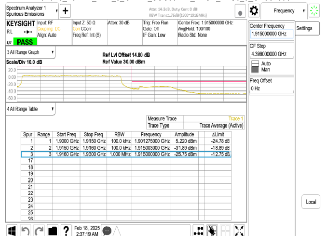
Band25_15MHz_DFT_s_OFDM_SCS30kHz_BPSK_RB36_0_CH381500
