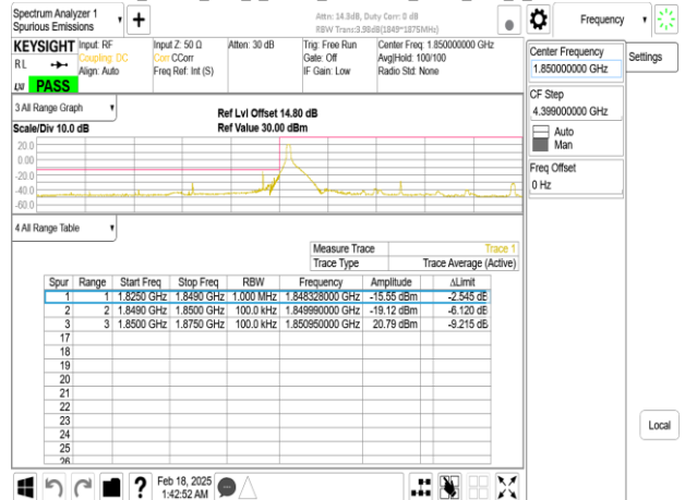
Band25_25MHz_DFT_s_OFDM_SCS30kHz_BPSK_RB64_0_CH372500
