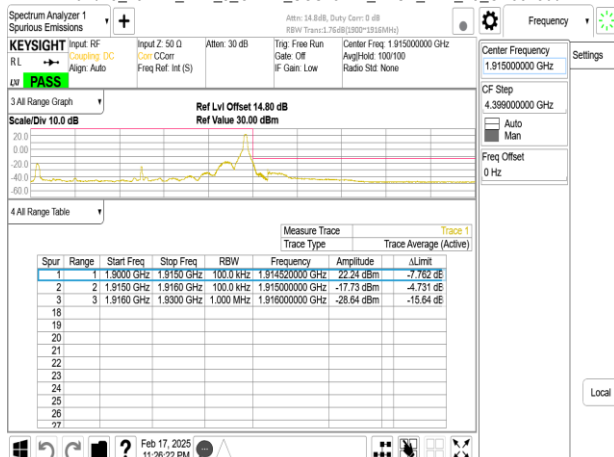
Band25_15MHz_DFT_s_OFDM_SCS15kHz_BPSK_RB1_78_CH381500
