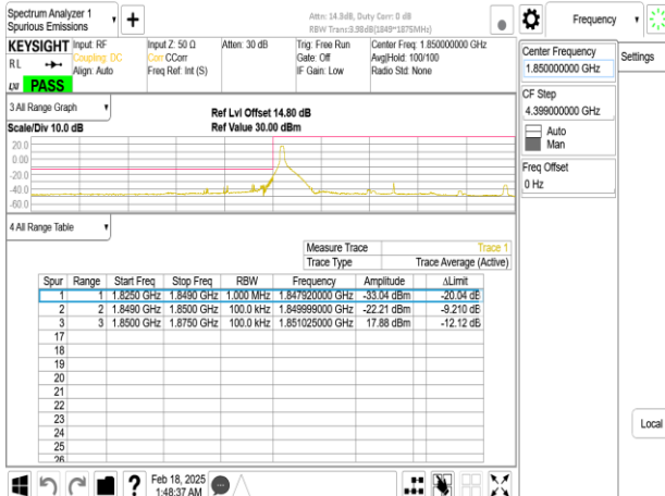
Band25_25MHz_CP_OFDM_SCS30kHz_QPSK_RB1_0_CH372500
