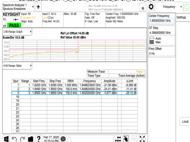
Band25_30MHz_DFT_s_OFDM_SCS15kHz_BPSK_RB1_0_CH373000
