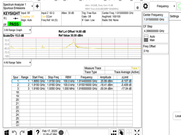
Band25_20MHz_CP_OFDM_SCS15kHz_QPSK_RB1_105_CH381000
