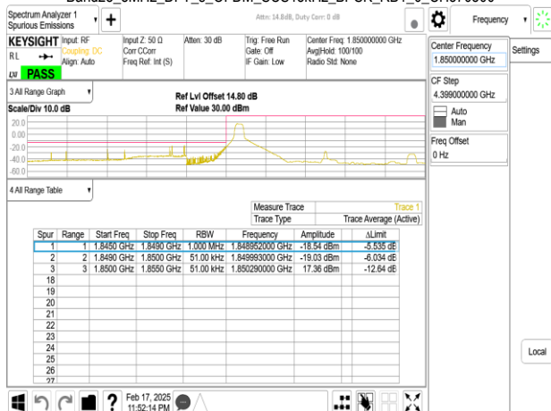
Band25_5MHz_DFT_s_OFDM_SCS15kHz_BPSK_RB25_0_CH370500
