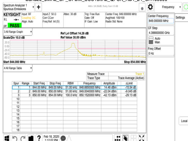
Band26_5MHz_CP_OFDM_SCS15kHz_QPSK_RB25_0_CH169300
