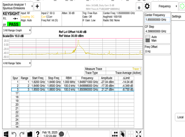
Band25_30MHz_DFT_s_OFDM_SCS30kHz_BPSK_RB1_0_CH373000
