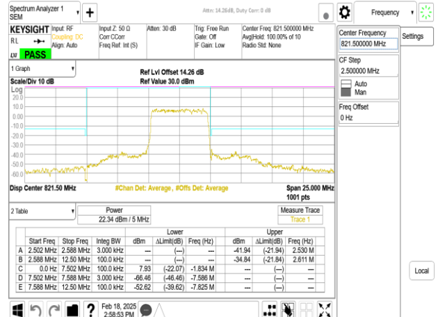
Band26-Part90s_5MHz_DFT_s_OFDM_SCS15kHz_BPSK_RB25_0_CH164300
