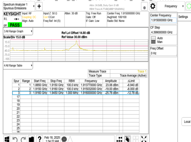
Band25_30MHz_DFT_s_OFDM_SCS30kHz_BPSK_RB75_0_CH380000
