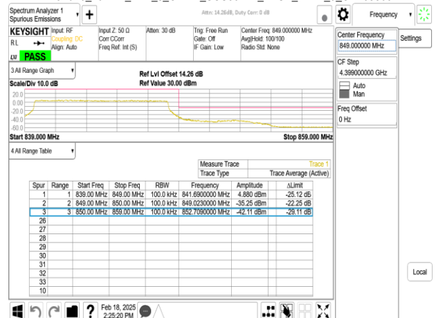
Band26_10MHz_DFT_s_OFDM_SCS30kHz_BPSK_RB24_0_CH168800
