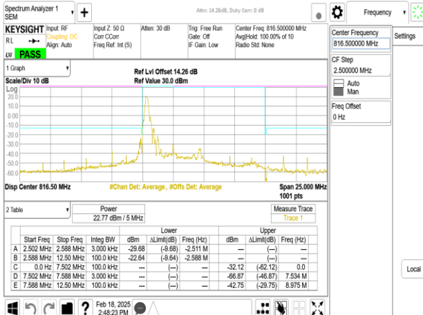
Band26-Part90s_5MHz_DFT_s_OFDM_SCS15kHz_BPSK_RB1_0_CH163300
