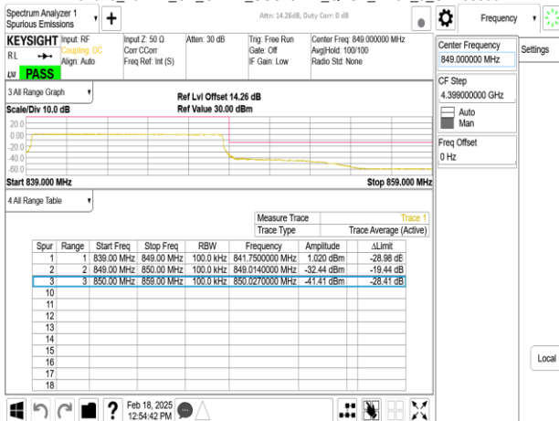
Band26_10MHz_DFT_s_OFDM_SCS30kHz_BPSK_RB1_0_CH168800
