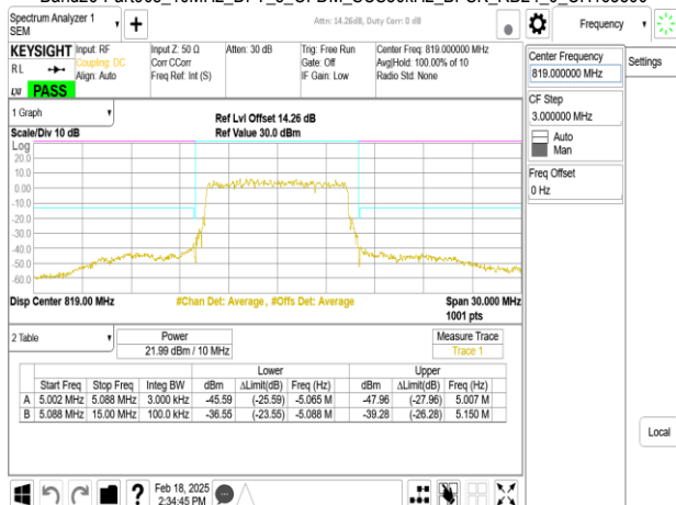
Band26-Part90s_10MHz_CP_OFDM_SCS30kHz_QPSK_RB1_0_CH163800
