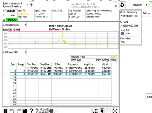
Band25_40MHz_CP_OFDM_SCS15kHz_QPSK_RB216_0_CH379000
