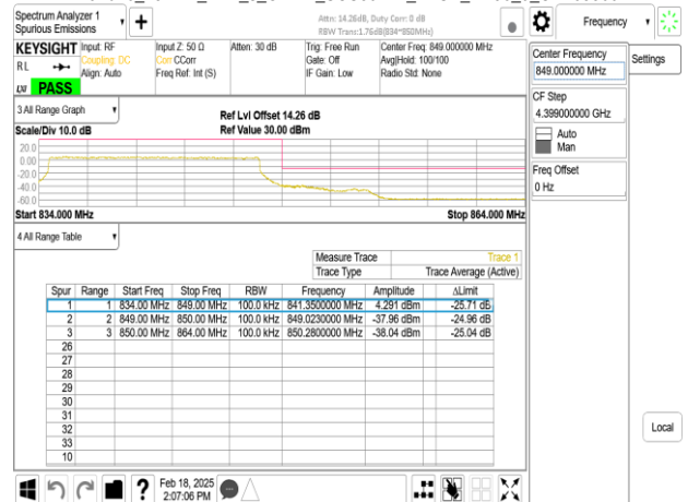
Band26_15MHz_CP_OFDM_SCS30kHz_QPSK_RB1_0_CH166300
