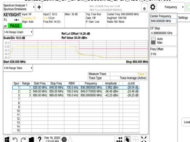
Band26_20MHz_CP_OFDM_SCS30kHz_QPSK_RB51_0_CH167800
