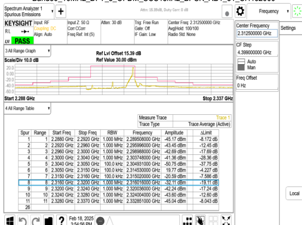
Band30_10MHz_DFT_s_OFDM_SCS15kHz_BPSK_RB1_51_CH462000
