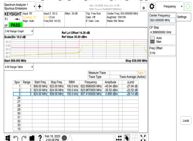
Band26_15MHz_CP_OFDM_SCS30kHz_QPSK_RB38_0_CH166300
