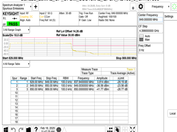
Band26_20MHz_CP_OFDM_SCS15kHz_QPSK_RB106_0_CH167800
