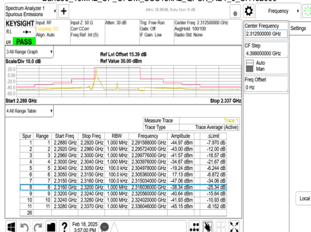
Band30_10MHz_CP_OFDM_SCS15kHz_QPSK_RB1_50_CH462000
