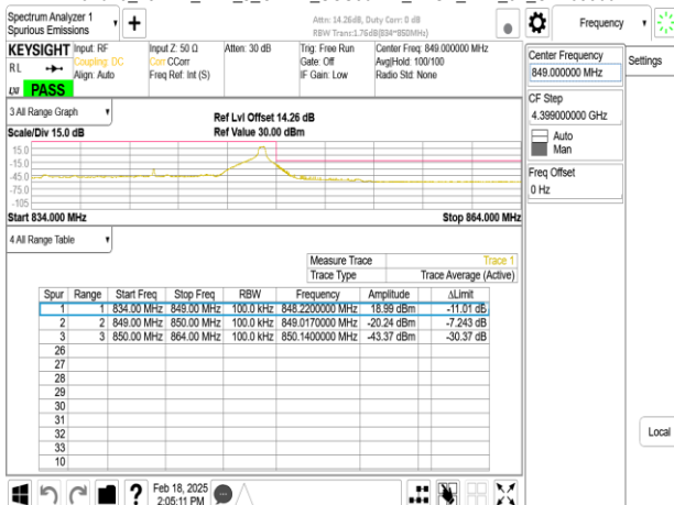
Band26_15MHz_DFT_s_OFDM_SCS30kHz_BPSK_RB1_37_CH168300
