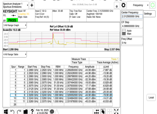
Band30_5MHz_DFT_s_OFDM_SCS15kHz_BPSK_RB25_0_CH462000
