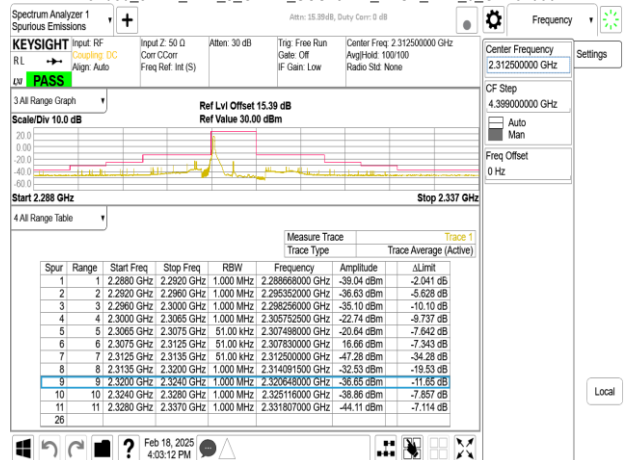
Band30_5MHz_DFT_s_OFDM_SCS15kHz_BPSK_RB1_24_CH462000
