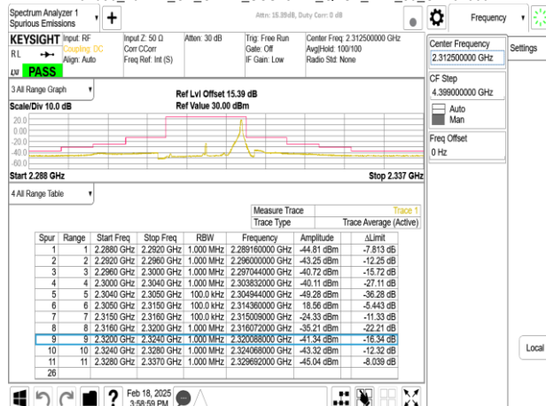
Band30_10MHz_CP_OFDM_SCS15kHz_QPSK_RB1_51_CH462000
