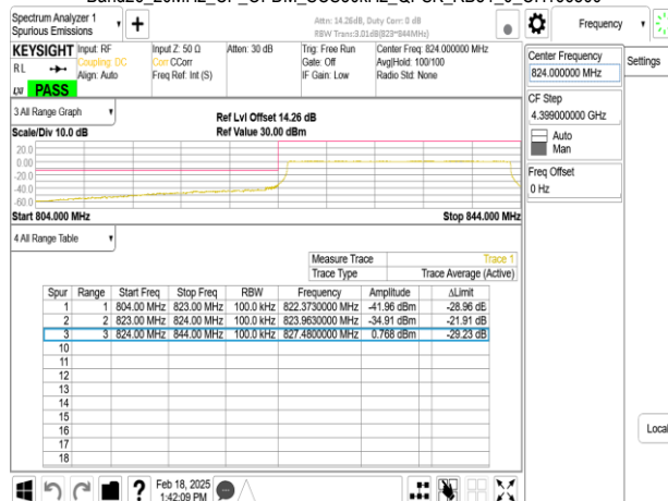
Band26_20MHz_CP_OFDM_SCS30kHz_QPSK_RB1_50_CH167800
