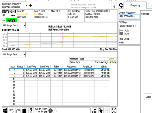
Band26_20MHz_CP_OFDM_SCS15kHz_QPSK_RB1_0_CH166800
