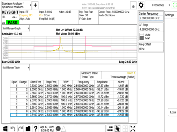
Band38_20MHz_DFT_s_OFDM_SCS15kHz_BPSK_RB1_105_CH516000
