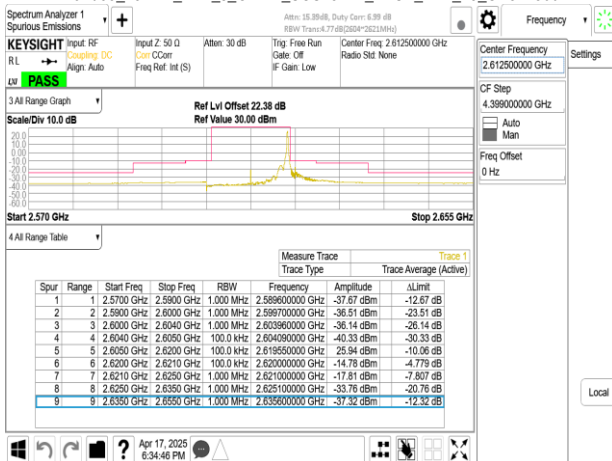
Band38_15MHz_DFT_s_OFDM_SCS15kHz_BPSK_RB75_0_CH522500
