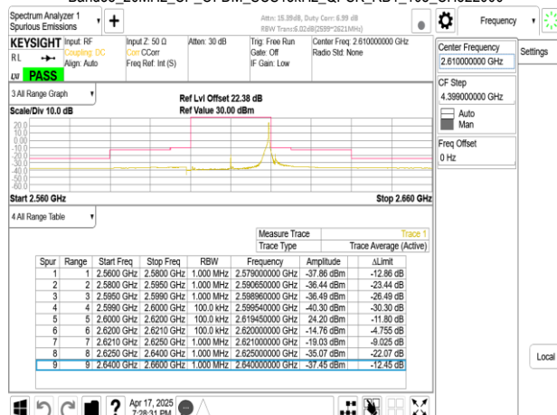
Band38_20MHz_CP_OFDM_SCS15kHz_QPSK_RB1_105_CH522000
