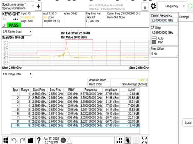
Band38_20MHz_DFT_s_OFDM_SCS30kHz_BPSK_RB1_50_CH522000
