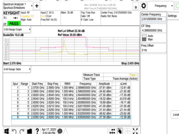
Band38_15MHz_CP_OFDM_SCS30kHz_QPSK_RB1_37_CH522500
