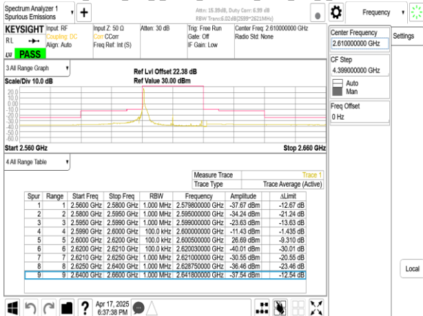
Band38_20MHz_DFT_s_OFDM_SCS15kHz_BPSK_RB1_105_CH522000
