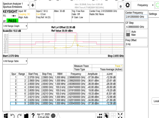
Band38_15MHz_CP_OFDM_SCS30kHz_QPSK_RB38_0_CH522500
