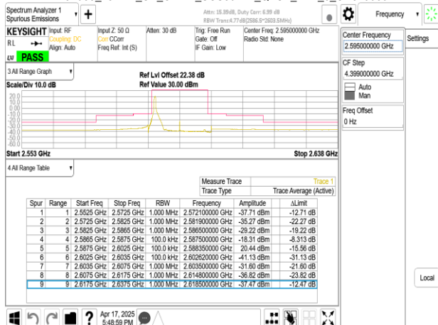
Band38_15MHz_CP_OFDM_SCS30kHz_QPSK_RB1_37_CH519000
