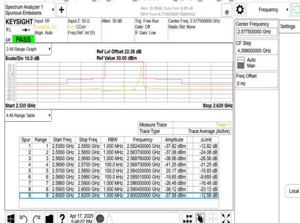
Band38_15MHz_CP_OFDM_SCS30kHz_QPSK_RB36_0_CH515500
