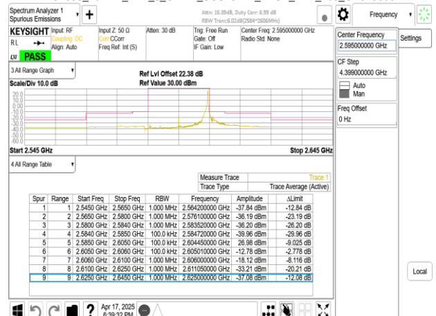
Band38_20MHz_DFT_s_OFDM_SCS15kHz_BPSK_RB1_105_CH519000
