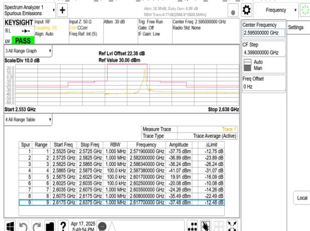
Band38_15MHz_CP_OFDM_SCS30kHz_QPSK_RB38_0_CH519000
