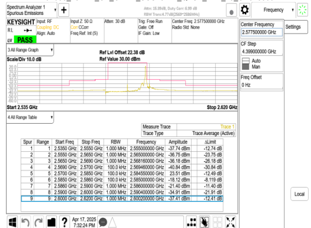
Band38_15MHz_CP_OFDM_SCS15kHz_QPSK_RB79_0_CH515500
