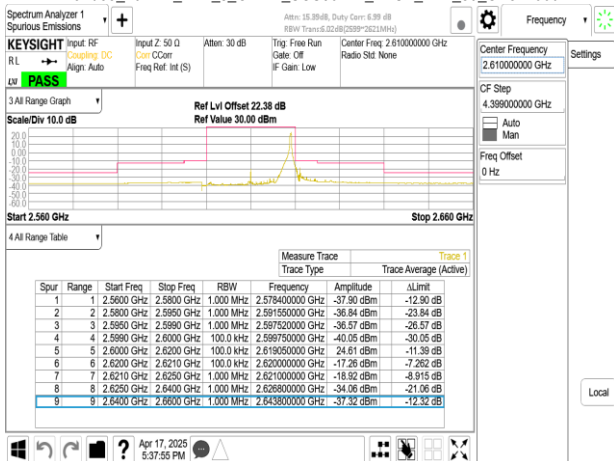
Band38_20MHz_DFT_s_OFDM_SCS30kHz_BPSK_RB50_0_CH522000
