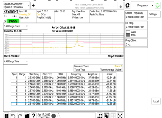
Band38_20MHz_CP_OFDM_SCS15kHz_QPSK_RB1_105_CH516000
