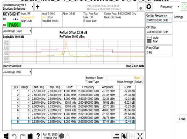
Band38_15MHz_DFT_s_OFDM_SCS30kHz_BPSK_RB1_37_CH522500
