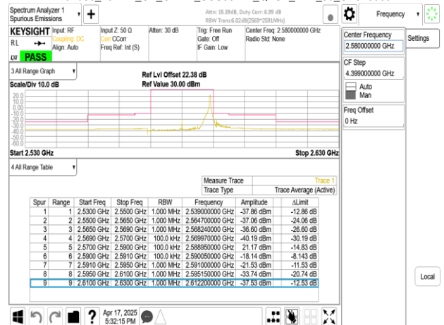
Band38_20MHz_CP_OFDM_SCS30kHz_QPSK_RB51_0_CH516000
