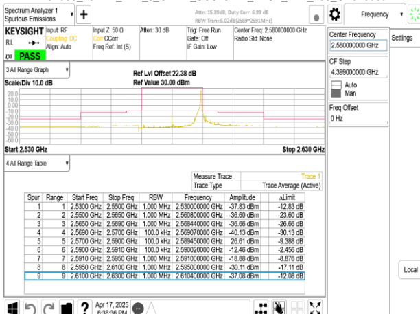
Band38_20MHz_DFT_s_OFDM_SCS15kHz_BPSK_RB1_105_CH516000
