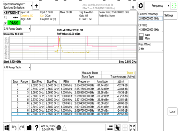
Band38_30MHz_CP_OFDM_SCS30kHz_QPSK_RB1_77_CH517000
