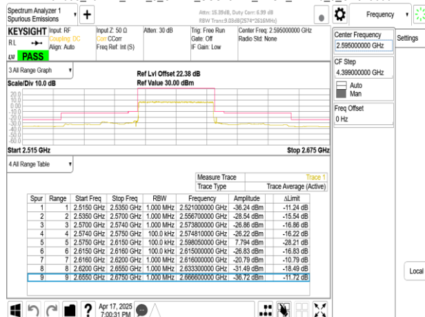
Band38_40MHz_DFT_s_OFDM_SCS15kHz_BPSK_RB216_0_CH519000
