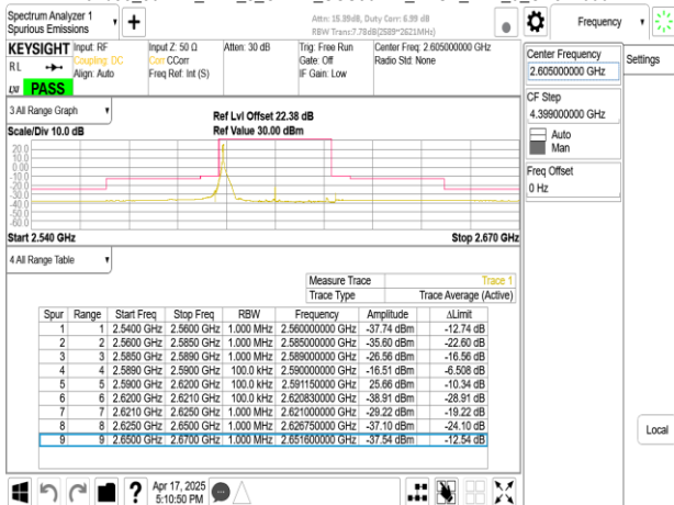
Band38_30MHz_DFT_s_OFDM_SCS30kHz_BPSK_RB1_77_CH521000
