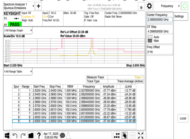
Band38_30MHz_CP_OFDM_SCS30kHz_QPSK_RB78_0_CH517000
