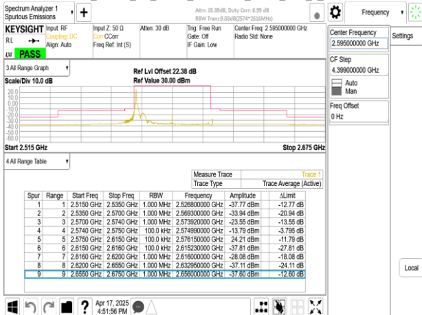
Band38_40MHz_CP_OFDM_SCS30kHz_QPSK_RB1_105_CH519000
