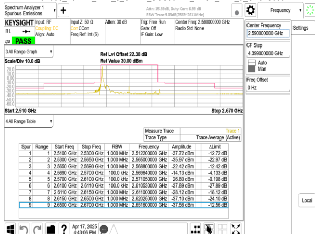
Band38_40MHz_DFT_s_OFDM_SCS30kHz_BPSK_RB1_105_CH518000
