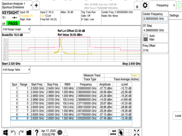
Band38_30MHz_DFT_s_OFDM_SCS30kHz_BPSK_RB1_77_CH517000
