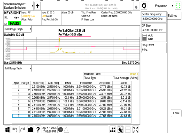
Band38_40MHz_CP_OFDM_SCS15kHz_QPSK_RB1_215_CH518000
