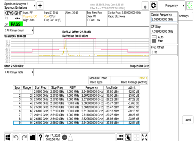
Band38_30MHz_DFT_s_OFDM_SCS30kHz_BPSK_RB1_77_CH519000
