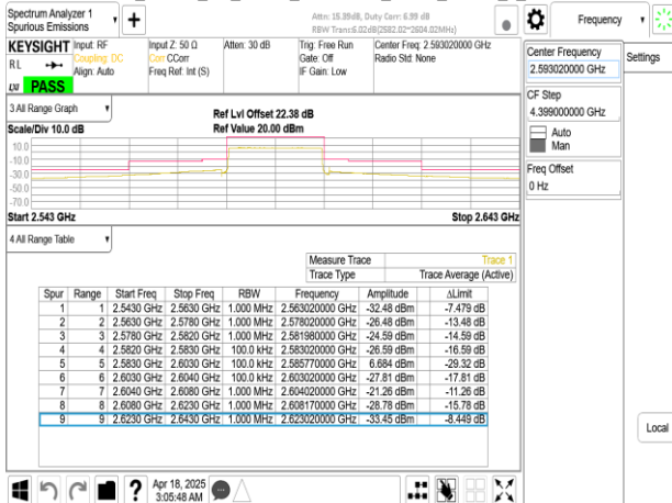
Band41_20MHz_CP_OFDM_SCS15kHz_QPSK_RB1_0_CH518604
