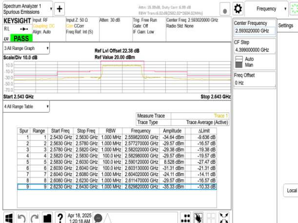
Band41_20MHz_DFT_s_OFDM_SCS30kHz_BPSK_RB50_0_CH518604
