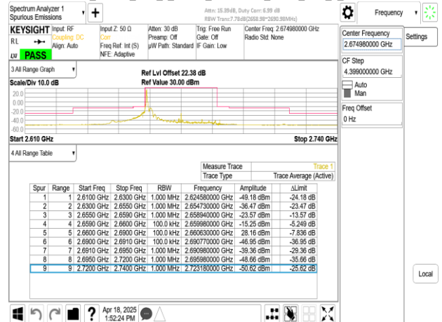
Band41_30MHz_DFT_s_OFDM_SCS15kHz_BPSK_RB1_159_CH534996
