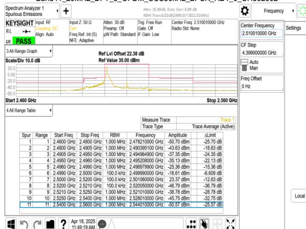
Band41_20MHz_DFT_s_OFDM_SCS30kHz_BPSK_RB1_50_CH502002
