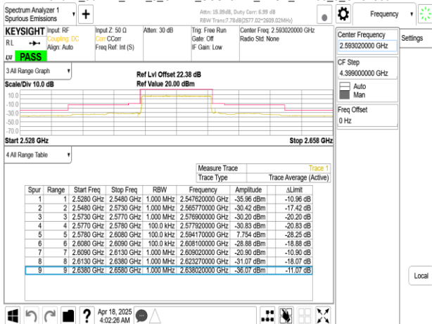
Band41_30MHz_DFT_s_OFDM_SCS15kHz_BPSK_RB1_0_CH518604
