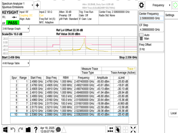
Band41_20MHz_CP_OFDM_SCS30kHz_QPSK_RB51_0_CH501204
