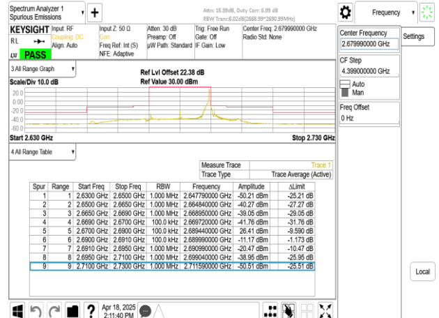
Band41_20MHz_CP_OFDM_SCS15kHz_QPSK_RB1_105_CH535998
