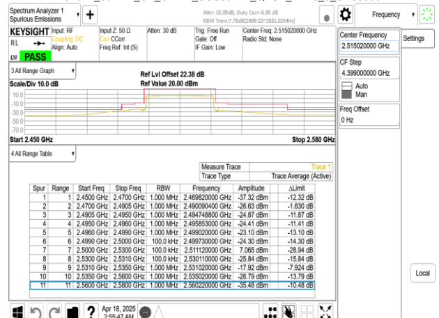
Band41_30MHz_CP_OFDM_SCS30kHz_QPSK_RB78_0_CH503004
