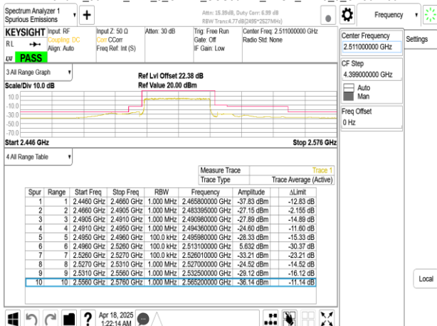
Band41_30MHz_DFT_s_OFDM_SCS30kHz_BPSK_RB75_0_CH502200
