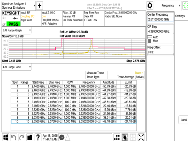
Band41_30MHz_CP_OFDM_SCS30kHz_QPSK_RB78_0_CH502200
