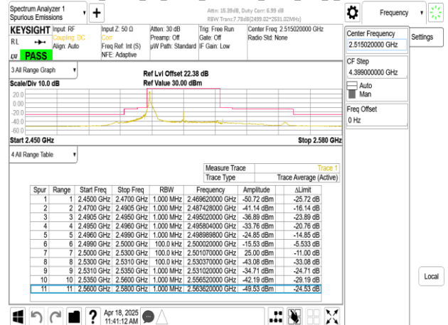
Band41_30MHz_CP_OFDM_SCS30kHz_QPSK_RB1_77_CH503004
