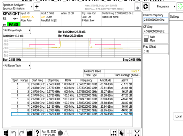
Band41_30MHz_CP_OFDM_SCS15kHz_QPSK_RB1_0_CH518604
