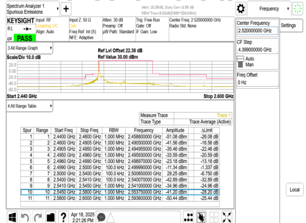
Band41_40MHz_CP_OFDM_SCS15kHz_QPSK_RB1_215_CH504000
