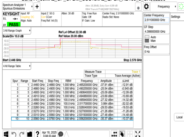
Band41_30MHz_CP_OFDM_SCS15kHz_QPSK_RB1_0_CH502200
