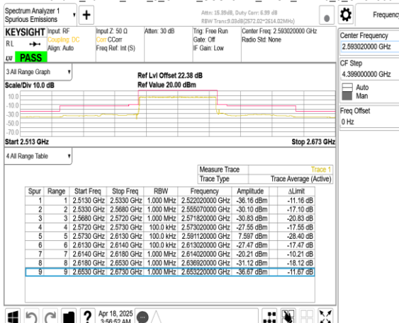
Band41_40MHz_DFT_s_OFDM_SCS15kHz_BPSK_RB216_0_CH518604
