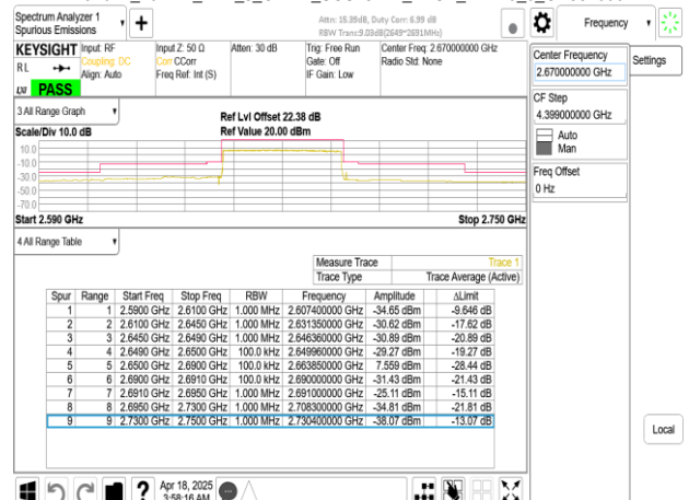
Band41_40MHz_DFT_s_OFDM_SCS15kHz_BPSK_RB216_0_CH534000
