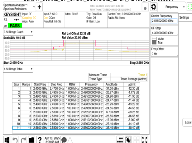
Band41_30MHz_CP_OFDM_SCS15kHz_QPSK_RB1_0_CH503004
