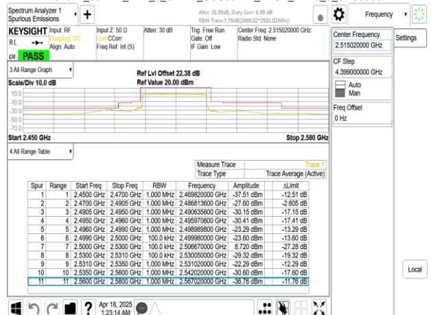
Band41_30MHz_DFT_s_OFDM_SCS30kHz_BPSK_RB75_0_CH503004
