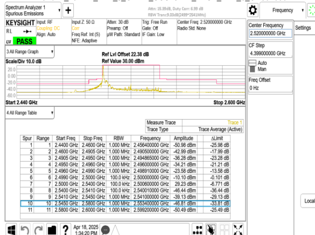
Band41_40MHz_DFT_s_OFDM_SCS15kHz_BPSK_RB1_215_CH504000
