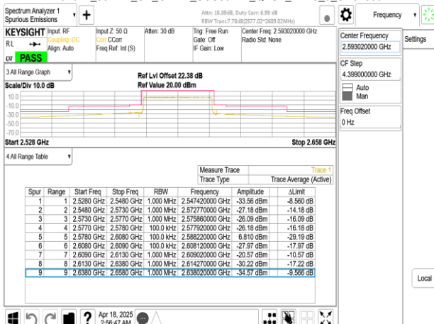
Band41_30MHz_CP_OFDM_SCS30kHz_QPSK_RB78_0_CH518604
