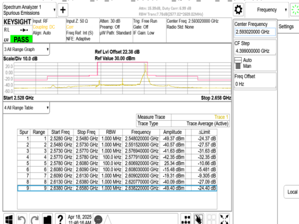
Band41_30MHz_CP_OFDM_SCS30kHz_QPSK_RB78_0_CH518604
