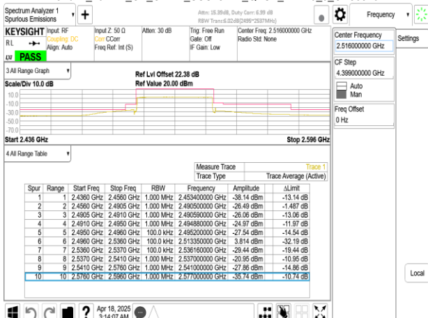
Band41_40MHz_CP_OFDM_SCS15kHz_QPSK_RB216_0_CH503202
