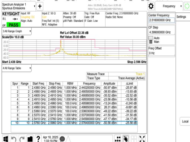
Band41_40MHz_DFT_s_OFDM_SCS15kHz_BPSK_RB1_215_CH503202
