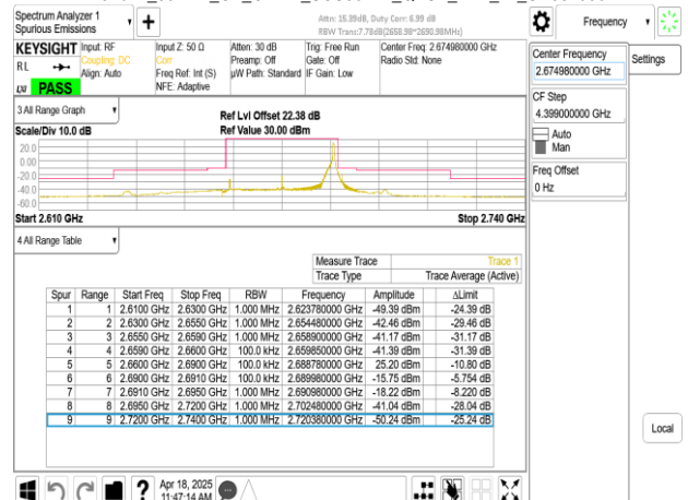
Band41_30MHz_CP_OFDM_SCS30kHz_QPSK_RB78_0_CH534996
