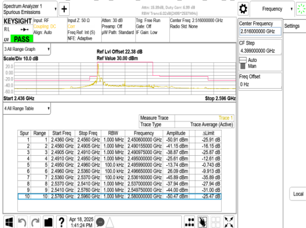
Band41_40MHz_CP_OFDM_SCS15kHz_QPSK_RB1_215_CH503202
