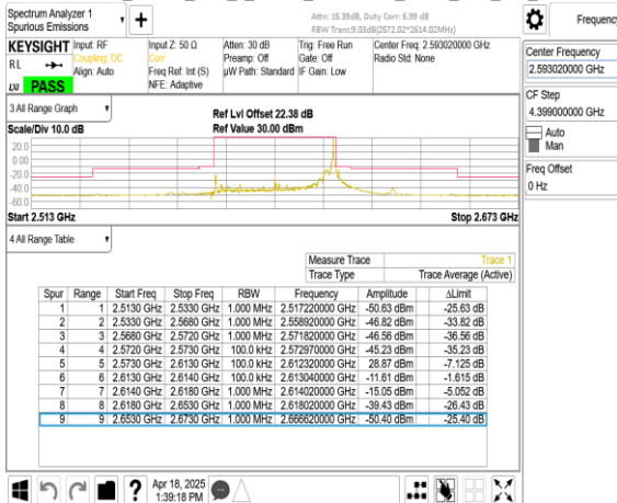
Band41_40MHz_DFT_s_OFDM_SCS15kHz_BPSK_RB216_0_CH518604
