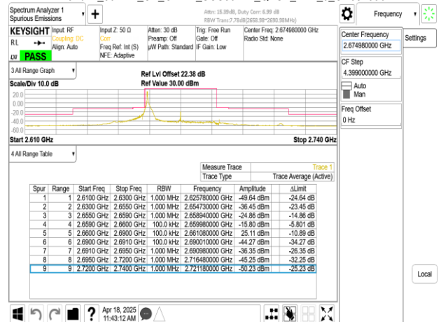
Band41_30MHz_CP_OFDM_SCS30kHz_QPSK_RB1_77_CH534996
