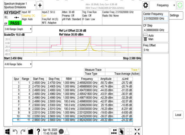
Band41_30MHz_CP_OFDM_SCS30kHz_QPSK_RB78_0_CH503004
