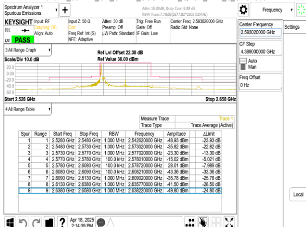
Band41_30MHz_CP_OFDM_SCS15kHz_QPSK_RB1_159_CH518604
