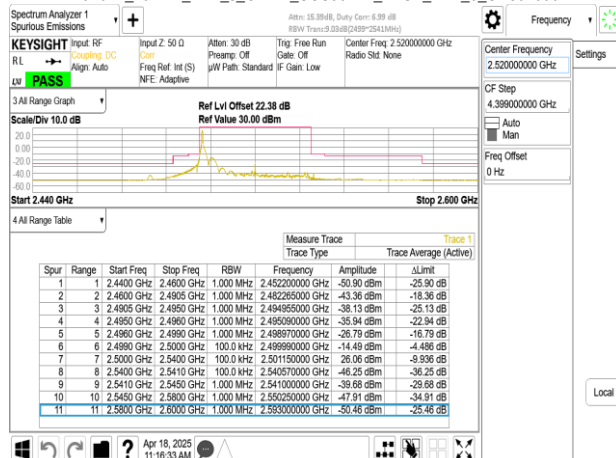
Band41_40MHz_DFT_s_OFDM_SCS30kHz_BPSK_RB1_105_CH504000
