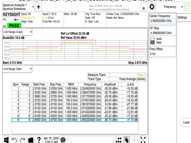
Band41_40MHz_DFT_s_OFDM_SCS30kHz_BPSK_RB1_0_CH518604
