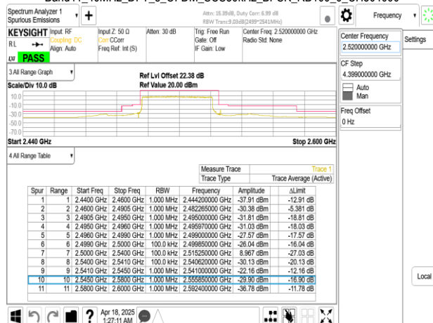
Band41_40MHz_DFT_s_OFDM_SCS30kHz_BPSK_RB1_0_CH504000
