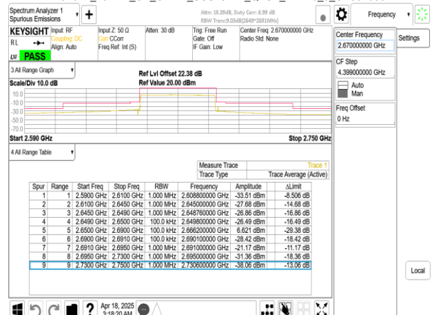
Band41_40MHz_CP_OFDM_SCS15kHz_QPSK_RB216_0_CH534000
