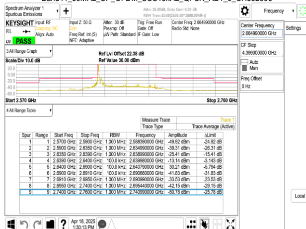
Band41_50MHz_CP_OFDM_SCS15kHz_QPSK_RB1_269_CH532998
