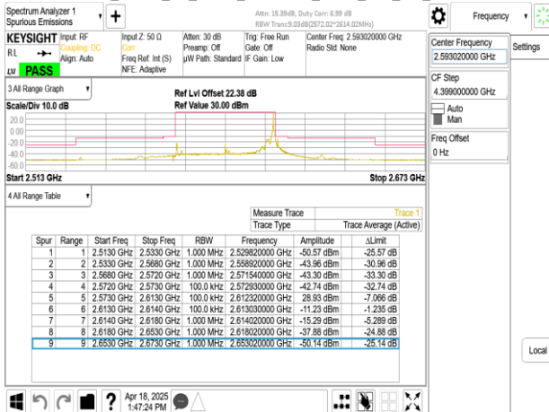
Band41_40MHz_CP_OFDM_SCS15kHz_QPSK_RB216_0_CH518604
