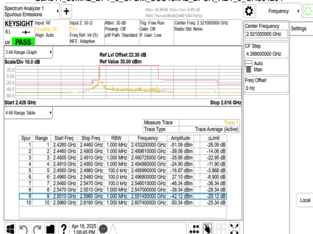
Band41_50MHz_DFT_s_OFDM_SCS15kHz_BPSK_RB1_269_CH504204
