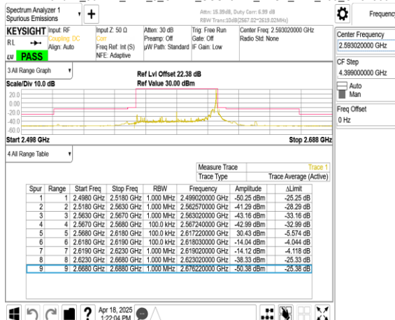
Band41_50MHz_DFT_s_OFDM_SCS15kHz_BPSK_RB270_0_CH518604
