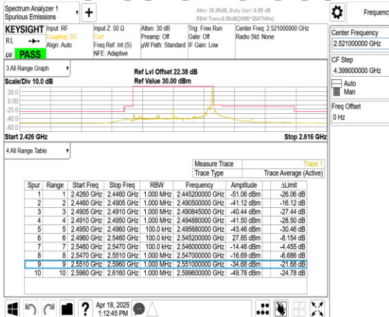
Band41_50MHz_CP_OFDM_SCS15kHz_QPSK_RB270_0_CH504204
