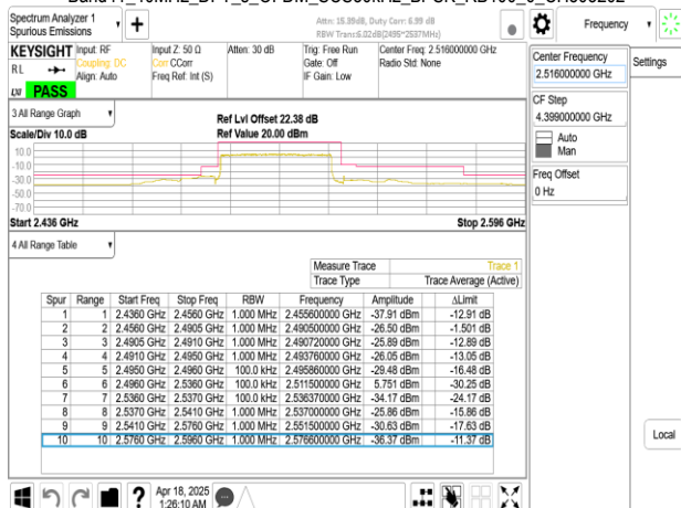
Band41_40MHz_DFT_s_OFDM_SCS30kHz_BPSK_RB1_0_CH503202
