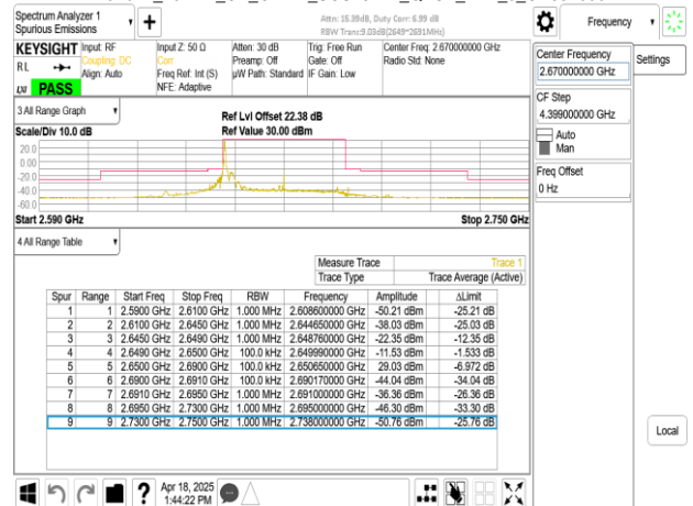
Band41_40MHz_CP_OFDM_SCS15kHz_QPSK_RB1_215_CH534000
