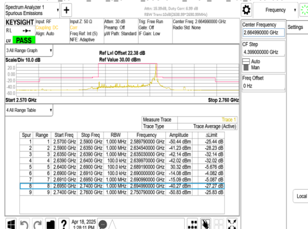
Band41_50MHz_DFT_s_OFDM_SCS15kHz_BPSK_RB270_0_CH532998
