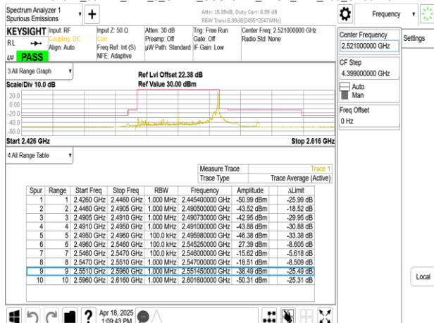
Band41_50MHz_DFT_s_OFDM_SCS15kHz_BPSK_RB270_0_CH504204
