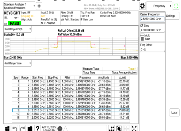
Band41_50MHz_CP_OFDM_SCS15kHz_QPSK_RB270_0_CH505002
