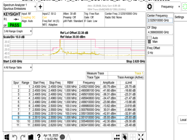
Band41_50MHz_DFT_s_OFDM_SCS15kHz_BPSK_RB1_269_CH505002
