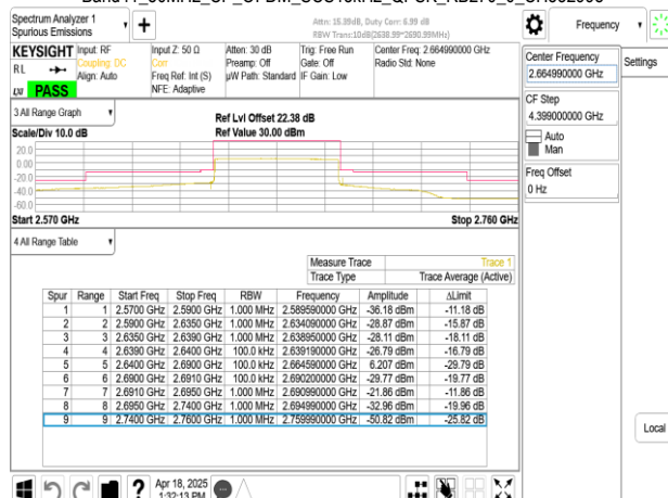
Band41_50MHz_CP_OFDM_SCS15kHz_QPSK_RB270_0_CH532998
