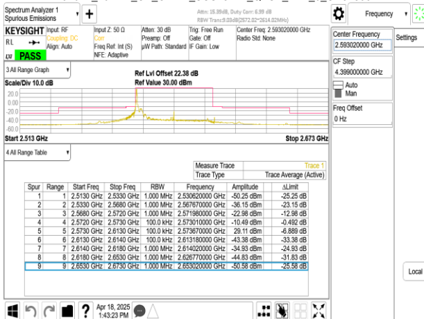
Band41_40MHz_CP_OFDM_SCS15kHz_QPSK_RB1_215_CH518604
