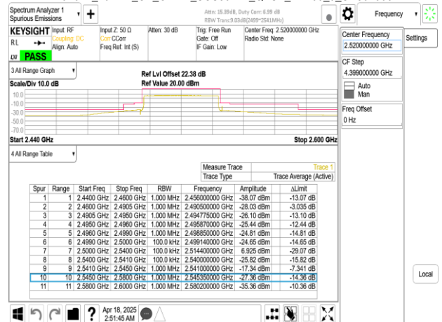
Band41_40MHz_CP_OFDM_SCS30kHz_QPSK_RB1_0_CH504000
