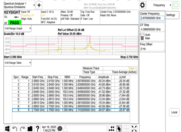
Band41_40MHz_CP_OFDM_SCS15kHz_QPSK_RB216_0_CH534000
