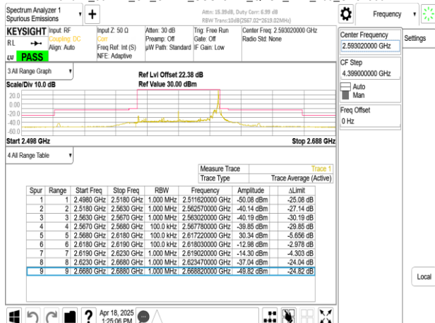
Band41_50MHz_CP_OFDM_SCS15kHz_QPSK_RB270_0_CH518604
