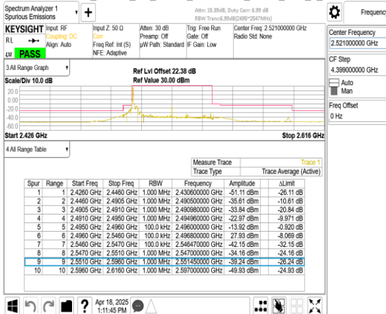
Band41_50MHz_CP_OFDM_SCS15kHz_QPSK_RB1_269_CH504204
