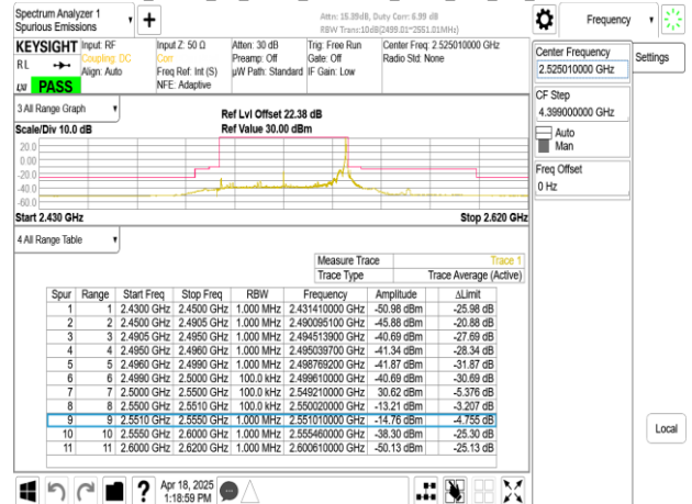
Band41_50MHz_CP_OFDM_SCS15kHz_QPSK_RB270_0_CH505002
