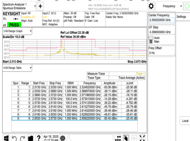
Band41_40MHz_DFT_s_OFDM_SCS30kHz_BPSK_RB1_105_CH518604
