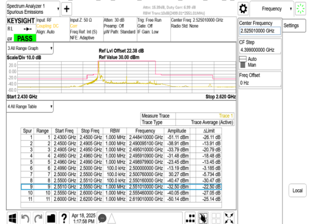
Band41_50MHz_CP_OFDM_SCS15kHz_QPSK_RB1_269_CH505002
