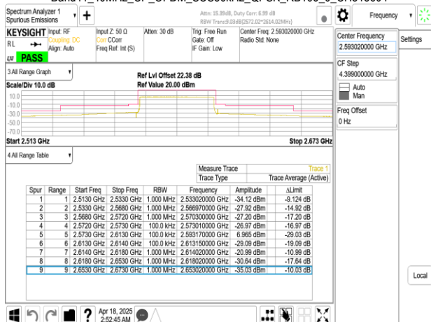
Band41_40MHz_CP_OFDM_SCS30kHz_QPSK_RB1_0_CH518604
