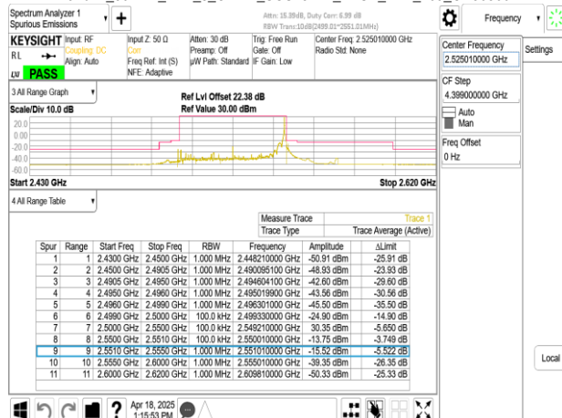
Band41_50MHz_DFT_s_OFDM_SCS15kHz_BPSK_RB270_0_CH505002
