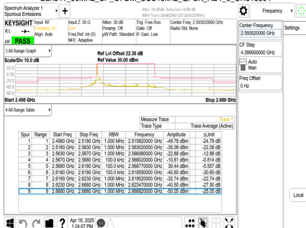
Band41_50MHz_CP_OFDM_SCS15kHz_QPSK_RB1_269_CH518604
