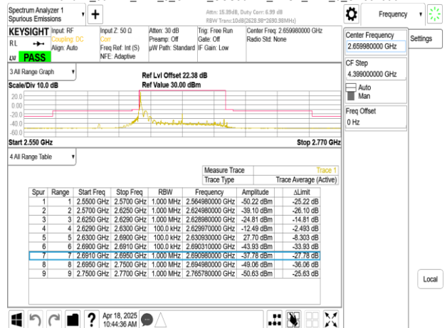
Band41_60MHz_DFT_s_OFDM_SCS30kHz_BPSK_RB1_161_CH531996
