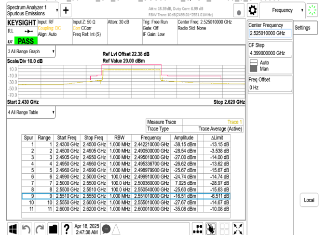
Band41_50MHz_CP_OFDM_SCS30kHz_QPSK_RB1_0_CH505002
