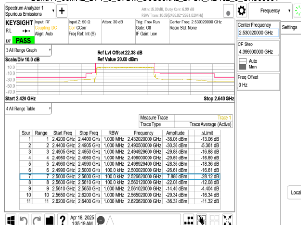
Band41_60MHz_DFT_s_OFDM_SCS30kHz_BPSK_RB1_0_CH506004
