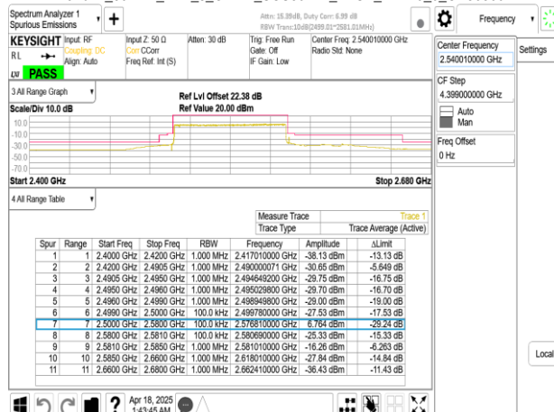
Band41_80MHz_DFT_s_OFDM_SCS30kHz_BPSK_RB216_0_CH508002
