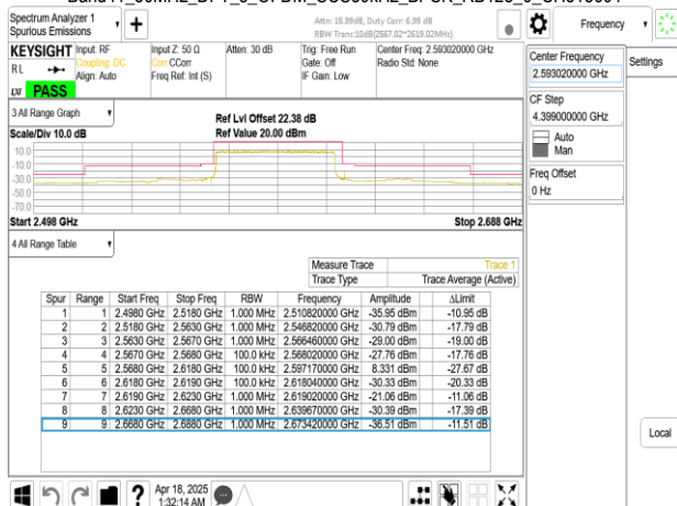
Band41_50MHz_DFT_s_OFDM_SCS30kHz_BPSK_RB1_0_CH518604
