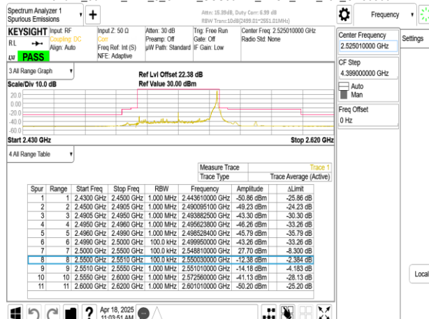
Band41_50MHz_DFT_s_OFDM_SCS30kHz_BPSK_RB1_132_CH505002
