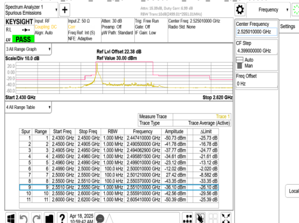
Band41_50MHz_DFT_s_OFDM_SCS30kHz_BPSK_RB1_132_CH505002
