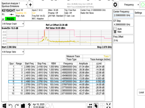
Band41_80MHz_DFT_s_OFDM_SCS30kHz_BPSK_RB1_216_CH507204
