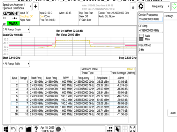
Band41_60MHz_DFT_s_OFDM_SCS30kHz_BPSK_RB1_0_CH505200
