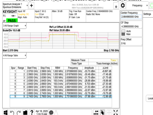
Band41_50MHz_DFT_s_OFDM_SCS30kHz_BPSK_RB1_0_CH532998
