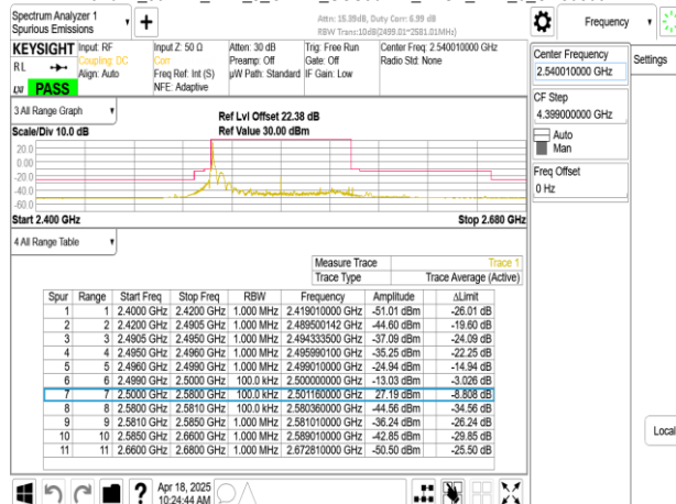
Band41_80MHz_DFT_s_OFDM_SCS30kHz_BPSK_RB1_216_CH508002
