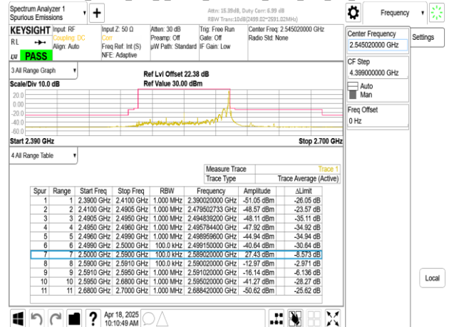
Band41_90MHz_DFT_s_OFDM_SCS30kHz_BPSK_RB243_0_CH509004
