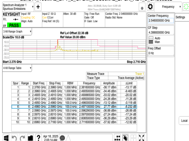
Band41_100MHz_DFT_s_OFDM_SCS30kHz_BPSK_RB1_272_CH509202
