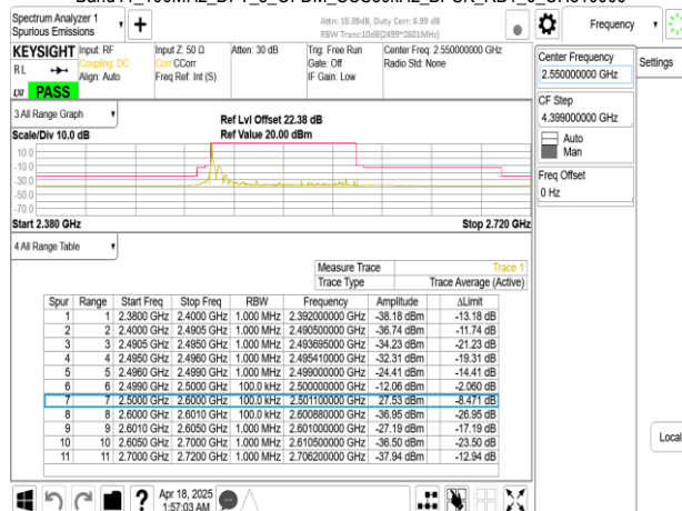
Band41_100MHz_DFT_s_OFDM_SCS30kHz_BPSK_RB1_272_CH510000
