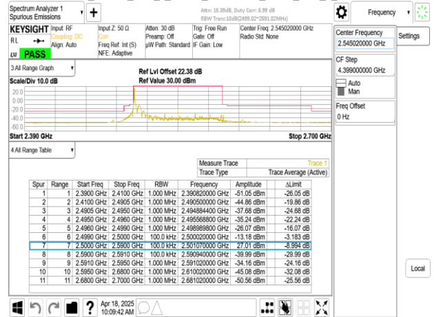
Band41_90MHz_DFT_s_OFDM_SCS30kHz_BPSK_RB1_244_CH509004
