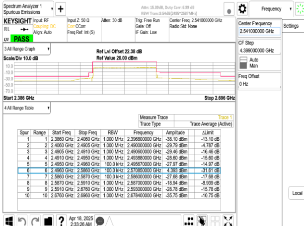
Band41_90MHz_CP_OFDM_SCS30kHz_QPSK_RB245_0_CH508200
