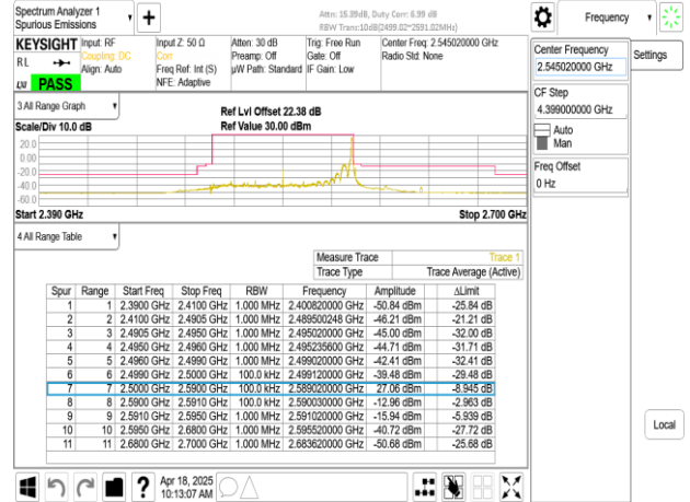
Band41_90MHz_CP_OFDM_SCS30kHz_QPSK_RB245_0_CH509004
