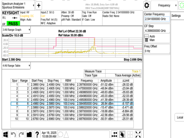
Band41_90MHz_DFT_s_OFDM_SCS30kHz_BPSK_RB243_0_CH508200
