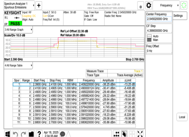
Band41_90MHz_CP_OFDM_SCS30kHz_QPSK_RB245_0_CH509004
