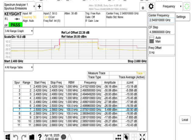
Band41_80MHz_CP_OFDM_SCS30kHz_QPSK_RB217_0_CH508002
