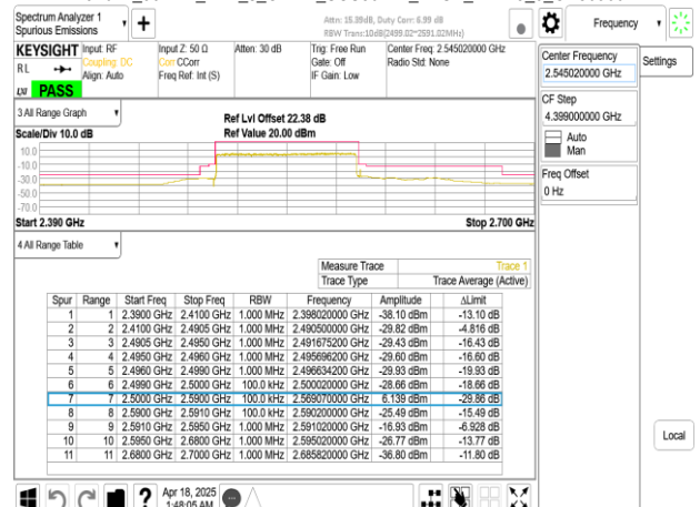
Band41_90MHz_DFT_s_OFDM_SCS30kHz_BPSK_RB243_0_CH509004
