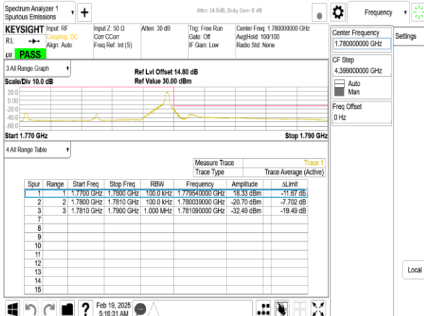
Band66_10MHz_CP_OFDM_SCS15kHz_QPSK_RB1_51_CH355000
