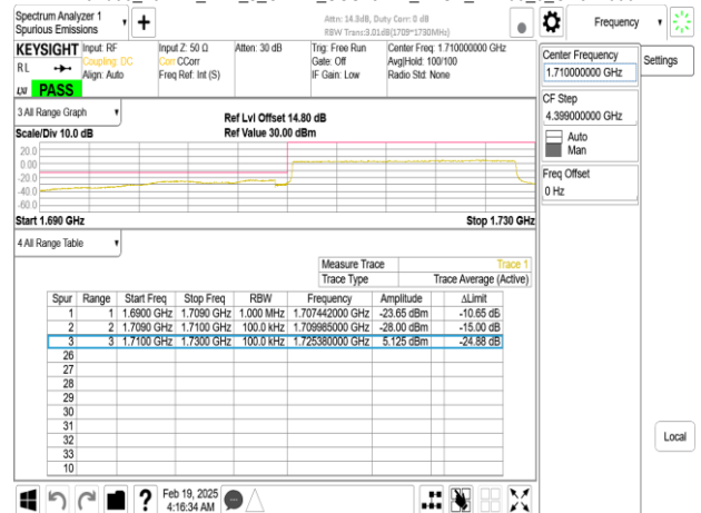
Band66_20MHz_DFT_s_OFDM_SCS15kHz_BPSK_RB1_0_CH344000
