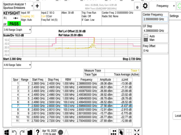
Band41_100MHz_CP_OFDM_SCS30kHz_QPSK_RB273_0_CH510000
