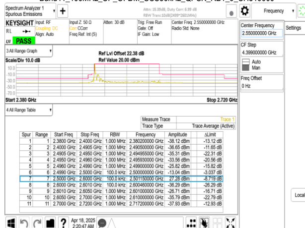
Band41_100MHz_CP_OFDM_SCS30kHz_QPSK_RB1_272_CH510000
