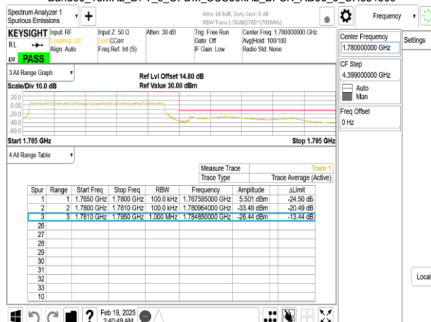
Band66_15MHz_DFT_s_OFDM_SCS30kHz_BPSK_RB36_0_CH354500
