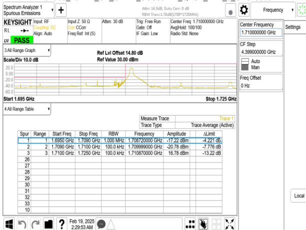
Band66_15MHz_CP_OFDM_SCS30kHz_QPSK_RB38_0_CH343500
