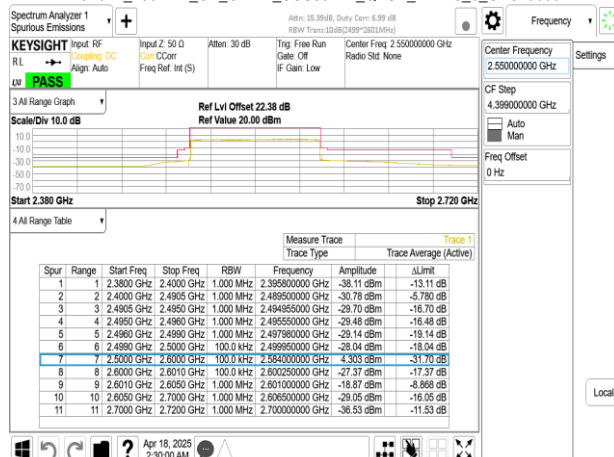
Band41_100MHz_CP_OFDM_SCS30kHz_QPSK_RB273_0_CH510000
