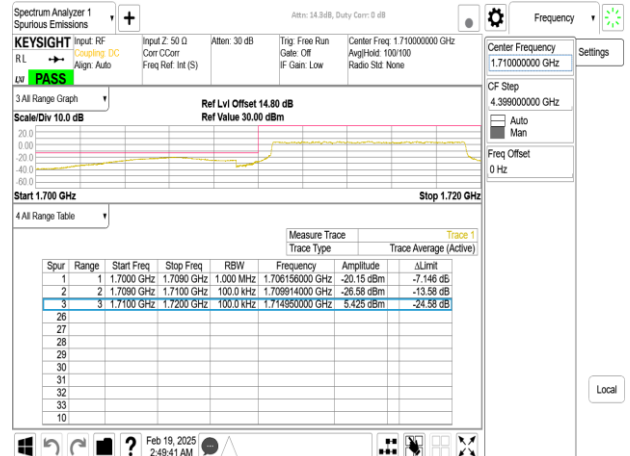
Band66_10MHz_DFT_s_OFDM_SCS30kHz_BPSK_RB24_0_CH343000
