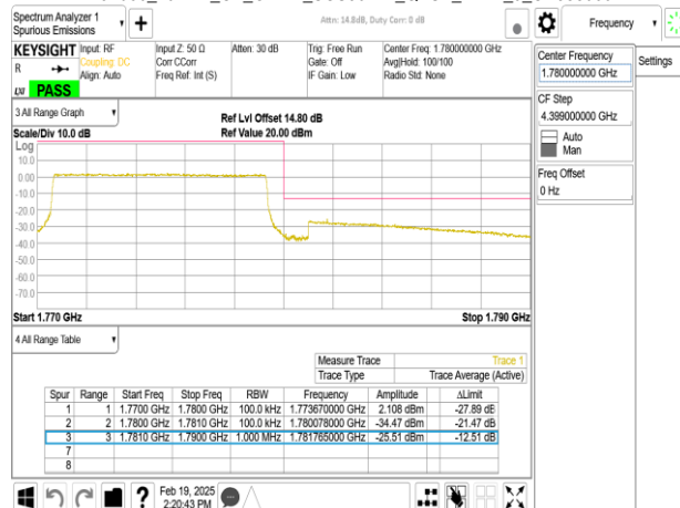
Band66_10MHz_CP_OFDM_SCS30kHz_QPSK_RB24_0_CH355000
