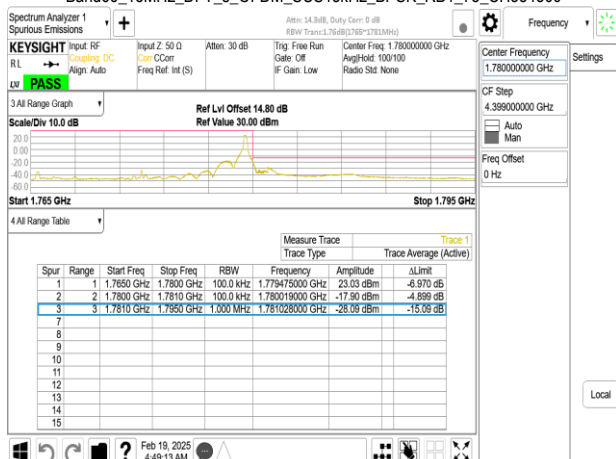
Band66_15MHz_DFT_s_OFDM_SCS15kHz_BPSK_RB1_78_CH34500
