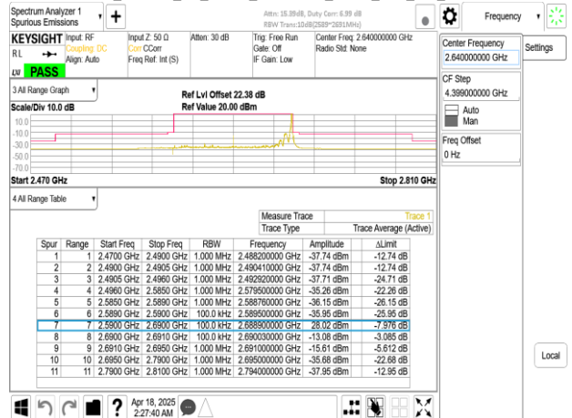
Band41_100MHz_CP_OFDM_SCS30kHz_QPSK_RB273_0_CH528000
