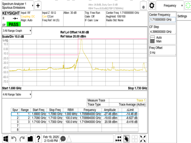
Band66_20MHz_DFT_s_OFDM_SCS30kHz_BPSK_RB50_0_CH344000
