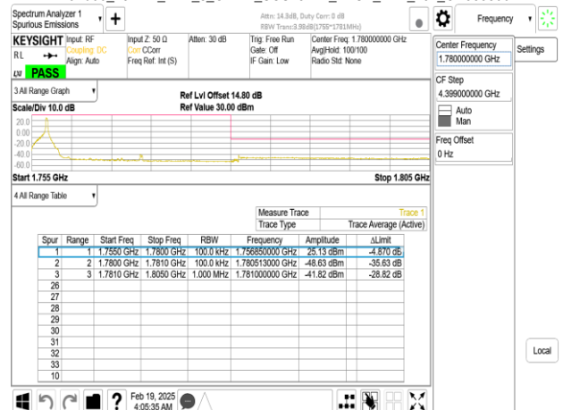
Band66_25MHz_DFT_s_OFDM_SCS15kHz_BPSK_RB1_132_CH353500
