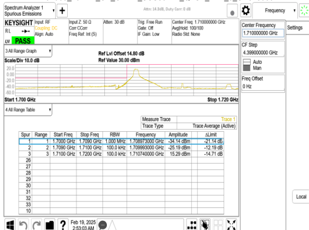
Band66_10MHz_CP_OFDM_SCS30kHz_QPSK_RB1_0_CH343000
