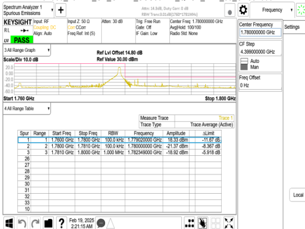
Band66_20MHz_CP_OFDM_SCS30kHz_QPSK_RB1_0_CH354000
