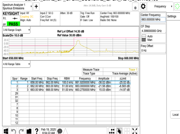
Band71_5MHz_CP_OFDM_SCS15kHz_QPSK_RB25_0_CH133100
