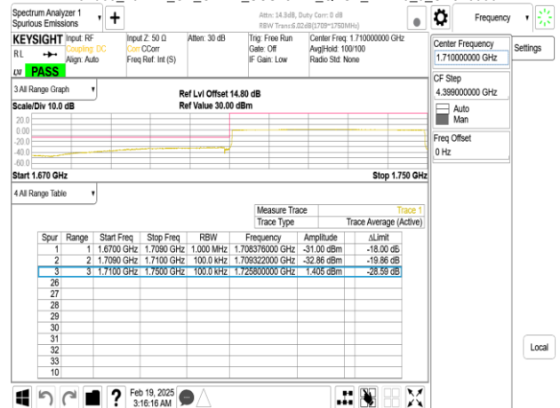
Band66_40MHz_CP_OFDM_SCS15kHz_QPSK_RB1_215_CH352000
