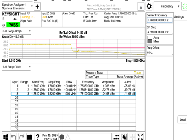
Band66_40MHz_DFT_s_OFDM_SCS30kHz_BPSK_RB100_0_CH352000
