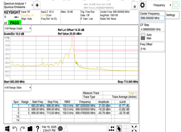
Band71_15MHz_DFT_s_OFDM_SCS15kHz_BPSK_RB75_0_CH138100
