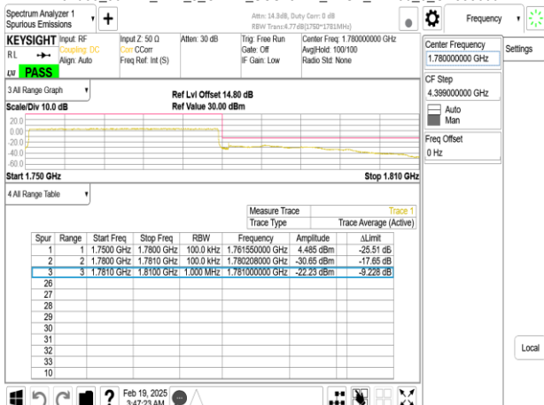
Band66_30MHz_DFT_s_OFDM_SCS15kHz_BPSK_RB160_0_CH353000
