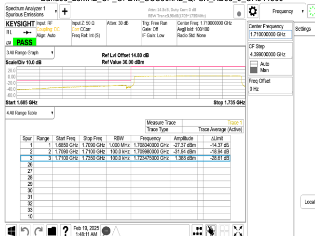
Band66_25MHz_CP_OFDM_SCS30kHz_QPSK_RB1_64_CH353500
