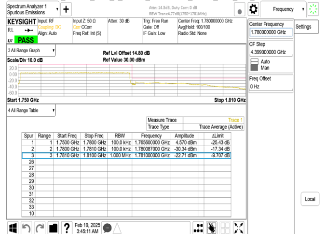
Band66_30MHz_CP_OFDM_SCS15kHz_QPSK_RB160_0_CH35000
