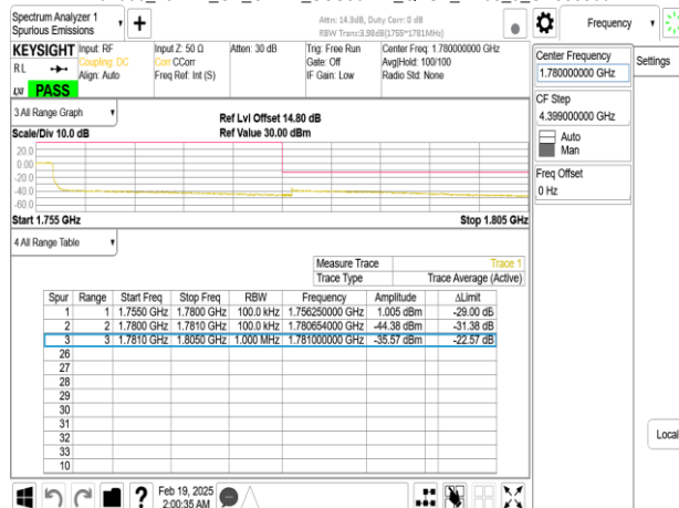
Band66_25MHz_CP_OFDM_SCS30kHz_QPSK_RB65_0_CH353500
