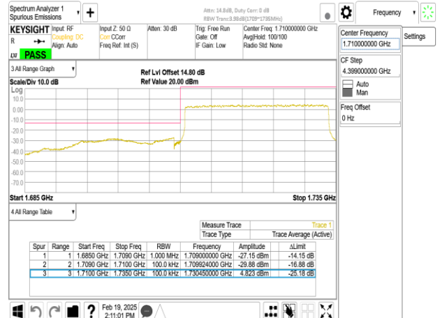
Band66_25MHz_DFT_s_OFDM_SCS30kHz_BPSK_RB64_0_CH344500
