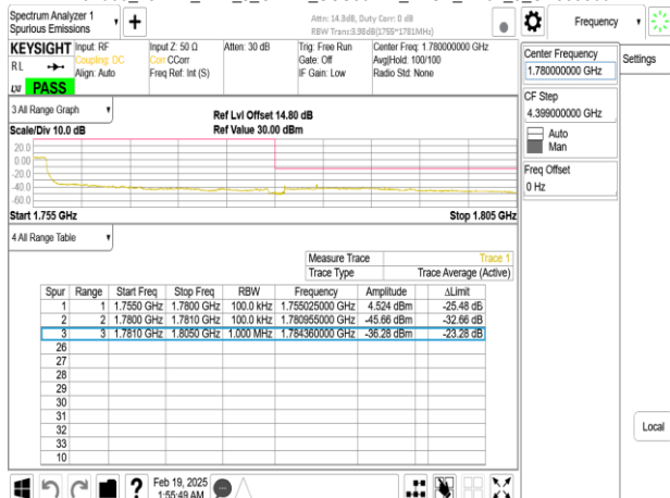
Band66_25MHz_CP_OFDM_SCS30kHz_QPSK_RB1_0_CH344500
