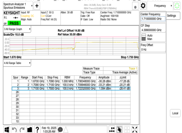
Band66_40MHz_CP_OFDM_SCS30kHz_QPSK_RB1_0_CH346000
