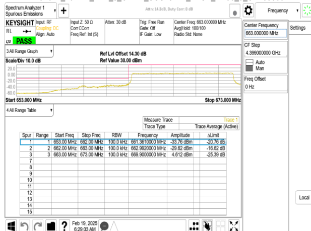
Band71_10MHz_DFT_s_OFDM_SCS15kHz_BPSK_RB50_0_CH133600
