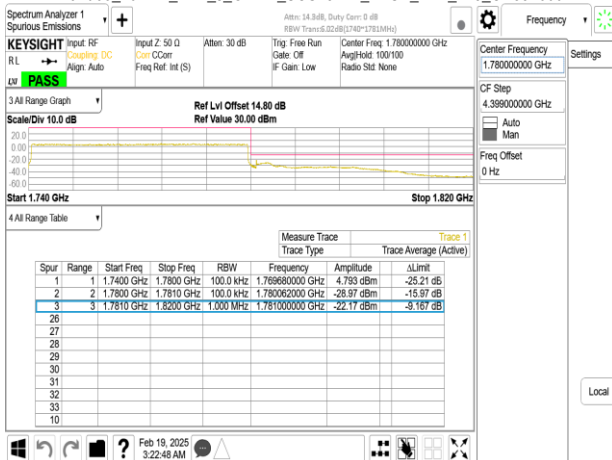
Band66_40MHz_DFT_s_OFDM_SCS15kHz_BPSK_RB216_0_CH352000
