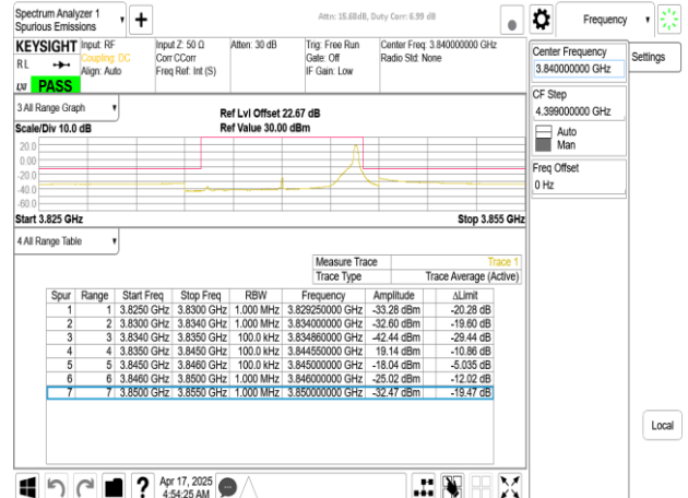
Band77-Part27_10MHz_CP_OFDM_SCS15kHz_QPSK_RB1_51_CH656000
