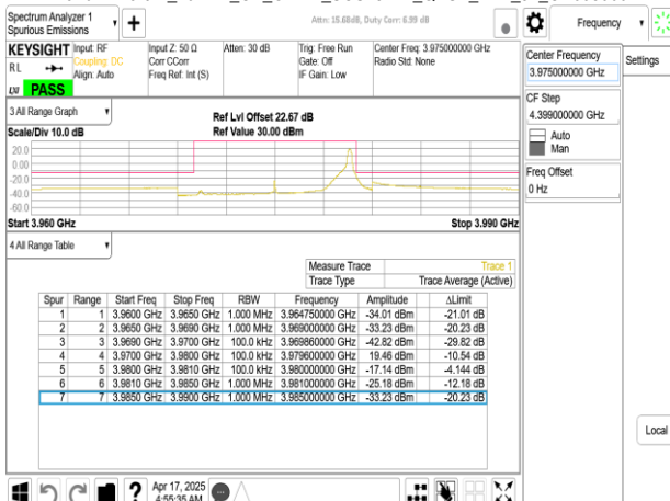
Band77-Part27_10MHz_CP_OFDM_SCS15kHz_QPSK_RB1_51_CH665000
