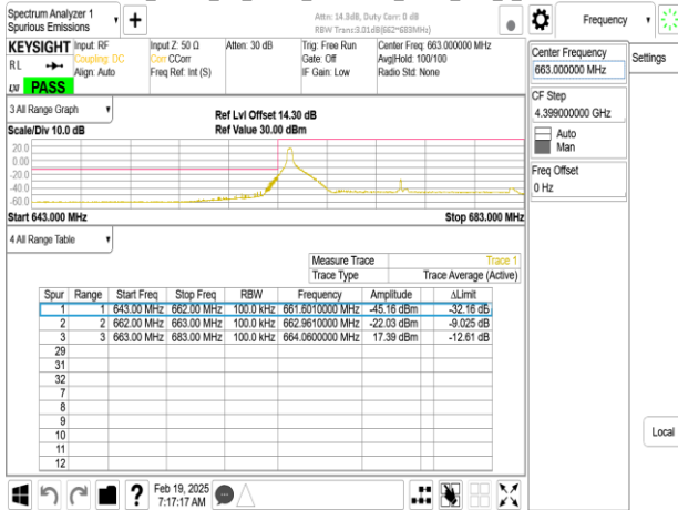
Band71_20MHz_CP_OFDM_SCS30kHz_QPSK_RB51_0_CH134600
