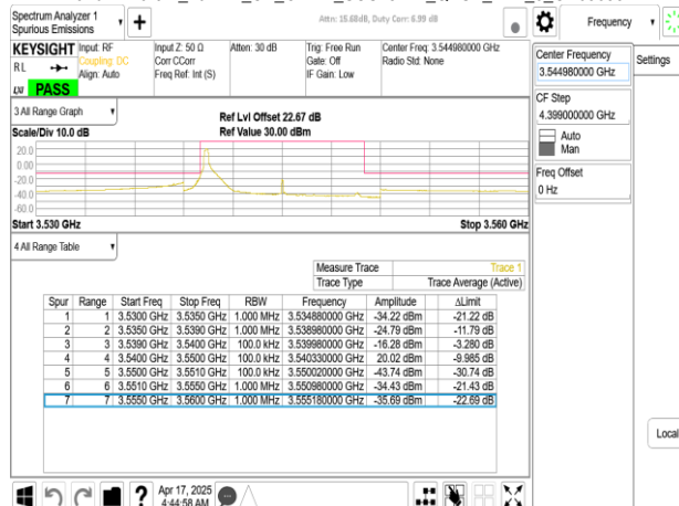
Band77-Part27_10MHz_CP_OFDM_SCS15kHz_QPSK_RB1_51_CH636332
