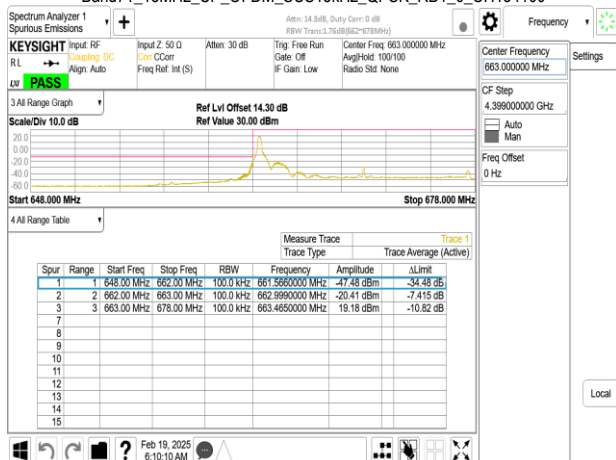
Band71_15MHz_CP_OFDM_SCS15kHz_QPSK_RB79_0_CH134100
