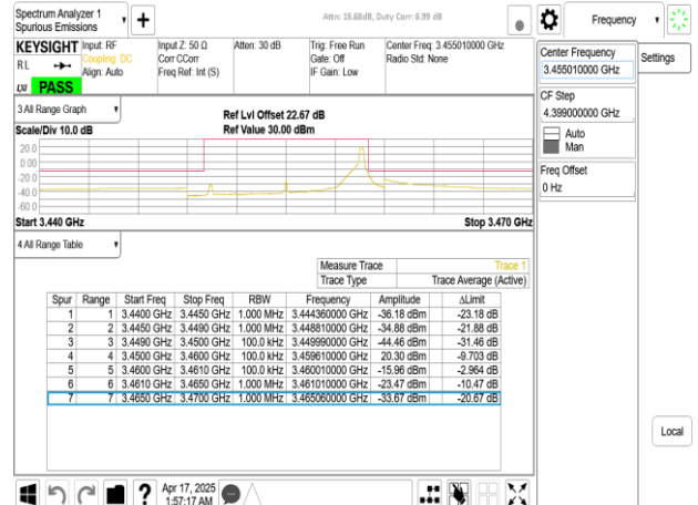
Band77-Part27_10MHz_DFT_s_OFDM_SCS15kHz_BPSK_RB1_51_CH630334
