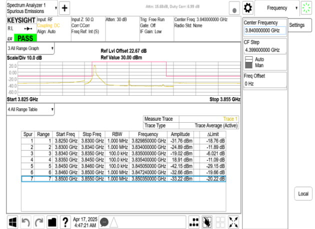
Band77-Part27_10MHz_CP_OFDM_SCS15kHz_QPSK_RB1_51_CH656000
