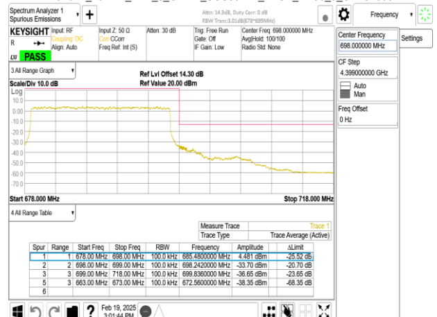
Band71_20MHz_DFT_s_OFDM_SCS30kHz_BPSK_RB50_0_CH137600
