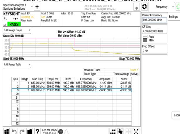
Band71_15MHz_CP_OFDM_SCS30kHz_QPSK_RB38_0_CH138100
