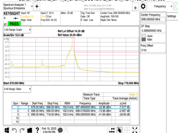
Band71_20MHz_CP_OFDM_SCS15kHz_QPSK_RB106_0_CH134600
