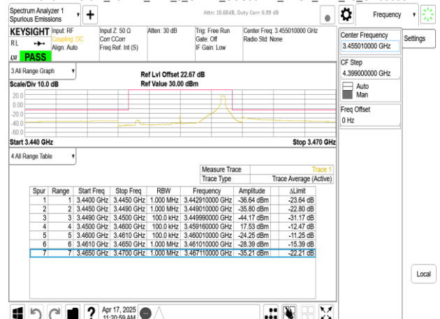
Band77-Part27_10MHz_DFT_s_OFDM_SCS30kHz_BPSK_RB1_23_CH630334
