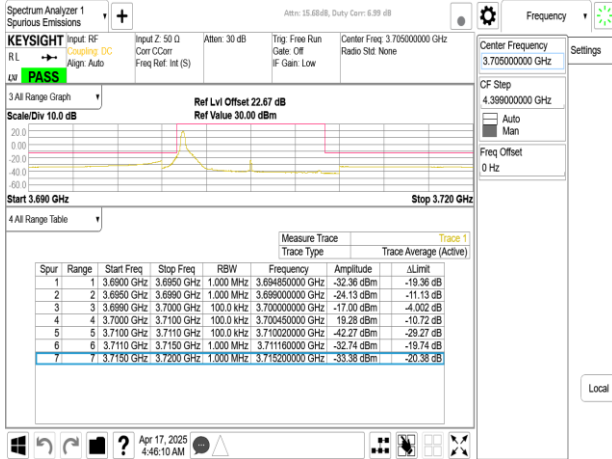
Band77-Part27_10MHz_CP_OFDM_SCS15kHz_QPSK_RB1_51_CH647000
