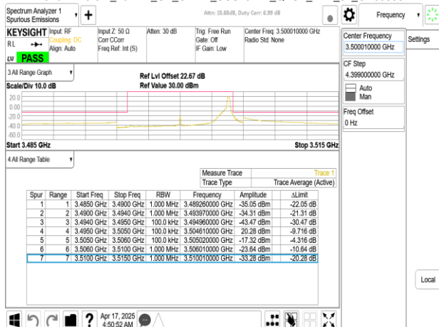
Band77-Part27_10MHz_CP_OFDM_SCS15kHz_QPSK_RB1_51_CH633334
