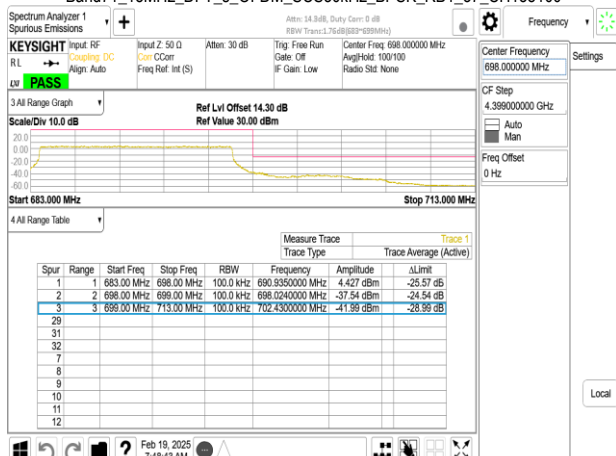
Band71_15MHz_DFT_s_OFDM_SCS30kHz_BPSK_RB36_0_CH138100
