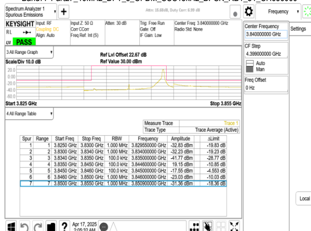
Band77-Part27_10MHz_DFT_s_OFDM_SCS15kHz_BPSK_RB1_51_CH656000
