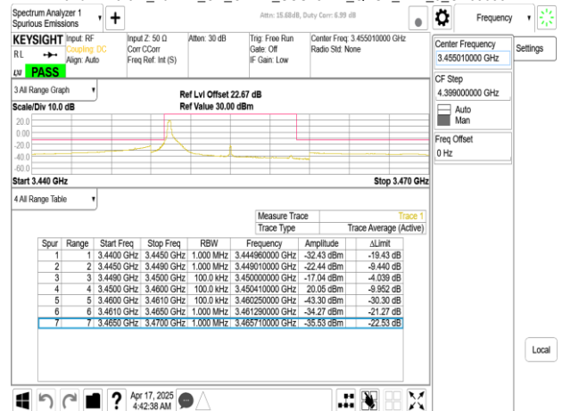
Band77-Part27_10MHz_CP_OFDM_SCS15kHz_QPSK_RB1_51_CH630334
