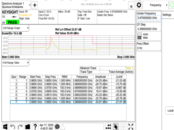
Band77-Part27_10MHz_CP_OFDM_SCS15kHz_QPSK_RB1_51_CH665000
