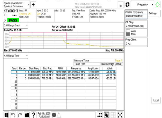
Band71_20MHz_DFT_s_OFDM_SCS30kHz_BPSK_RB50_0_CH137600
