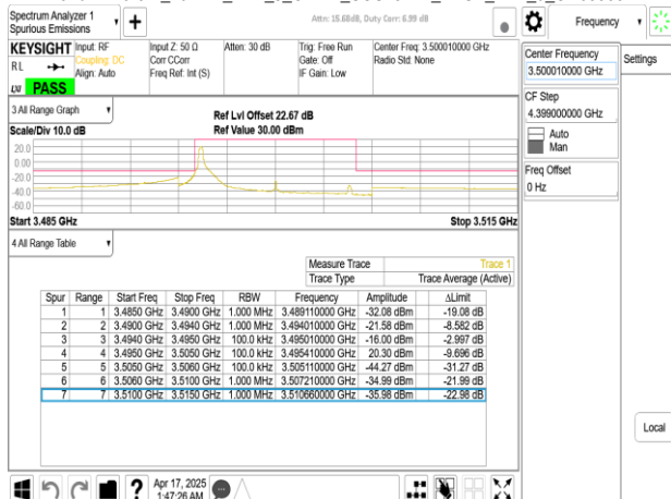
Band77-Part27_10MHz_DFT_s_OFDM_SCS15kHz_BPSK_RB1_51_CH633334
