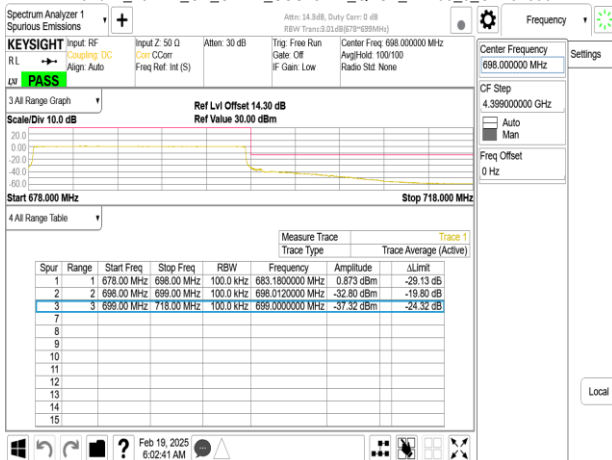
Band71_20MHz_CP_OFDM_SCS15kHz_QPSK_RB1_105_CH137600
