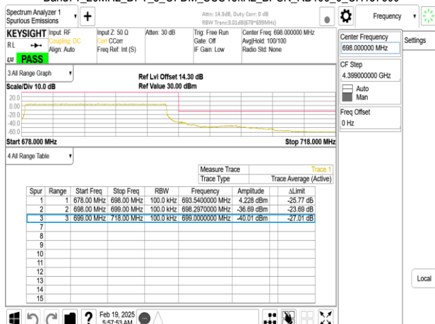
Band71_20MHz_DFT_s_OFDM_SCS15kHz_BPSK_RB100_0_CH137600
