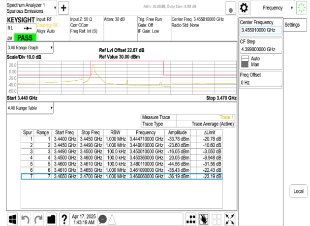
Band77-Part27_10MHz_DFT_s_OFDM_SCS15kHz_BPSK_RB1_51_CH630334
