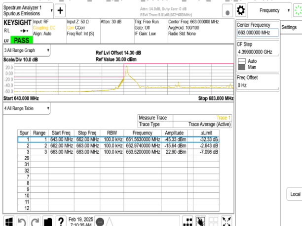
Band71_20MHz_DFT_s_OFDM_SCS30kHz_BPSK_RB1_0_CH134600
