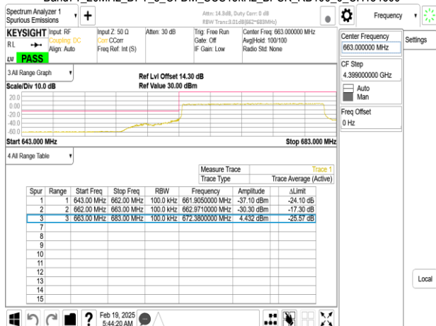
Band71_20MHz_DFT_s_OFDM_SCS15kHz_BPSK_RB1_0_CH134600
