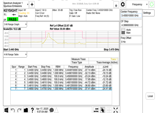
Band77-Part27_10MHz_DFT_s_OFDM_SCS30kHz_BPSK_RB1_23_CH630334
