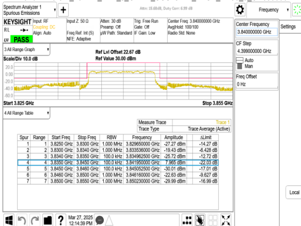
Band77-Part27_10MHz_DFT_s_OFDM_SCS15kHz_BPSK_RB1_0_CH656000
