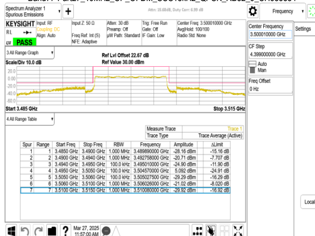
Band77-Part27_10MHz_CP_OFDM_SCS15kHz_QPSK_RB1_0_CH636332
