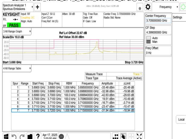
Band77-Part27_10MHz_DFT_s_OFDM_SCS15kHz_BPSK_RB1_51_CH647000
