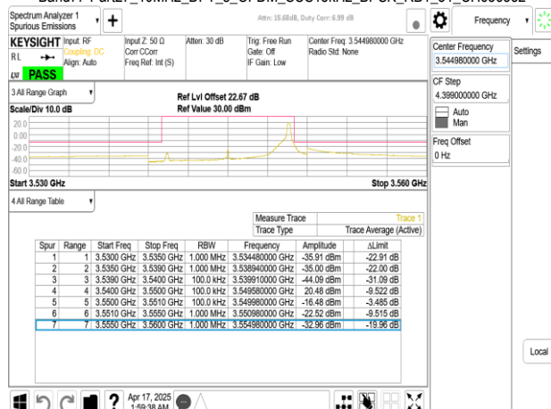
Band77-Part27_10MHz_DFT_s_OFDM_SCS15kHz_BPSK_RB1_51_CH636332
