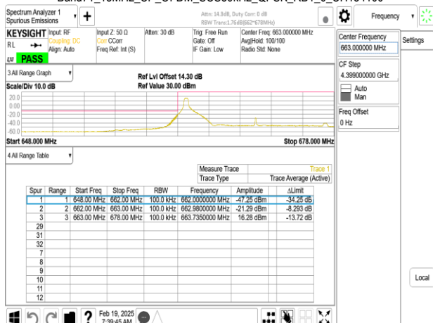
Band71_15MHz_CP_OFDM_SCS30kHz_QPSK_RB1_0_CH134100
