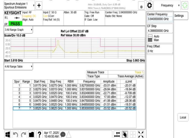
Band77-Part27_15MHz_CP_OFDM_SCS30kHz_QPSK_RB1_37_CH656000
