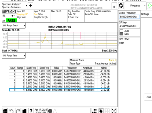
Band77-Part27_20MHz_DFT_s_OFDM_SCS15kHz_BPSK_RB1_0_CH633334
