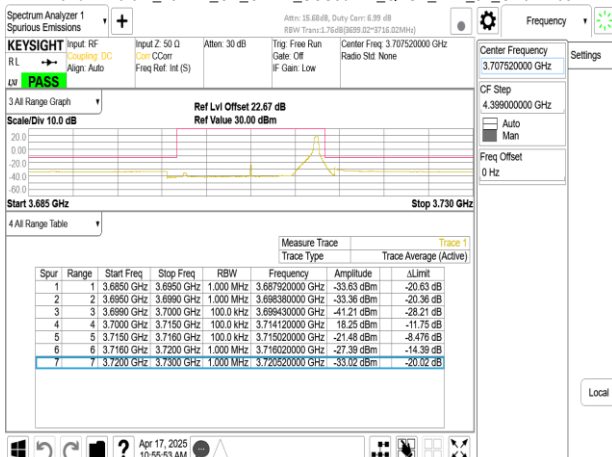
Band77-Part27_15MHz_CP_OFDM_SCS30kHz_QPSK_RB1_37_CH647168
