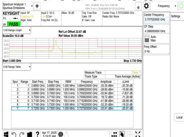
Band77-Part27_15MHz_DFT_s_OFDM_SCS30kHz_BPSK_RB1_37_CH647168
