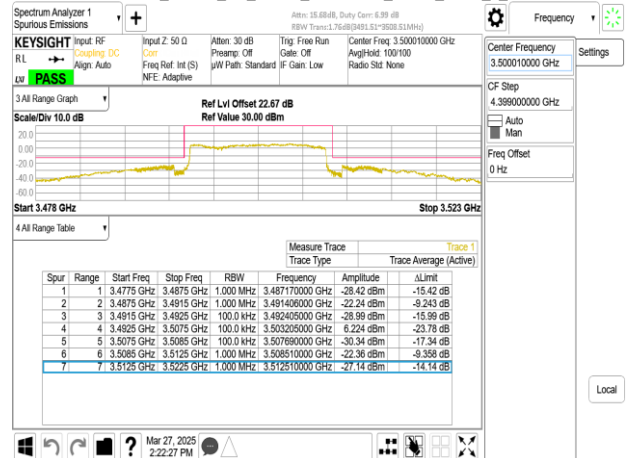
Band77-Part27_15MHz_CP_OFDM_SCS30kHz_QPSK_RB1_0_CH636166
