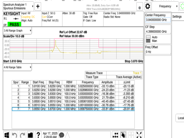
Band77-Part27_20MHz_DFT_s_OFDM_SCS15kHz_BPSK_RB1_0_CH656000
