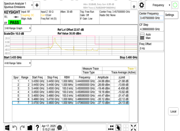
Band77-Part27_15MHz_DFT_s_OFDM_SCS30kHz_BPSK_RB1_37_CH630500
