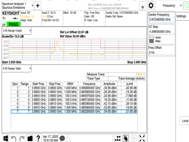
Band77-Part27_15MHz_CP_OFDM_SCS30kHz_QPSK_RB1_37_CH664832
