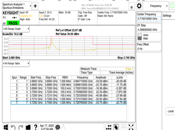
Band77-Part27_20MHz_DFT_s_OFDM_SCS15kHz_BPSK_RB1_0_CH647334
