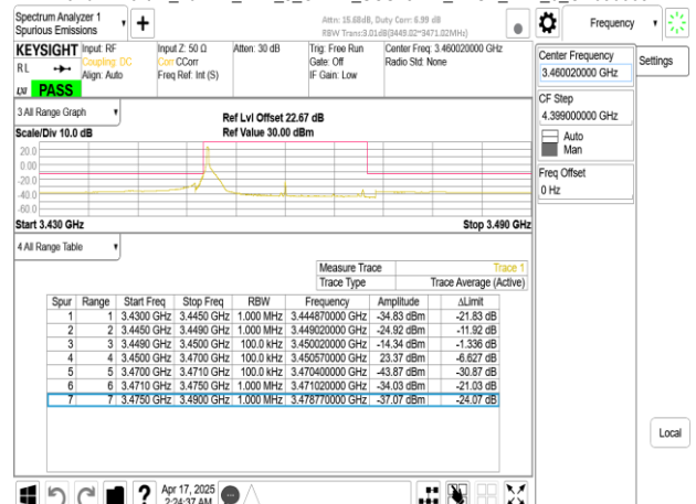
Band77-Part27_20MHz_DFT_s_OFDM_SCS15kHz_BPSK_RB1_0_CH630668
