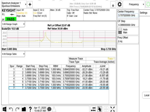
Band77-Part27_15MHz_CP_OFDM_SCS30kHz_QPSK_RB1_37_CH647168
