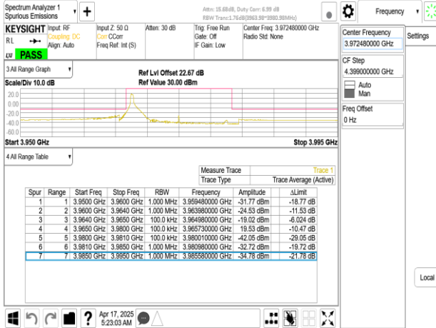
Band77-Part27_15MHz_DFT_s_OFDM_SCS30kHz_BPSK_RB1_37_CH664832
