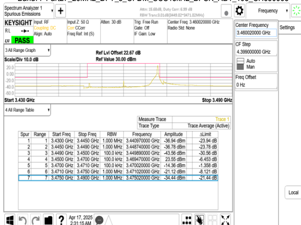
Band77-Part27_20MHz_DFT_s_OFDM_SCS15kHz_BPSK_RB100_0_CH633334
