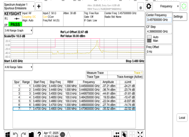
Band77-Part27_15MHz_DFT_s_OFDM_SCS30kHz_BPSK_RB1_37_CH630500
