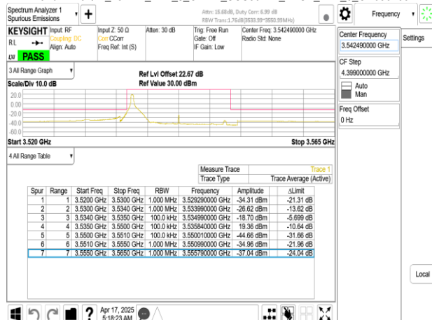
Band77-Part27_15MHz_DFT_s_OFDM_SCS30kHz_BPSK_RB1_37_CH636166
