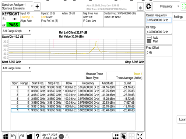
Band77-Part27_15MHz_CP_OFDM_SCS30kHz_QPSK_RB1_37_CH664832
