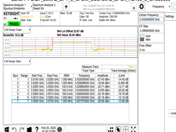
Band77-Part27_20MHz_DFT_s_OFDM_SCS15kHz_BPSK_RB1_0_CH636000
