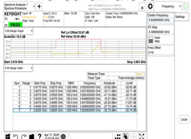
Band77-Part27_15MHz_CP_OFDM_SCS30kHz_QPSK_RB1_37_CH656000
