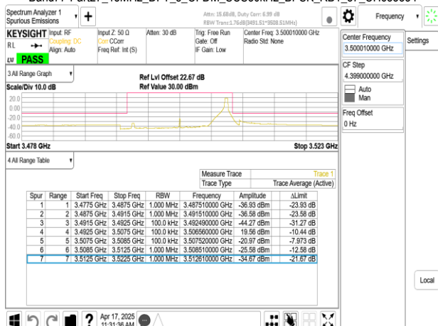
Band77-Part27_15MHz_DFT_s_OFDM_SCS30kHz_BPSK_RB1_37_CH633334
