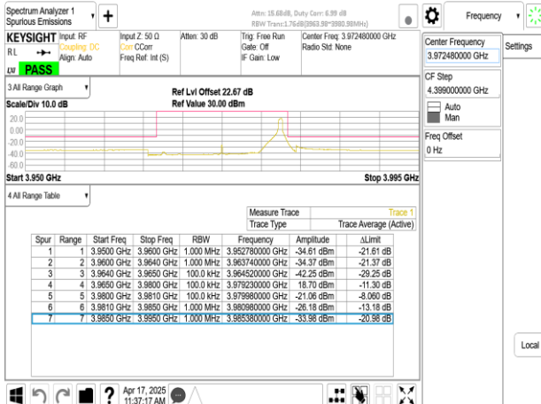
Band77-Part27_15MHz_DFT_s_OFDM_SCS30kHz_BPSK_RB1_37_CH664832
