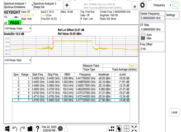
Band77-Part27_20MHz_DFT_s_OFDM_SCS15kHz_BPSK_RB1_0_CH630668
