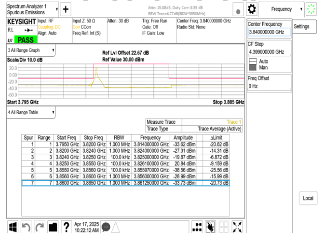
Band77-Part27_30MHz_CP_OFDM_SCS30kHz_QPSK_RB1_77_CH656000
