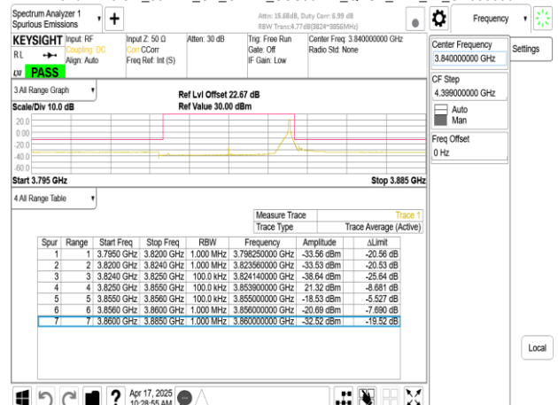
Band77-Part27_30MHz_CP_OFDM_SCS30kHz_QPSK_RB1_77_CH656000
