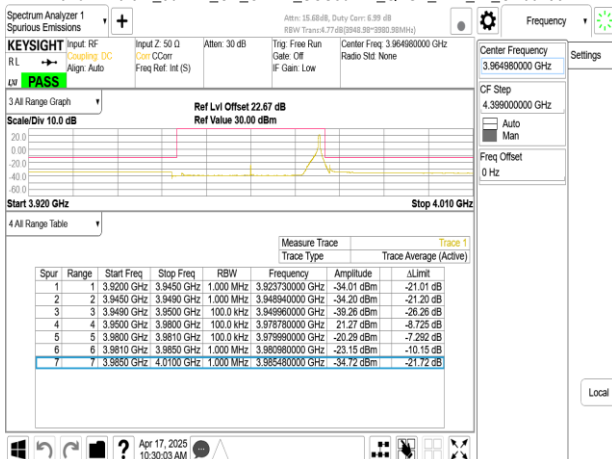
Band77-Part27_30MHz_CP_OFDM_SCS30kHz_QPSK_RB1_77_CH664332
