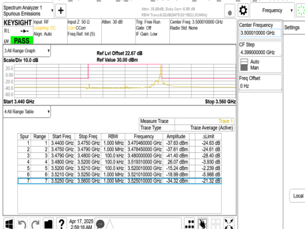
Band77-Part27_40MHz_DFT_s_OFDM_SCS15kHz_BPSK_RB1_215_CH633334
