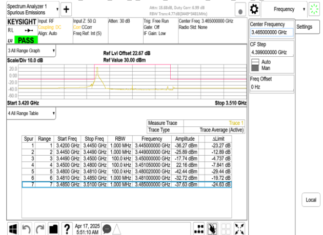
Band77-Part27_30MHz_DFT_s_OFDM_SCS30kHz_BPSK_RB1_77_CH631000
