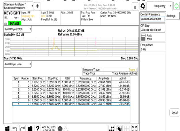
Band77-Part27_30MHz_CP_OFDM_SCS15kHz_QPSK_RB1_0_CH656000
