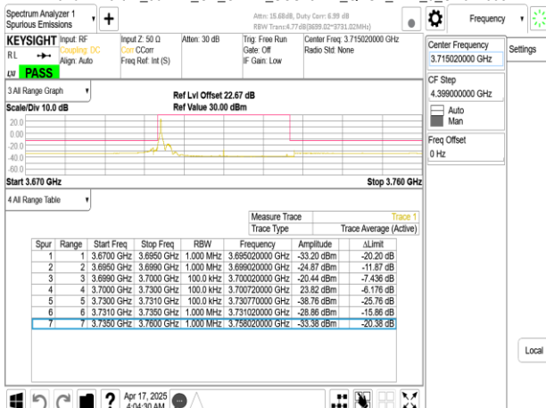
Band77-Part27_30MHz_CP_OFDM_SCS15kHz_QPSK_RB1_0_CH647668
