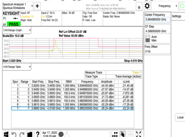
Band77-Part27_30MHz_DFT_s_OFDM_SCS30kHz_BPSK_RB1_77_CH664332
