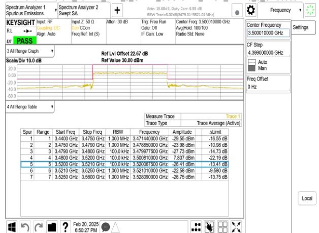
Band77-Part27_40MHz_DFT_s_OFDM_SCS15kHz_BPSK_RB1_0_CH633332
