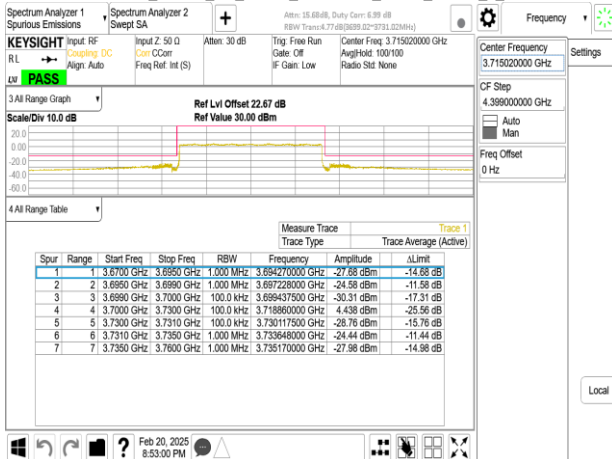
Band77-Part27_30MHz_CP_OFDM_SCS15kHz_QPSK_RB1_0_CH647668
