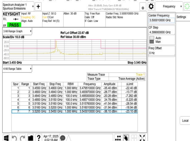
Band77-Part27_30MHz_CP_OFDM_SCS15kHz_QPSK_RB1_0_CH633334
