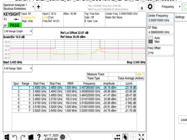
Band77-Part27_30MHz_CP_OFDM_SCS15kHz_QPSK_RB160_0_CH635666
