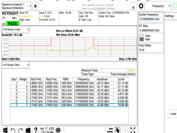
Band77-Part27_40MHz_DFT_s_OFDM_SCS15kHz_BPSK_RB1_215_CH648000
