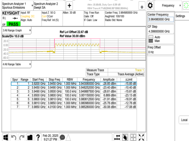
Band77-Part27_30MHz_CP_OFDM_SCS15kHz_QPSK_RB1_0_CH664332
