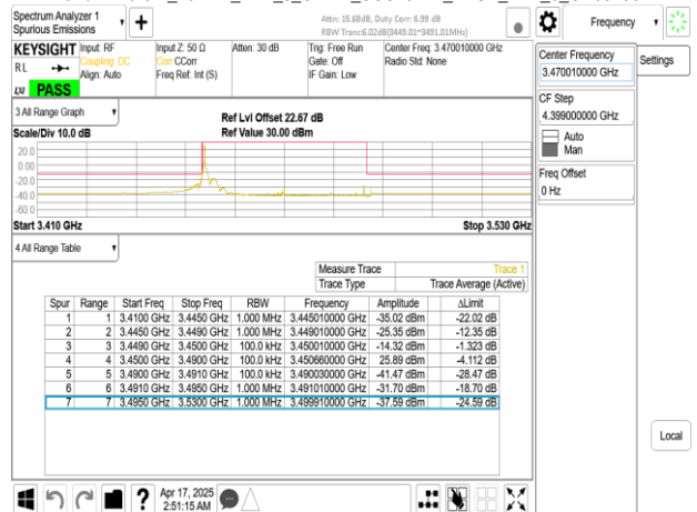
Band77-Part27_40MHz_DFT_s_OFDM_SCS15kHz_BPSK_RB1_215_CH631334
