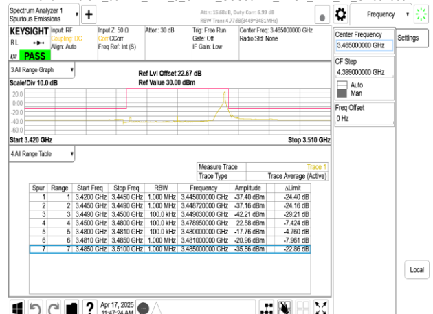
Band77-Part27_30MHz_DFT_s_OFDM_SCS30kHz_BPSK_RB1_77_CH631000
