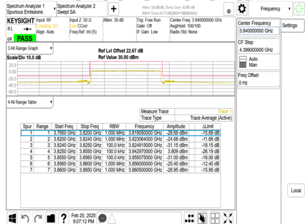
Band77-Part27_30MHz_CP_OFDM_SCS15kHz_QPSK_RB1_0_CH656000
