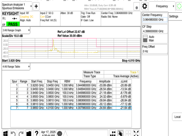
Band77-Part27_30MHz_CP_OFDM_SCS15kHz_QPSK_RB1_0_CH664332
