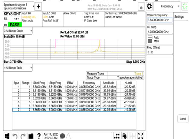
Band77-Part27_40MHz_DFT_s_OFDM_SCS15kHz_BPSK_RB1_215_CH656000
