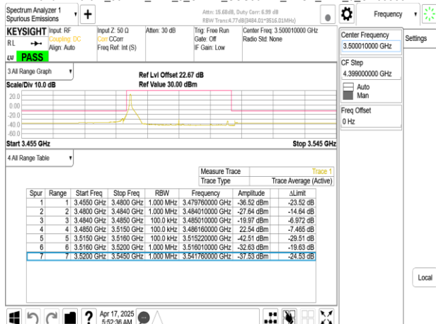
Band77-Part27_30MHz_DFT_s_OFDM_SCS30kHz_BPSK_RB1_77_CH633334
