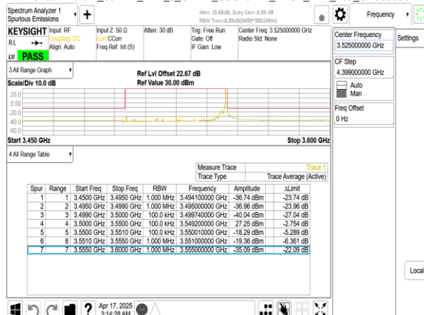
Band77-Part27_50MHz_DFT_s_OFDM_SCS15kHz_BPSK_RB1_269_CH635000
