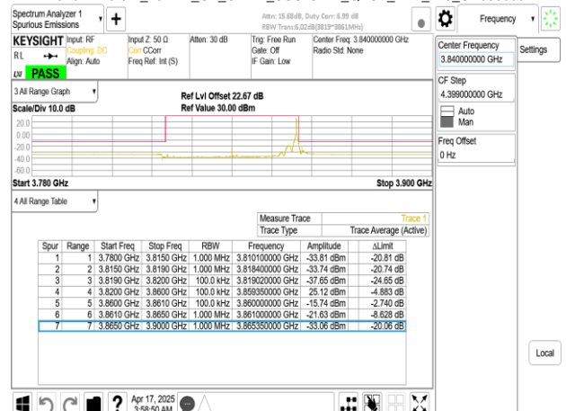
Band77-Part27_40MHz_CP_OFDM_SCS15kHz_QPSK_RB1_215_CH656000
