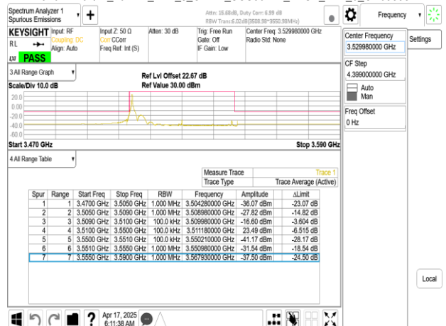
Band77-Part27_40MHz_DFT_s_OFDM_SCS30kHz_BPSK_RB1_0_CH635332
