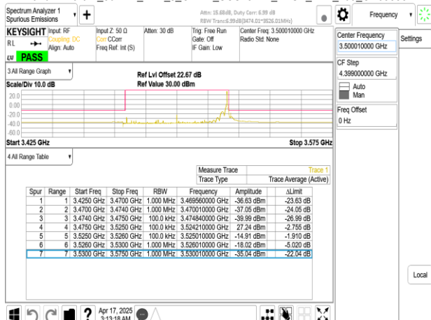
Band77-Part27_50MHz_DFT_s_OFDM_SCS15kHz_BPSK_RB1_269_CH633334
