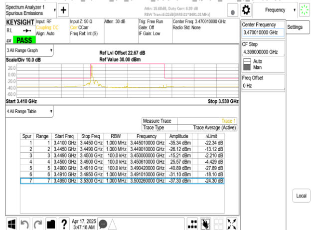
Band77-Part27_40MHz_CP_OFDM_SCS15kHz_QPSK_RB1_215_CH631334
