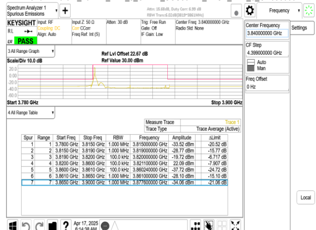
Band77-Part27_40MHz_DFT_s_OFDM_SCS30kHz_BPSK_RB1_0_CH656000
