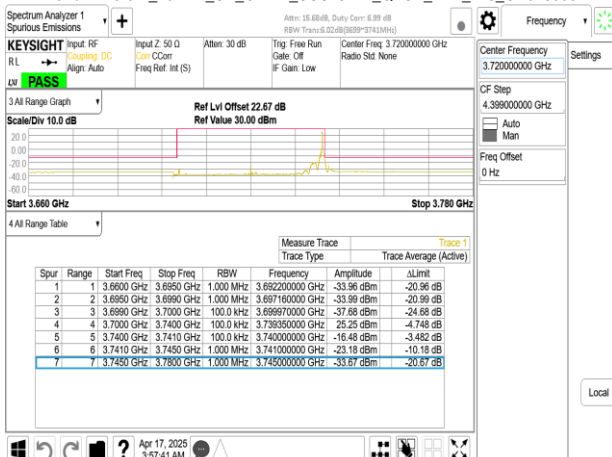
Band77-Part27_40MHz_CP_OFDM_SCS15kHz_QPSK_RB1_215_CH648000
