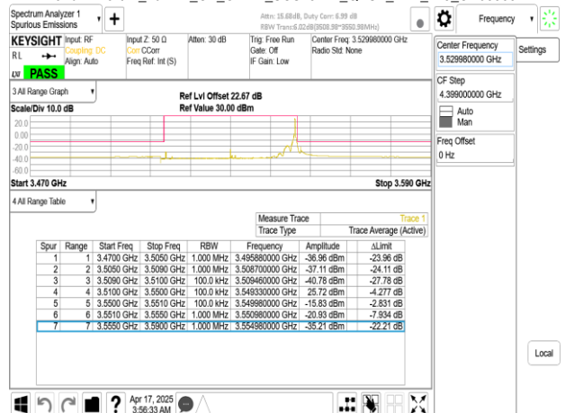
Band77-Part27_40MHz_CP_OFDM_SCS15kHz_QPSK_RB1_215_CH635332
