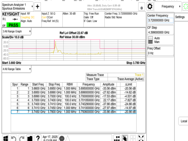
Band77-Part27_40MHz_DFT_s_OFDM_SCS30kHz_BPSK_RB1_0_CH648000
