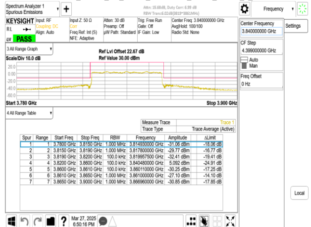
Band77-Part27_40MHz_CP_OFDM_SCS30kHz_QPSK_RB1_0_CH656000
