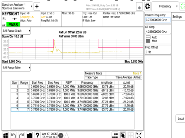
Band77-Part27_40MHz_CP_OFDM_SCS30kHz_QPSK_RB1_0_CH648000
