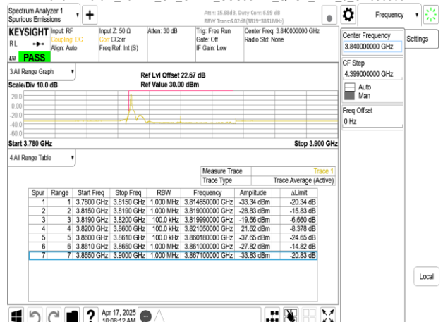
Band77-Part27_40MHz_CP_OFDM_SCS30kHz_QPSK_RB1_0_CH656000
