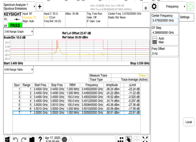
Band77-Part27_50MHz_DFT_s_OFDM_SCS30kHz_BPSK_RB1_0_CH631668
