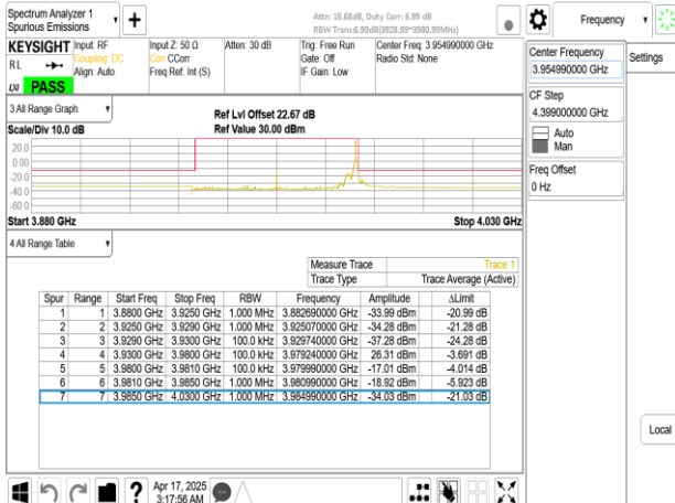
Band77-Part27_50MHz_DFT_s_OFDM_SCS15kHz_BPSK_RB1_269_CH663666
