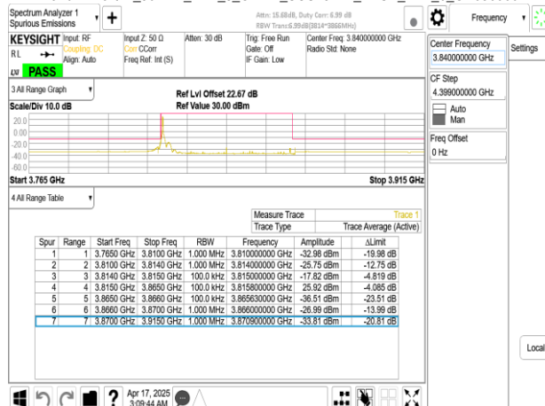
Band77-Part27_50MHz_DFT_s_OFDM_SCS15kHz_BPSK_RB1_269_CH656000
