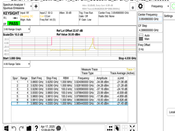
Band77-Part27_50MHz_CP_OFDM_SCS30kHz_QPSK_RB133_0_CH613668
