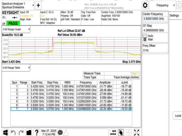
Band77-Part27_50MHz_DFT_s_OFDM_SCS30kHz_BPSK_RB1_0_CH633334
