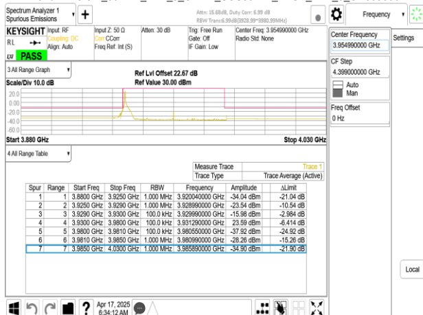
Band77-Part27_50MHz_DFT_s_OFDM_SCS30kHz_BPSK_RB1_0_CH663666
