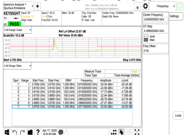
Band77-Part27_50MHz_DFT_s_OFDM_SCS30kHz_BPSK_RB1_0_CH656000
