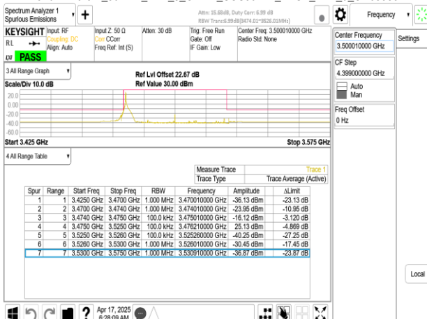
Band77-Part27_50MHz_DFT_s_OFDM_SCS30kHz_BPSK_RB1_0_CH633334
