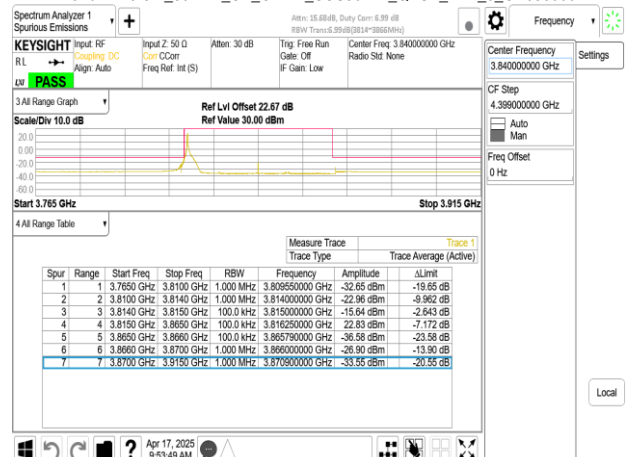
Band77-Part27_50MHz_CP_OFDM_SCS30kHz_QPSK_RB1_0_CH656000
