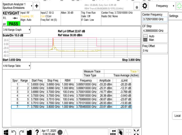
Band77-Part27_50MHz_DFT_s_OFDM_SCS15kHz_BPSK_RB1_269_CH648334
