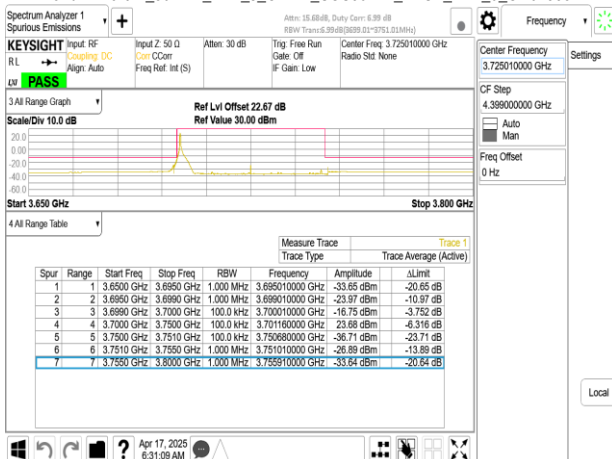
Band77-Part27_50MHz_DFT_s_OFDM_SCS30kHz_BPSK_RB1_0_CH648334
