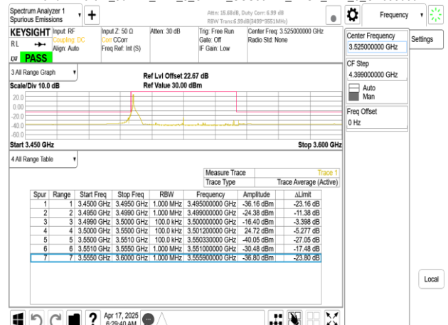
Band77-Part27_50MHz_DFT_s_OFDM_SCS30kHz_BPSK_RB1_0_CH635000
