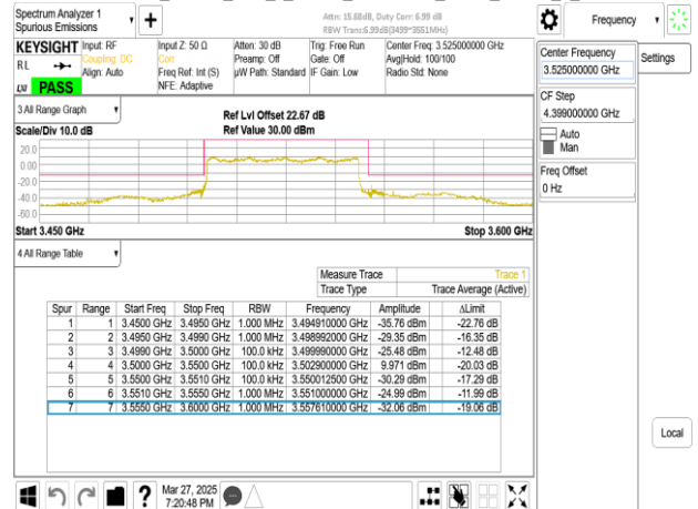
Band77-Part27_50MHz_DFT_s_OFDM_SCS30kHz_BPSK_RB1_0_CH635000
