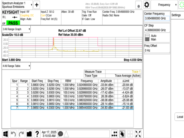
Band77-Part27_50MHz_DFT_s_OFDM_SCS15kHz_BPSK_RB1_269_CH663666
