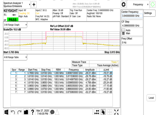
Band77-Part27_50MHz_CP_OFDM_SCS30kHz_QPSK_RB1_0_CH656000
