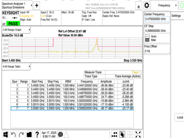
Band77-Part27_50MHz_CP_OFDM_SCS30kHz_QPSK_RB133_0_CH633334
