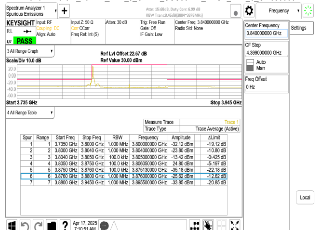
Band77-Part27_70MHz_DFT_s_OFDM_SCS30kHz_BPSK_RB1_0_CH656000
