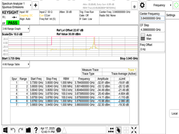
Band77-Part27_70MHz_DFT_s_OFDM_SCS30kHz_BPSK_RB180_0_CH663000
