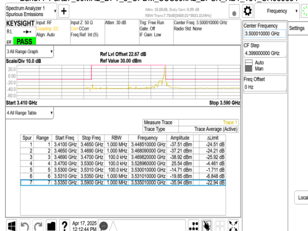
Band77-Part27_60MHz_DFT_s_OFDM_SCS30kHz_BPSK_RB162_0_CH634666
