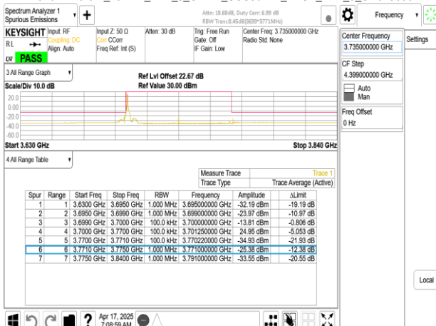
Band77-Part27_70MHz_DFT_s_OFDM_SCS30kHz_BPSK_RB1_0_CH649000
