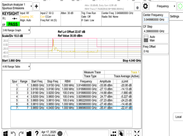
Band77-Part27_60MHz_DFT_s_OFDM_SCS30kHz_BPSK_RB1_0_CH663332
