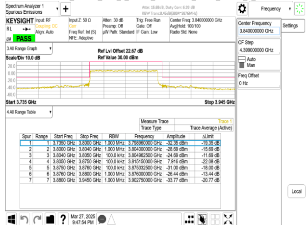
Band77-Part27_70MHz_DFT_s_OFDM_SCS30kHz_BPSK_RB1_0_CH656000
