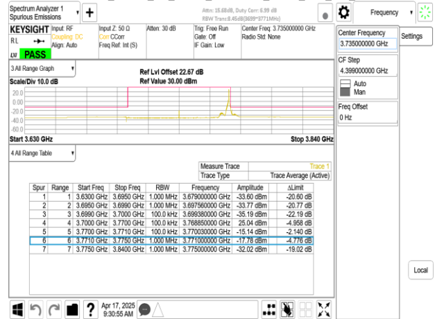
Band77-Part27_70MHz_CP_OFDM_SCS30kHz_QPSK_RB189_0_CH656000
