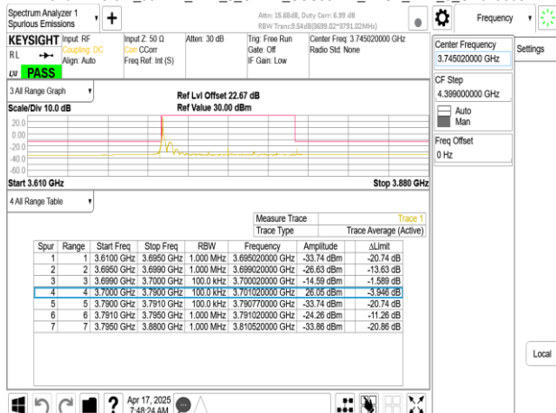
Band77-Part27_90MHz_DFT_s_OFDM_SCS30kHz_BPSK_RB1_244_CH649668
