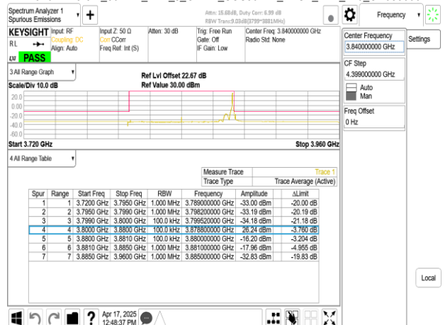
Band77-Part27_80MHz_DFT_s_OFDM_SCS30kHz_BPSK_RB1_216_CH656000
