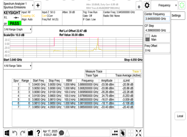
Band77-Part27_80MHz_DFT_s_OFDM_SCS30kHz_BPSK_RB1_0_CH632668
