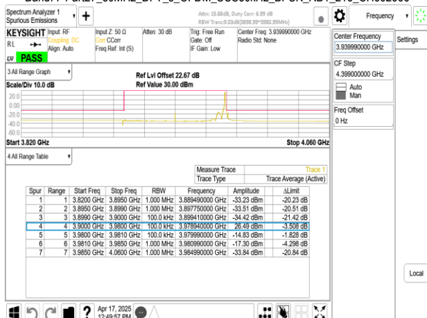
Band77-Part27_80MHz_DFT_s_OFDM_SCS30kHz_BPSK_RB1_216_CH662666
