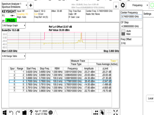
Band77-Part27_80MHz_DFT_s_OFDM_SCS30kHz_BPSK_RB1_216_CH649334
