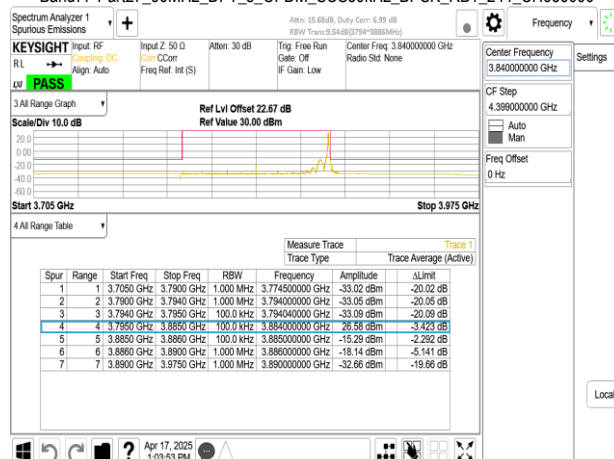
Band77-Part27_90MHz_DFT_s_OFDM_SCS30kHz_BPSK_RB1_244_CH656000
