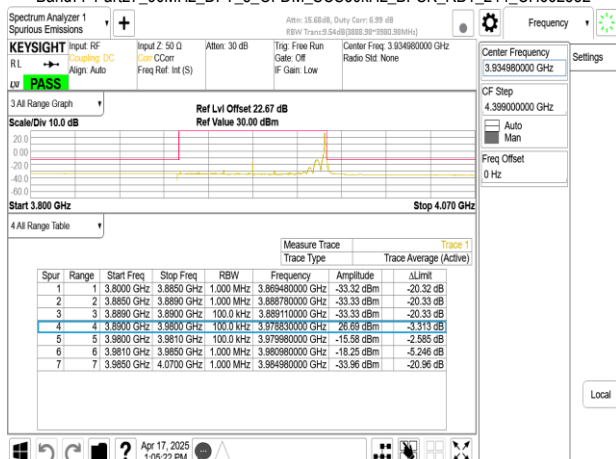
Band77-Part27_90MHz_DFT_s_OFDM_SCS30kHz_BPSK_RB1_244_CH662332
