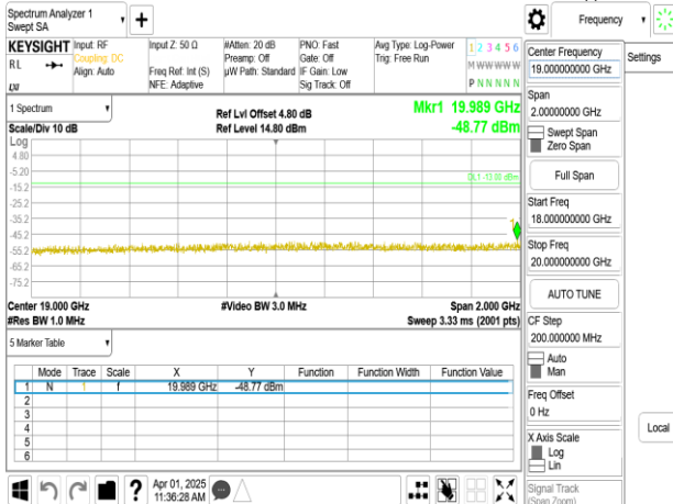
Band25_40MHz_DFT_s_OFDM_SCS15kHz_BPSK_RB1_1_CH379000_upper 18G
