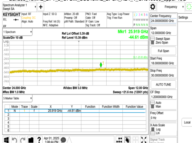
Band38_15MHz_DFT_s_OFDM_SCS15kHz_BPSK_RB1_1_CH522500_upper 18G
