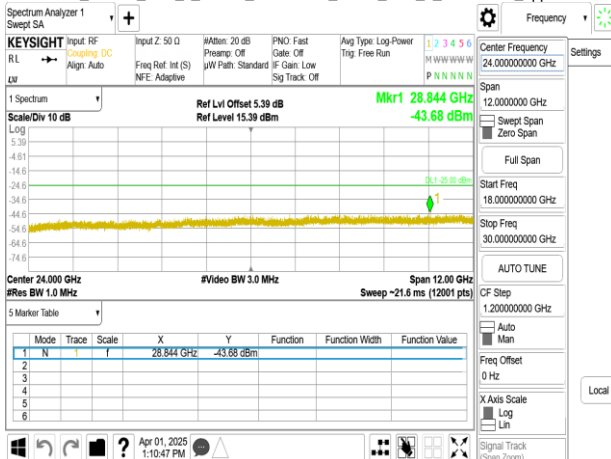
Band38_30MHz_DFT_s_OFDM_SCS30kHz_BPSK_RB1_1_CH517000_upper 18G
