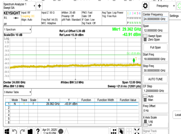
Band38_20MHz_DFT_s_OFDM_SCS15kHz_BPSK_RB1_1_CH516000_upper 18G
