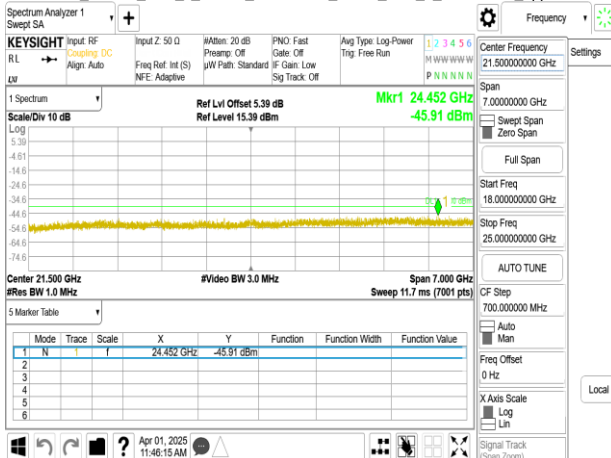
Band30_10MHz_DFT_s_OFDM_SCS30kHz_BPSK_RB1_1_CH462000_upper 18G
