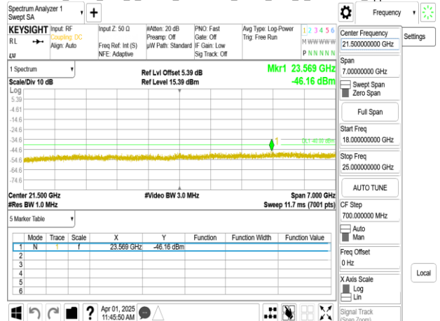
Band30_10MHz_DFT_s_OFDM_SCS15kHz_BPSK_RB1_1_CH515000_upper 18G
