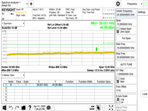
Band38_20MHz_DFT_s_OFDM_SCS30kHz_BPSK_RB1_1_CH516000_upper 18G
