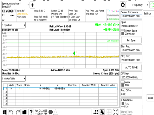
Band2_15MHz_DFT_s_OFDM_SCS30kHz_BPSK_RB1_1_CH376000_upper 18G
