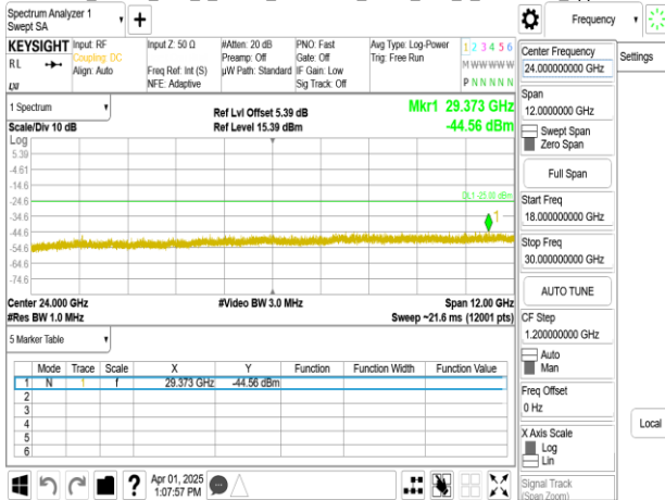
Band38_20MHz_DFT_s_OFDM_SCS15kHz_BPSK_RB1_1_CH522000_upper 18G
