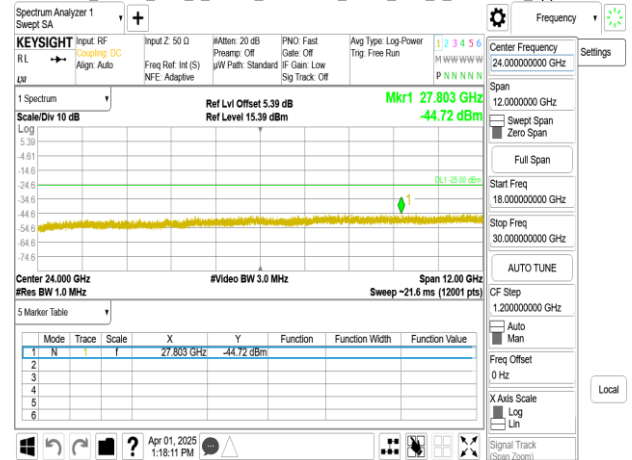
Band38_30MHz_DFT_s_OFDM_SCS30kHz_BPSK_RB1_1_CH521000_upper 18G
