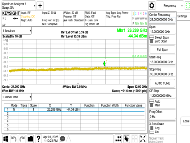
Band38_30MHz_DFT_s_OFDM_SCS15kHz_BPSK_RB1_1_CH521000_upper 18G
