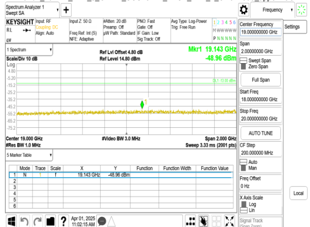
Band2_20MHz_DFT_s_OFDM_SCS15kHz_BPSK_RB1_1_CH376000_upper 18G
