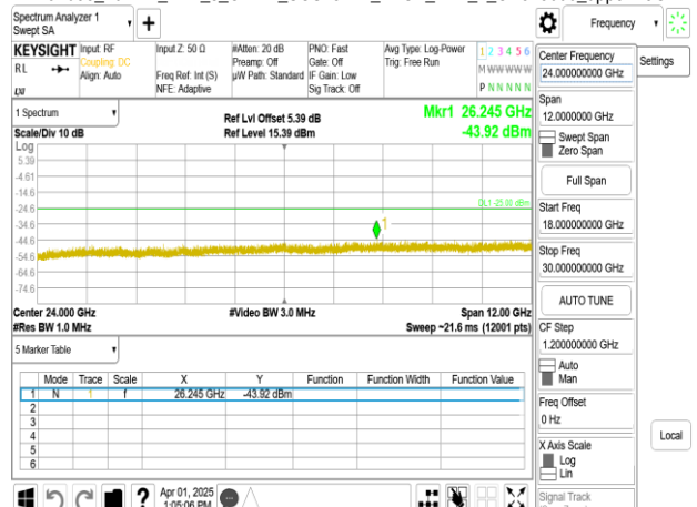
Band30_10MHz_DFT_s_OFDM_SCS15kHz_BPSK_RB1_1_CH515000_upper 18G
