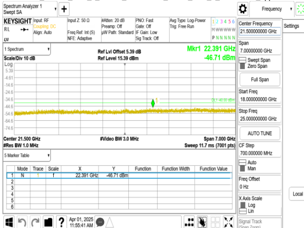
Band30_5MHz_DFT_s_OFDM_SCS15kHz_BPSK_RB1_1_CH461500_upper 18G
