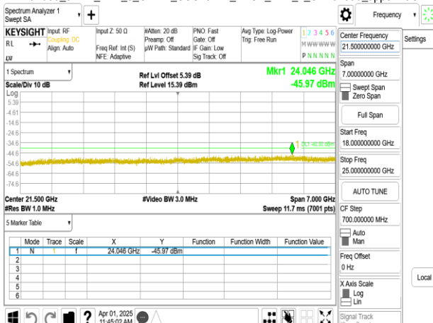
Band30_5MHz_DFT_s_OFDM_SCS15kHz_BPSK_RB1_1_CH461500_upper 18G
