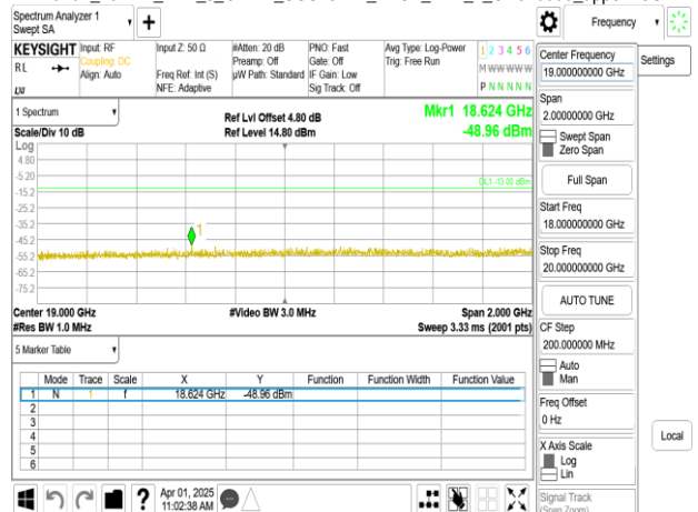
Band2_20MHz_DFT_s_OFDM_SCS15kHz_BPSK_RB1_1_CH380000_upper 18G
