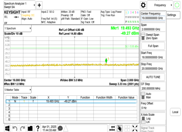
Band25_40MHz_DFT_s_OFDM_SCS30kHz_BPSK_RB1_1_CH379000_upper 18G
