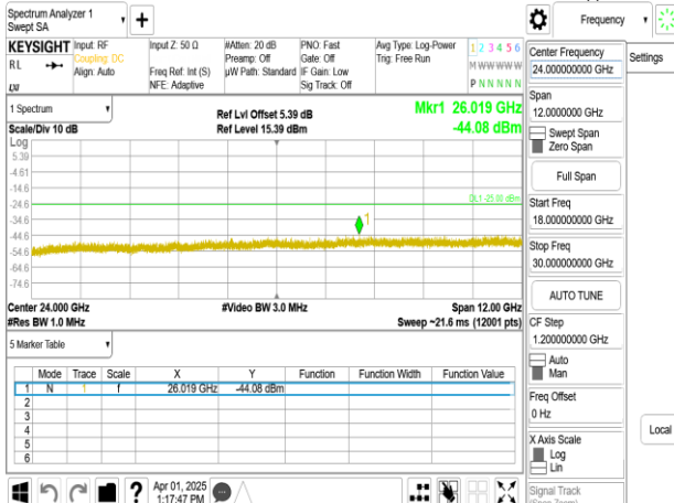
Band38_30MHz_DFT_s_OFDM_SCS30kHz_BPSK_RB1_1_CH517000_upper 18G
