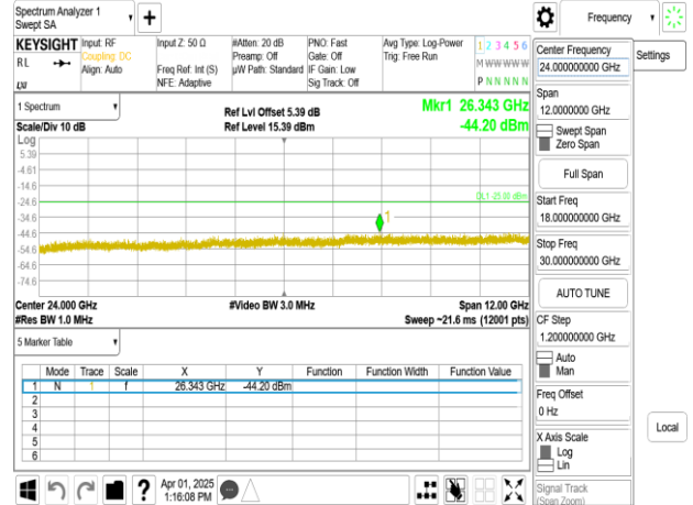
Band38_25MHz_DFT_s_OFDM_SCS15kHz_BPSK_RB1_1_CH516500_upper 18G
