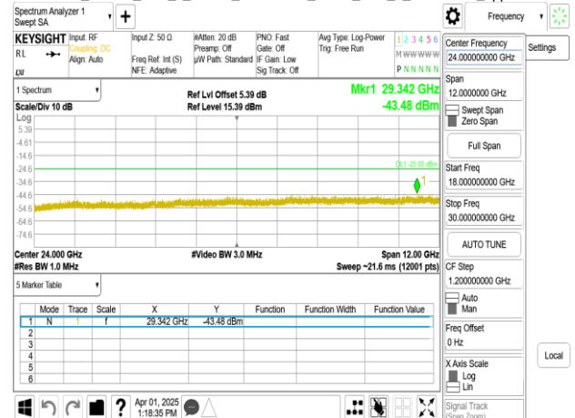
Band38_40MHz_DFT_s_OFDM_SCS15kHz_BPSK_RB1_1_CH518000_upper 18G
