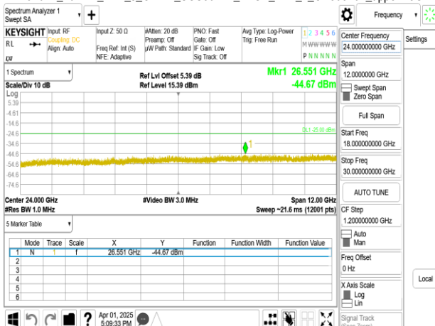
Band41_40MHz_DFT_s_OFDM_SCS30kHz_BPSK_RB1_1_CH503202_upper 18G
