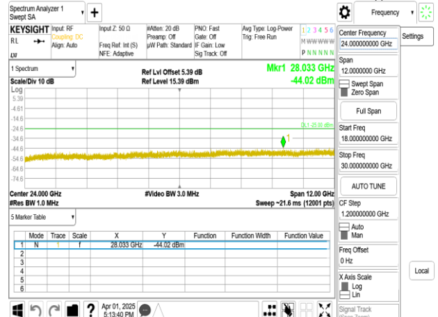
Band41_60MHz_DFT_s_OFDM_SCS30kHz_BPSK_RB1_1_CH531996_upper 18G
