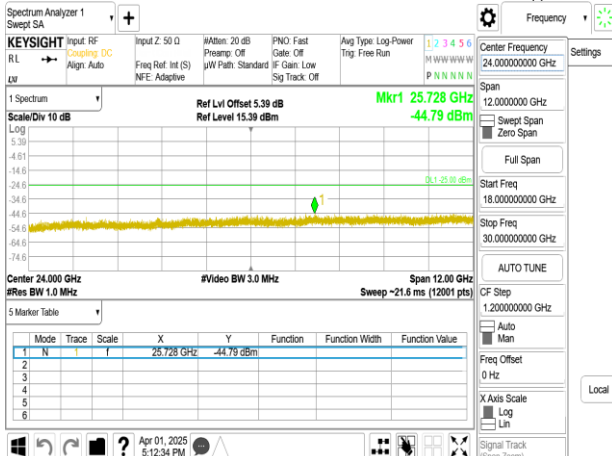
Band41_60MHz_DFT_s_OFDM_SCS30kHz_BPSK_RB1_1_CH505200_upper 18G
