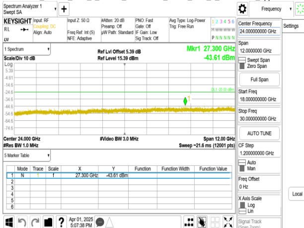
Band41_30MHz_DFT_s_OFDM_SCS15kHz_BPSK_RB1_1_CH502200_upper 18G
