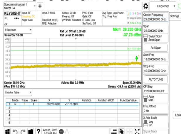
Band77-Part27_10MHz_DFT_s_OFDM_SCS15kHz_BPSK_RB1_1_CH650000_upper 18G
