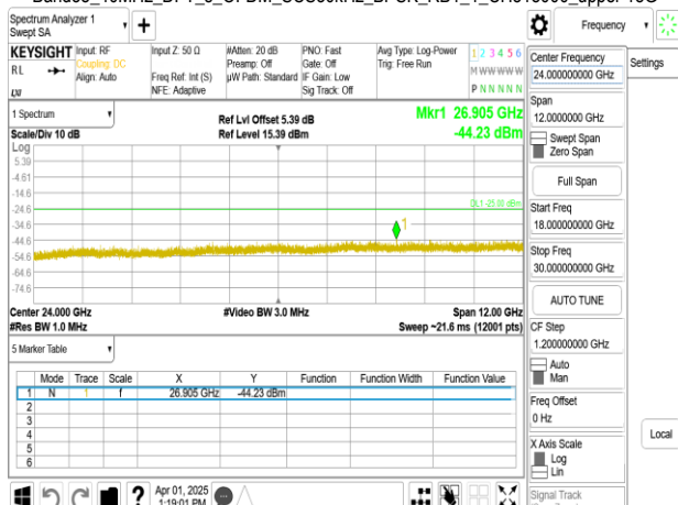
Band38_40MHz_DFT_s_OFDM_SCS30kHz_BPSK_RB1_1_CH518000_upper 18G
