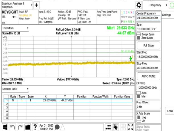
Band41_40MHz_DFT_s_OFDM_SCS15kHz_BPSK_RB1_1_CH534000_upper 18G
