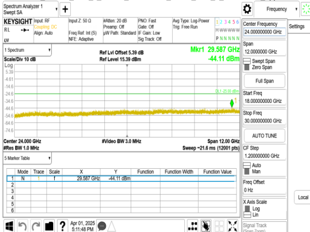
Band41_50MHz_DFT_s_OFDM_SCS30kHz_BPSK_RB1_1_CH532998_upper 18G
