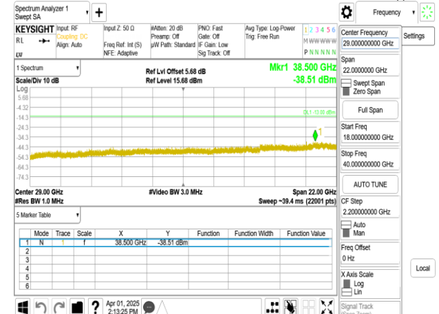
Band77-Part27_100MHz_DFT_s_OFDM_SCS30kHz_BPSK_RB1_1_CH662000_upper 18G
