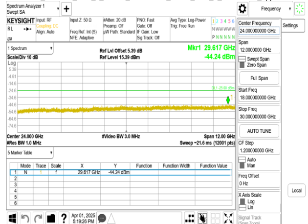
Band41_100MHz_DFT_s_OFDM_SCS30kHz_BPSK_RB1_1_CH528000_upper 18G
