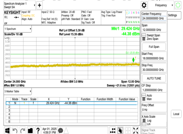
Band41_30MHz_DFT_s_OFDM_SCS15kHz_BPSK_RB1_1_CH534996_upper 18G
