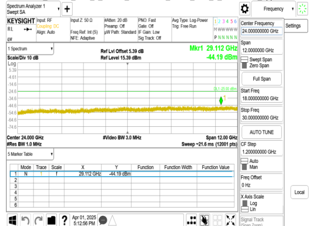
Band41_60MHz_DFT_s_OFDM_SCS30kHz_BPSK_RB1_1_CH518604_upper 18G
