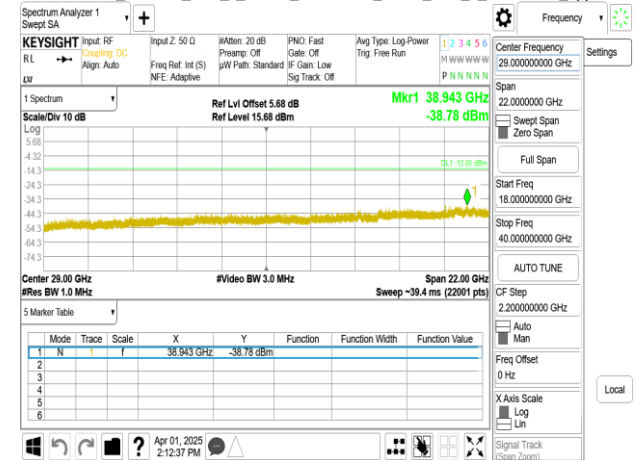
Band77-Part27_100MHz_DFT_s_OFDM_SCS30kHz_BPSK_RB1_1_CH656000_upper 18G
