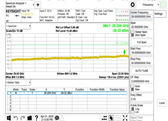
Band77-Part27_100MHz_DFT_s_OFDM_SCS30kHz_BPSK_RB1_1_CH662000_upper 18G
