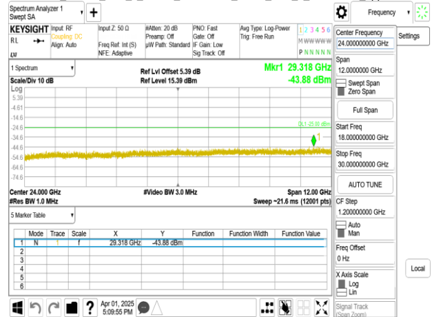
Band41_40MHz_DFT_s_OFDM_SCS30kHz_BPSK_RB1_1_CH518604_upper 18G
