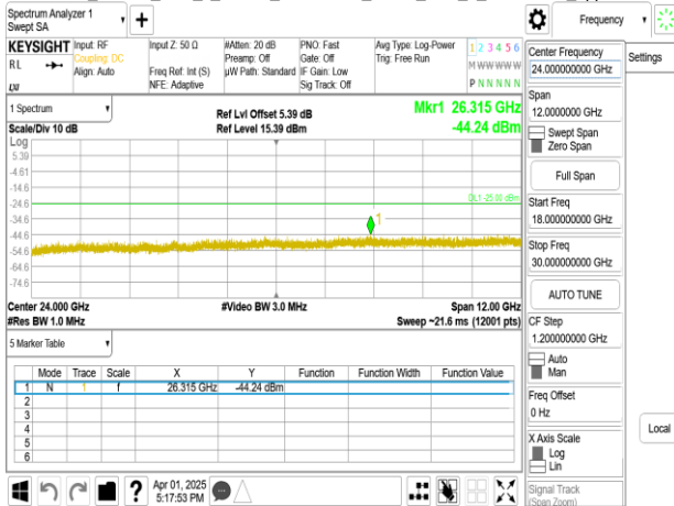
Band41_90MHz_DFT_s_OFDM_SCS30kHz_BPSK_RB1_1_CH528996_upper 18G
