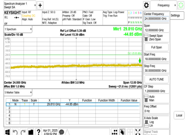
Band41_30MHz_DFT_s_OFDM_SCS15kHz_BPSK_RB1_1_CH534996_upper 18G
