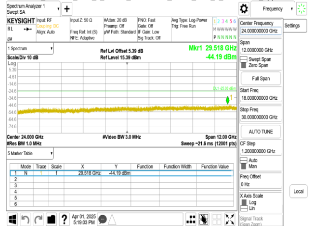
Band41_100MHz_DFT_s_OFDM_SCS30kHz_BPSK_RB1_1_CH518604_upper 18G
