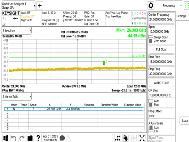
Band41_30MHz_DFT_s_OFDM_SCS30kHz_BPSK_RB1_1_CH518604_upper 18G
