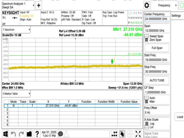
Band38_5MHz_DFT_s_OFDM_SCS15kHz_BPSK_RB1_1_CH523500_upper 18G
