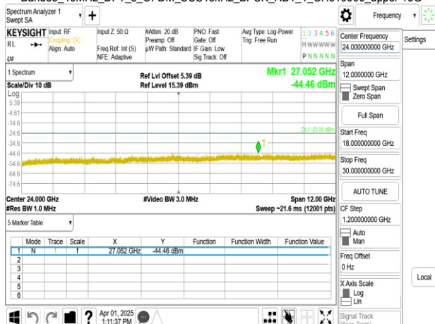
Band38_40MHz_DFT_s_OFDM_SCS15kHz_BPSK_RB1_1_CH520000_upper 18G
