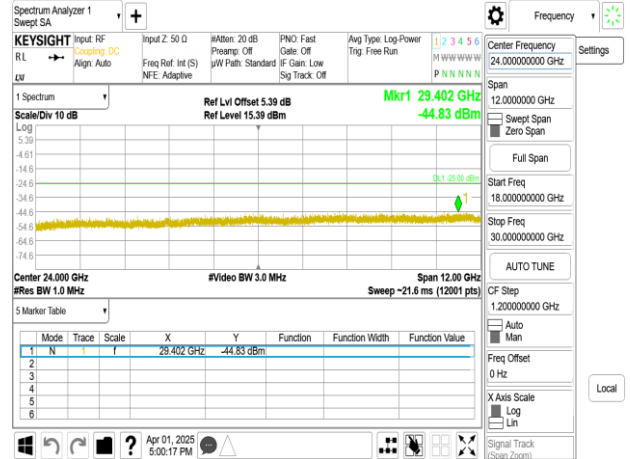
Band41_40MHz_DFT_s_OFDM_SCS15kHz_BPSK_RB1_1_CH504000_upper 18G
