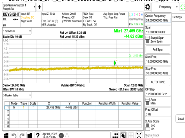
Band41_80MHz_DFT_s_OFDM_SCS30kHz_BPSK_RB1_1_CH518604_upper 18G
