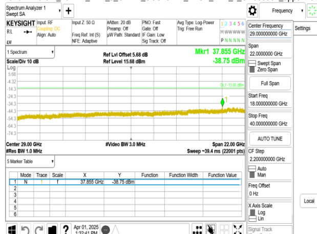
Band77-Part27_10MHz_DFT_s_OFDM_SCS15kHz_BPSK_RB1_1_CH636332_upper 18G
