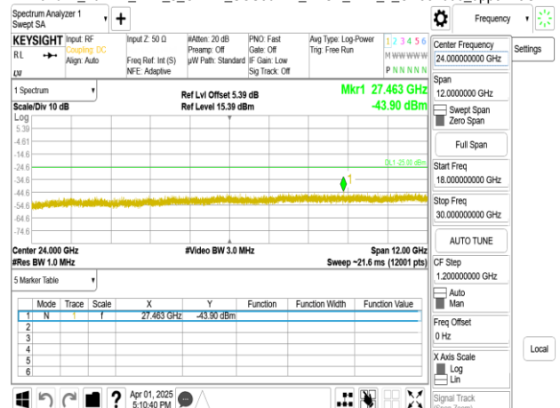
Band41_40MHz_DFT_s_OFDM_SCS30kHz_BPSK_RB1_1_CH534000_upper 18G
