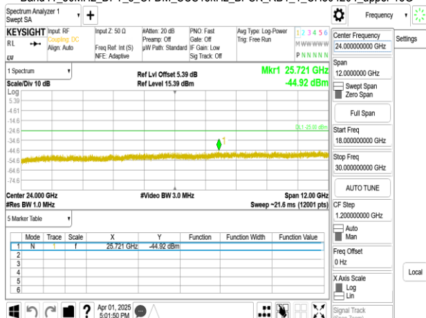
Band41_50MHz_DFT_s_OFDM_SCS15kHz_BPSK_RB1_1_CH505002_upper 18G
