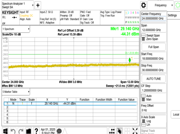
Band41_100MHz_DFT_s_OFDM_SCS30kHz_BPSK_RB1_1_CH509202_upper 18G
