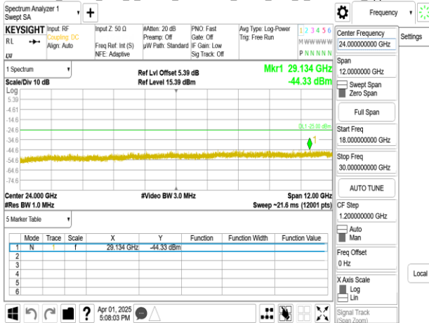
Band41_30MHz_DFT_s_OFDM_SCS30kHz_BPSK_RB1_1_CH503004_upper 18G
