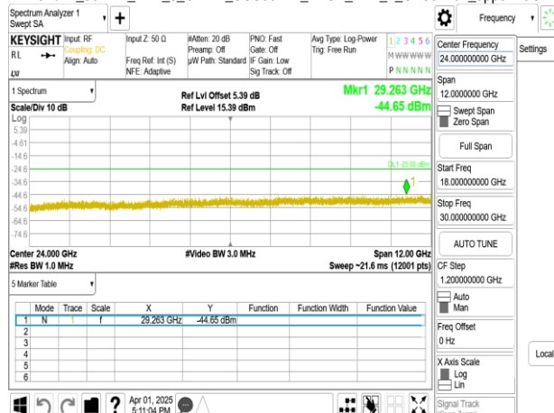
Band41_50MHz_DFT_s_OFDM_SCS30kHz_BPSK_RB1_1_CH505002_upper 18G
