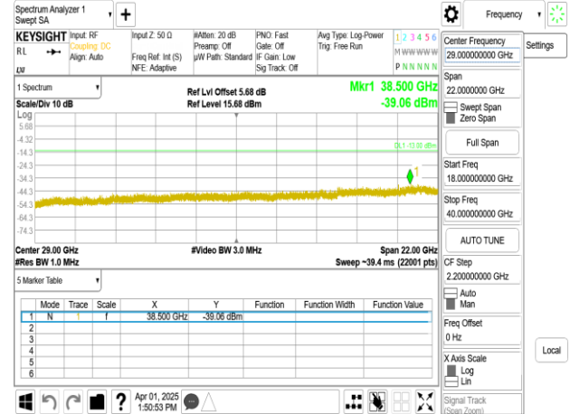
Band77-Part27_15MHz_DFT_s_OFDM_SCS30kHz_BPSK_RB1_1_CH656000_upper 18G
