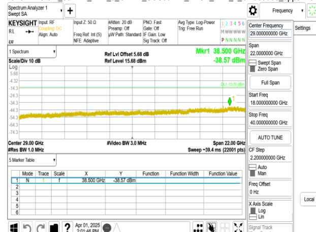
Band77-Part27_50MHz_DFT_s_OFDM_SCS30kHz_BPSK_RB1_1_CH663666_upper 18G
