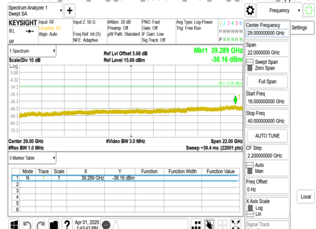
Band77-Part27_40MHz_DFT_s_OFDM_SCS15kHz_BPSK_RB1_1_CH664000_upper 18G
