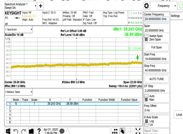
Band77-Part27_20MHz_DFT_s_OFDM_SCS15kHz_BPSK_RB1_1_CH656000_upper 18G
