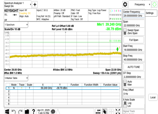
Band77-Part27_10MHz_DFT_s_OFDM_SCS30kHz_BPSK_RB1_1_CH656000_upper 18G
