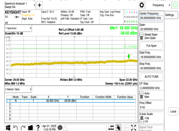
Band77-Part27_40MHz_DFT_s_OFDM_SCS15kHz_BPSK_RB1_1_CH664000_upper 18G
