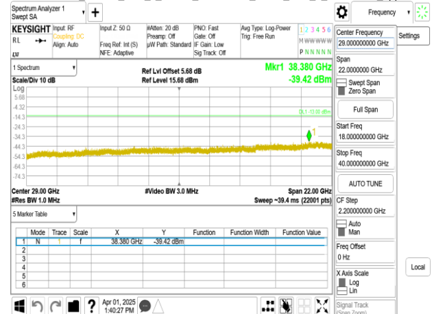
Band77-Part27_30MHz_DFT_s_OFDM_SCS15kHz_BPSK_RB1_1_CH656000_upper 18G
