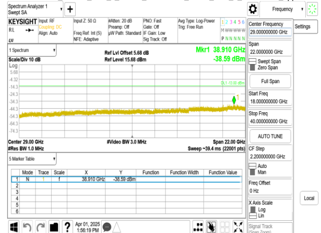
Band77-Part27_30MHz_DFT_s_OFDM_SCS30kHz_BPSK_RB1_1_CH664332_upper 18G
