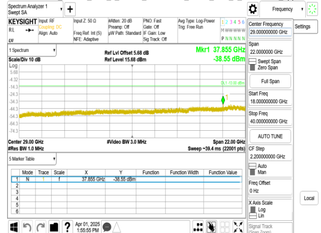
Band77-Part27_30MHz_DFT_s_OFDM_SCS30kHz_BPSK_RB1_1_CH656000_upper 18G
