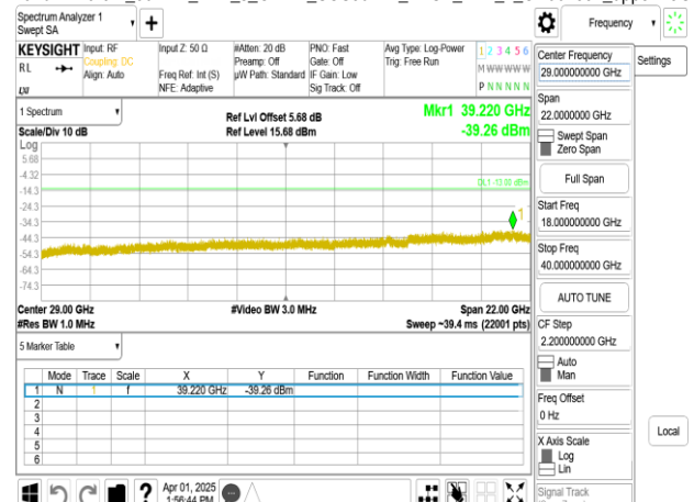
Band77-Part27_30MHz_DFT_s_OFDM_SCS30kHz_BPSK_RB1_1_CH664332_upper 18G
