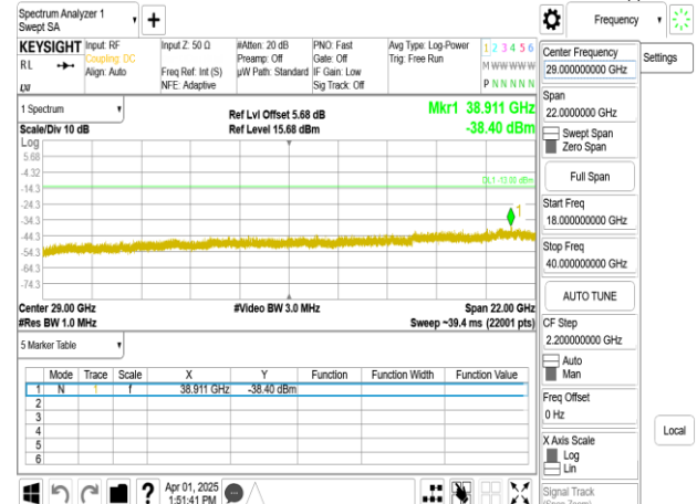
Band77-Part27_15MHz_DFT_s_OFDM_SCS30kHz_BPSK_RB1_1_CH664832_upper 18G
