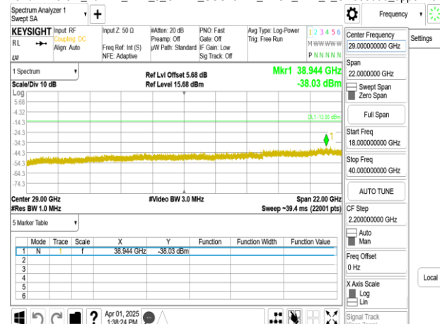
Band77-Part27_20MHz_DFT_s_OFDM_SCS15kHz_BPSK_RB1_1_CH664666_upper 18G
