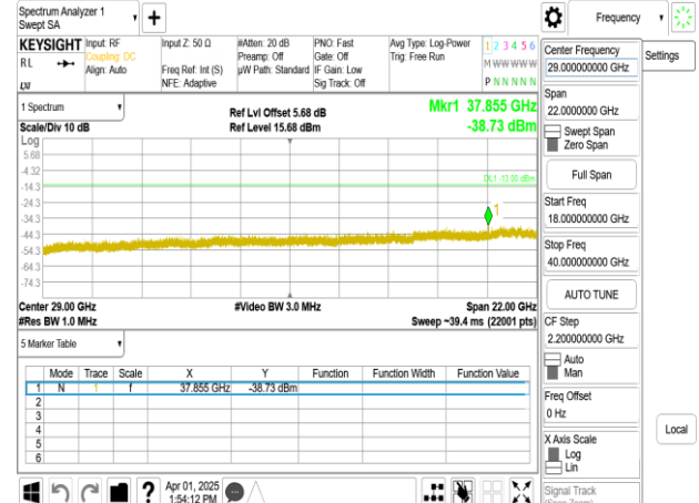
Band77-Part27_20MHz_DFT_s_OFDM_SCS30kHz_BPSK_RB1_1_CH664666_upper 18G
