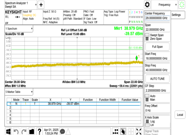
Band77-Part27_20MHz_DFT_s_OFDM_SCS30kHz_BPSK_RB1_1_CH656000_upper 18G
