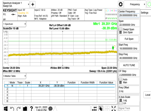
Band77-Part27_40MHz_DFT_s_OFDM_SCS30kHz_BPSK_RB1_1_CH635332_upper 18G
