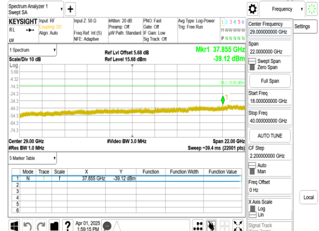
Band77-Part27_40MHz_DFT_s_OFDM_SCS30kHz_BPSK_RB1_1_CH664000_upper 18G
