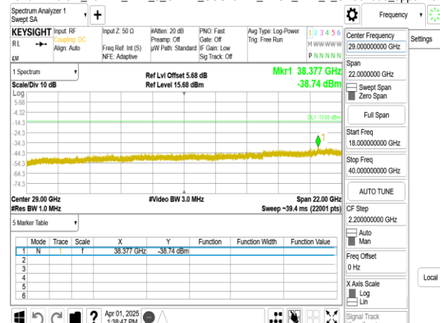
Band77-Part27_20MHz_DFT_s_OFDM_SCS15kHz_BPSK_RB1_1_CH664666_upper 18G
