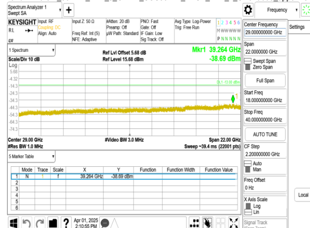
Band77-Part27_90MHz_DFT_s_OFDM_SCS30kHz_BPSK_RB1_1_CH656000_upper 18G
