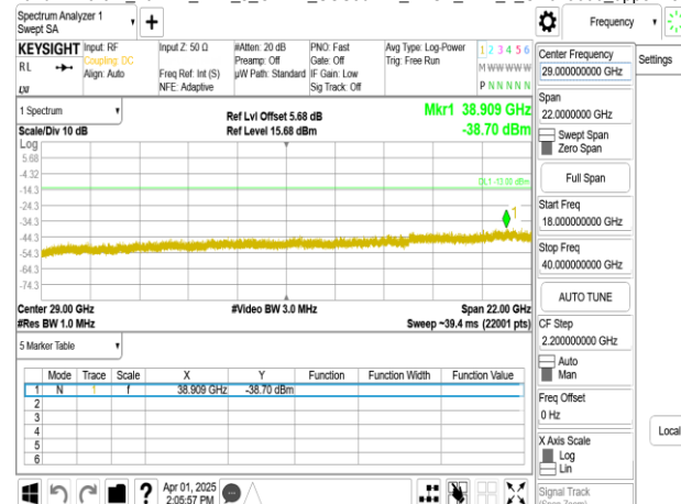
Band77-Part27_70MHz_DFT_s_OFDM_SCS30kHz_BPSK_RB1_1_CH656000_upper 18G
