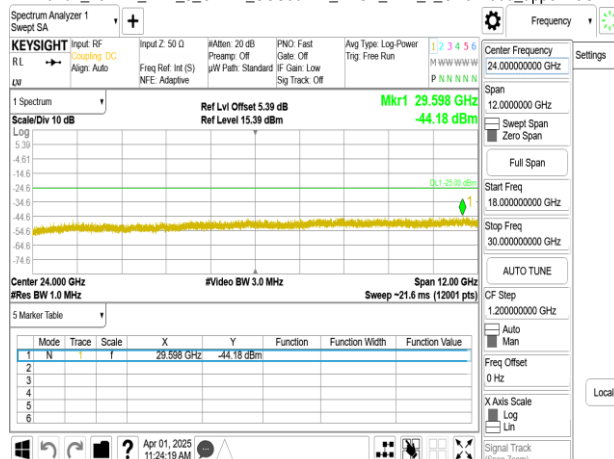
Band7_25MHz_DFT_s_OFDM_SCS30kHz_BPSK_RB1_1_CH511500_upper 18G
