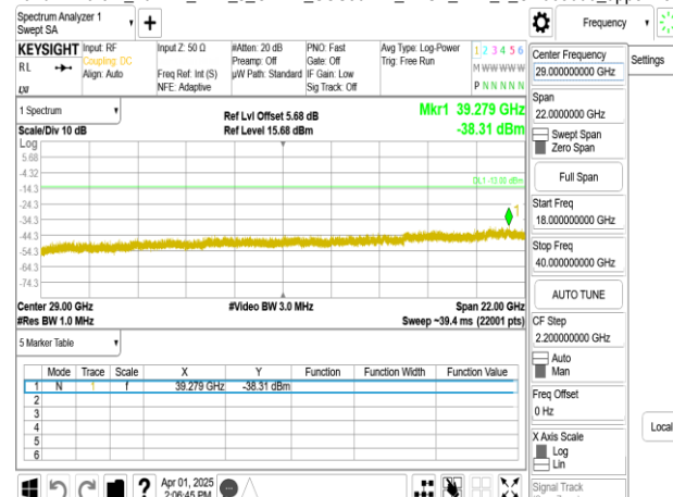
Band77-Part27_70MHz_DFT_s_OFDM_SCS30kHz_BPSK_RB1_1_CH663000_upper 18G
