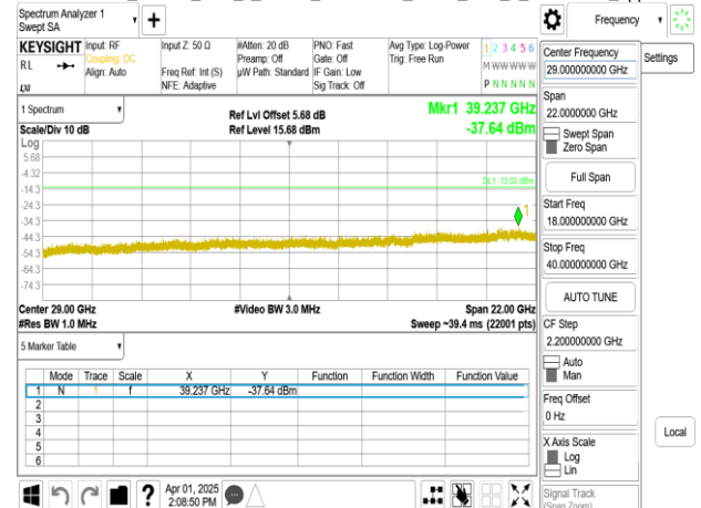
Band77-Part27_80MHz_DFT_s_OFDM_SCS30kHz_BPSK_RB1_1_CH626666_upper 18G
