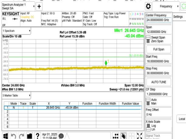
Band7_15MHz_DFT_s_OFDM_SCS15kHz_BPSK_RB1_1_CH512500_upper 18G
