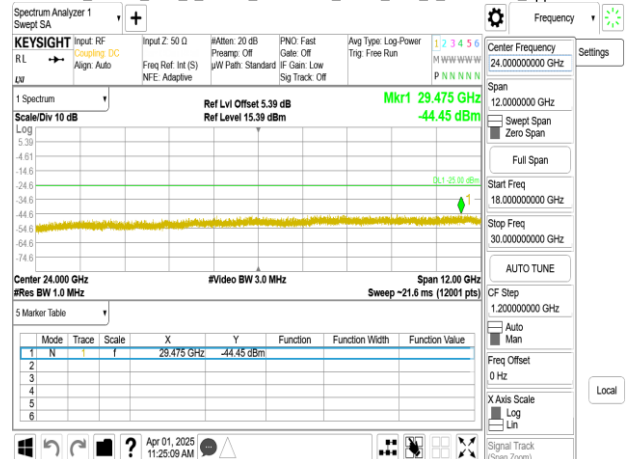
Band7_30MHz_DFT_s_OFDM_SCS30kHz_BPSK_RB1_1_CH511000_upper 18G
