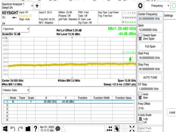
Band7_15MHz_DFT_s_OFDM_SCS15kHz_BPSK_RB1_1_CH507000_upper 18G
