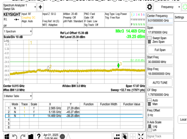
Band7_5MHz_DFT_s_OFDM_SCS15kHz_BPSK_RB1_1_CH513500_below 18G
