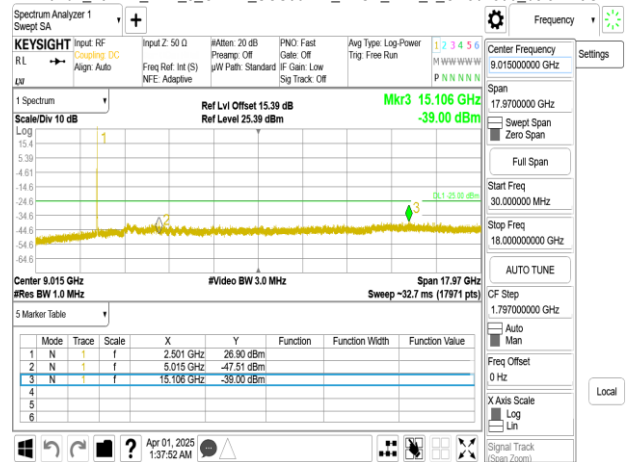
Band7_15MHz_DFT_s_OFDM_SCS30kHz_BPSK_RB1_1_CH507000_below 18G
