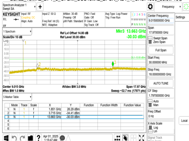
Band2_15MHz_DFT_s_OFDM_SCS15kHz_BPSK_RB1_1_CH376000_below 18G
