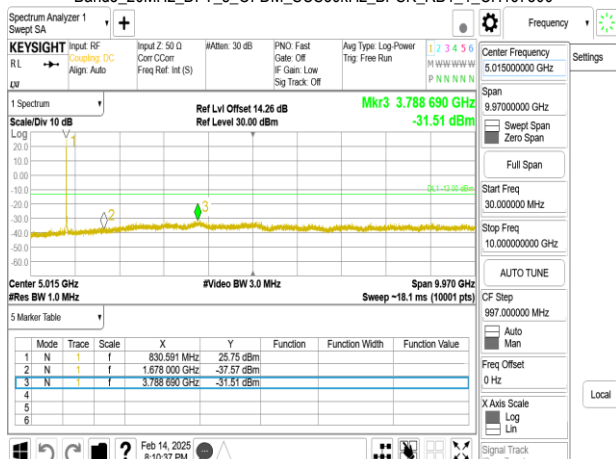
Band5_20MHz_DFT_s_OFDM_SCS30kHz_BPSK_RB1_1_CH167800
