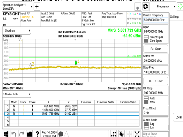
Band5_20MHz_DFT_s_OFDM_SCS30kHz_BPSK_RB1_1_CH167300
