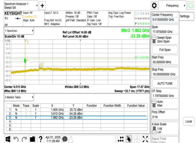
Band2_5MHz_DFT_s_OFDM_SCS15kHz_BPSK_RB1_1_CH381500_below 18G
