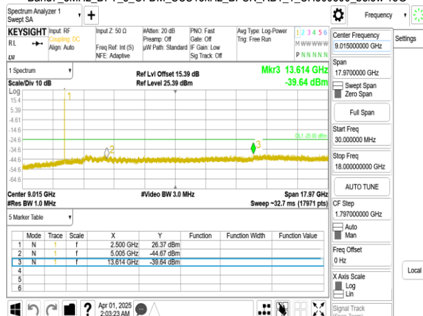
Band7_5MHz_DFT_s_OFDM_SCS15kHz_BPSK_RB1_1_CH507000_below 18G
