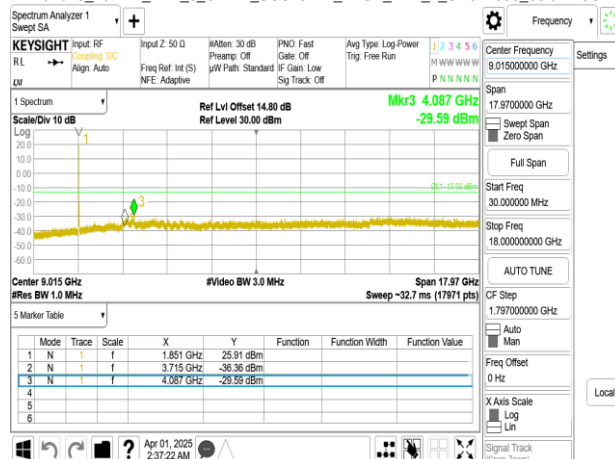
Band25_15MHz_DFT_s_OFDM_SCS15kHz_BPSK_RB1_1_CH371500_below 18G
