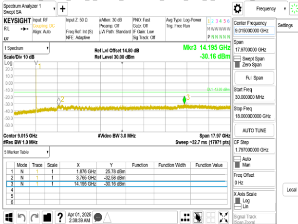
Band25_15MHz_DFT_s_OFDM_SCS15kHz_BPSK_RB1_1_CH381500_below 18G
