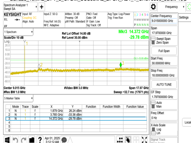
Band25_10MHz_DFT_s_OFDM_SCS30kHz_BPSK_RB1_1_CH382000_below 18G
