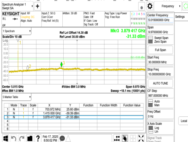
Band12_10MHz_DFT_s_OFDM_SCS30kHz_BPSK_RB1_1.CH142200
