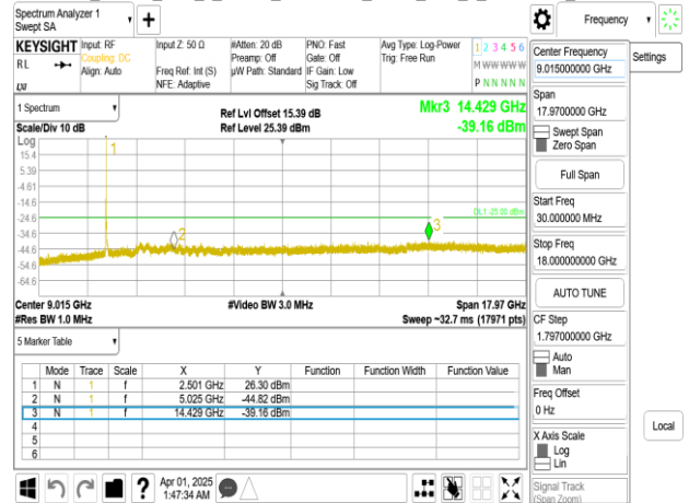
Band7_25MHz_DFT_s_OFDM_SCS30kHz_BPSK_RB1_1_CH507000_below 18G
