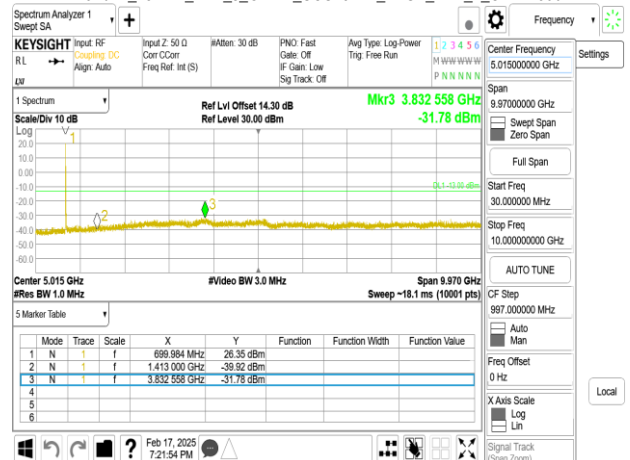
Band12_15MHz_DFT_s_OFDM_SCS15kHz_BPSK_RB1_1.CH141500
