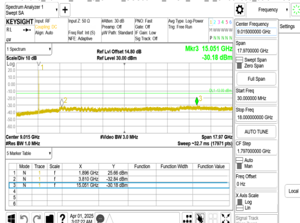
Band25_25MHz_DFT_s_OFDM_SCS15kHz_BPSK_RB1_1_CH372500_below 18G
