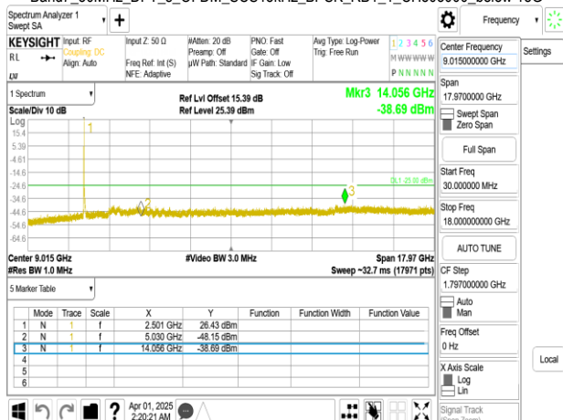
Band7_30MHz_DFT_s_OFDM_SCS15kHz_BPSK_RB1_1_CH507000_below 18G
