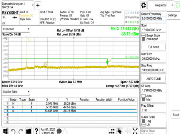
Band7_25MHz_DFT_s_OFDM_SCS15kHz_BPSK_RB1_1_CH511500_below 18G
