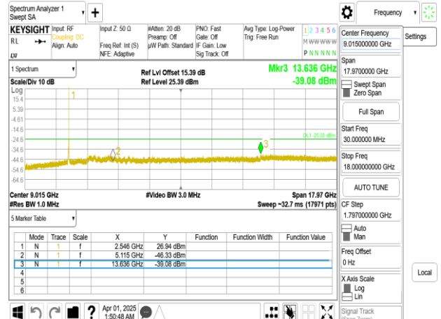
Band7_25MHz_DFT_s_OFDM_SCS30kHz_BPSK_RB1_1_CH511500_below 18G
