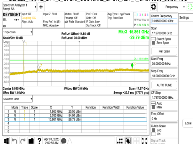
Band25_40MHz_DFT_s_OFDM_SCS15kHz_BPSK_RB1_1_CH379000_below 18G
