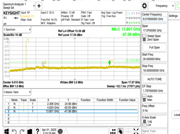
Band30_10MHz_DFT_s_OFDM_SCS30kHz_BPSK_RB1_1_CH462000_below 18G
