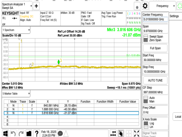
Band26_15MHz_DFT_s_OFDM_SCS15kHz_BPSK_RB1_1_CH166300
