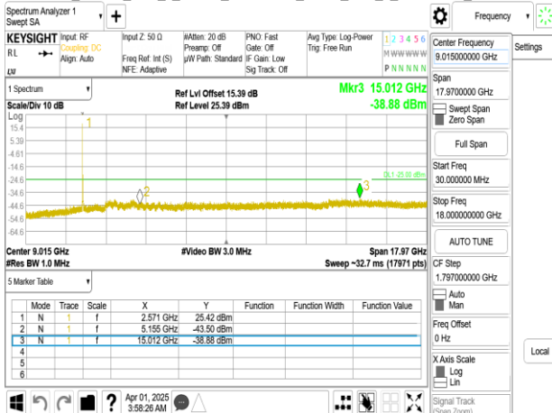
Band38_15MHz_DFT_s_OFDM_SCS30kHz_BPSK_RB1_1_CH519000_below 18G
