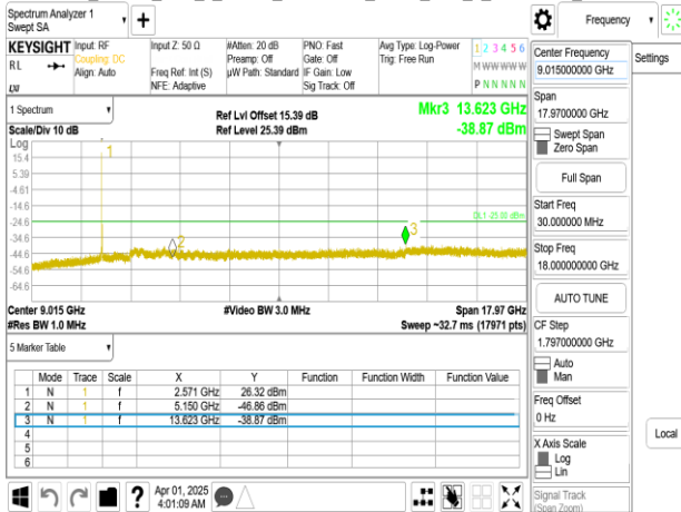
Band38_10MHz_DFT_s_OFDM_SCS30kHz_BPSK_RB1_1_CH519000_below 18G
