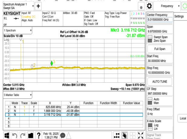
Band26_20MHz_DFT_s_OFDM_SCS30kHz_BPSK_RB1_1_CH167300
