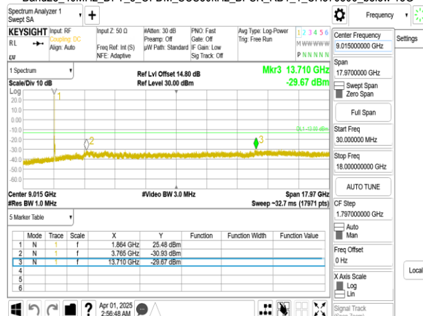
Band25_40MHz_DFT_s_OFDM_SCS30kHz_BPSK_RB1_1_CH379000_below 18G
