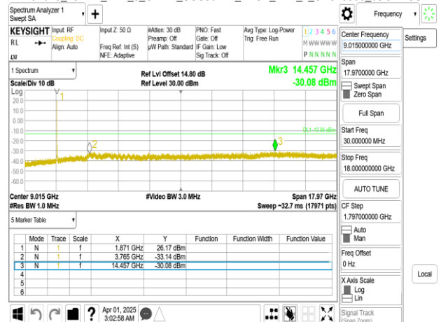
Band25_25MHz_DFT_s_OFDM_SCS30kHz_BPSK_RB1_1_CH380500_below 18G
