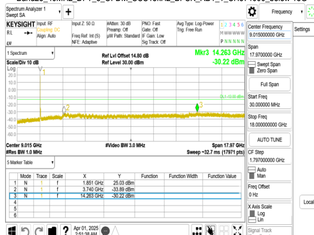
Band25_40MHz_DFT_s_OFDM_SCS15kHz_BPSK_RB1_1_CH374000_below 18G
