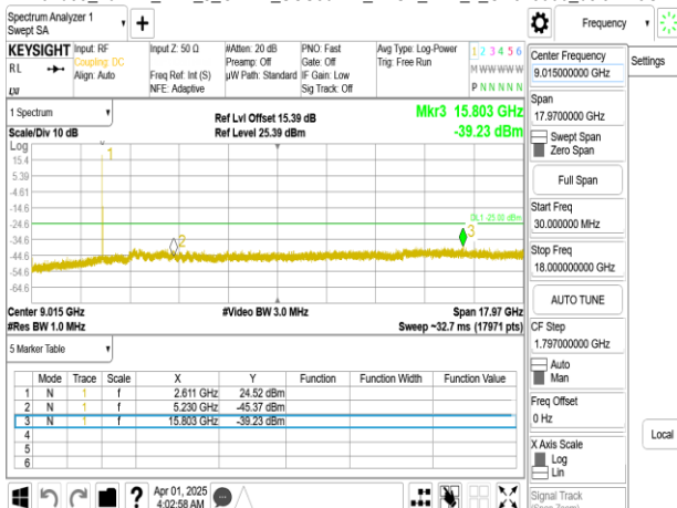
Band38_10MHz_DFT_s_OFDM_SCS30kHz_BPSK_RB1_1_CH523000_below 18G
