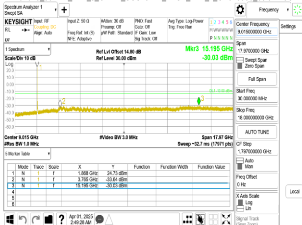
Band25_30MHz_DFT_s_OFDM_SCS15kHz_BPSK_RB1_1_CH380000_below 18G
