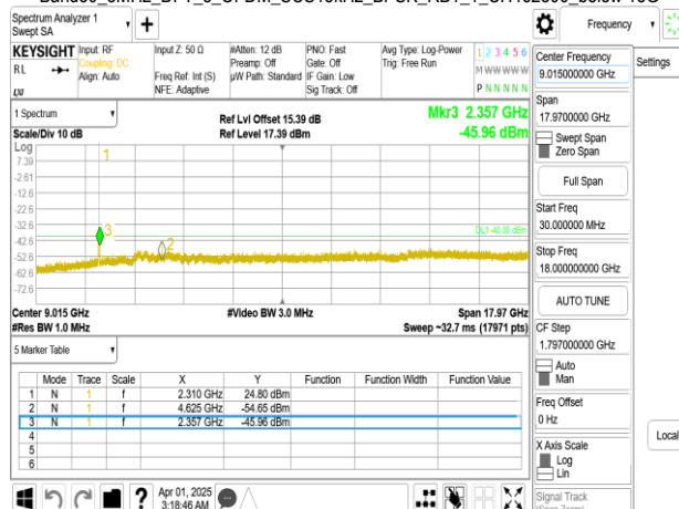
Band30_10MHz_DFT_s_OFDM_SCS15kHz_BPSK_RB1_1_CH462000_below 18G
