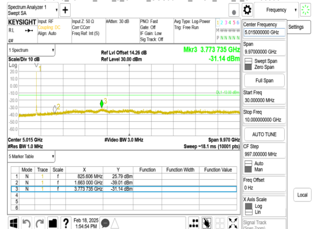
Band26_15MHz_DFT_s_OFDM_SCS30kHz_BPSK_RB1_1_CH167300
