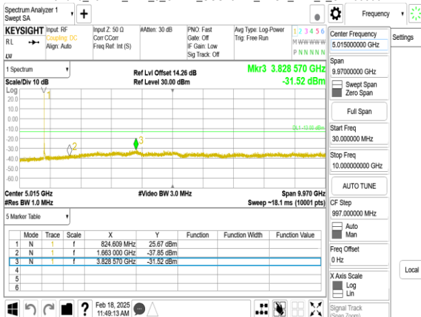
Band26_15MHz_DFT_s_OFDM_SCS15kHz_BPSK_RB1_1_CH167300
