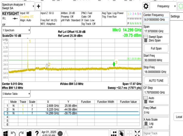
Band38_15MHz_DFT_s_OFDM_SCS30kHz_BPSK_RB1_1_CH522500_below 18G
