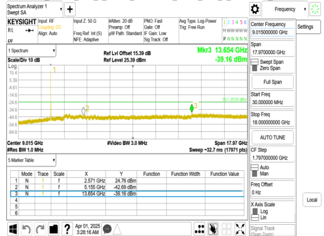
Band38_15MHz_DFT_s_OFDM_SCS15kHz_BPSK_RB1_1_CH519000_below 18G
