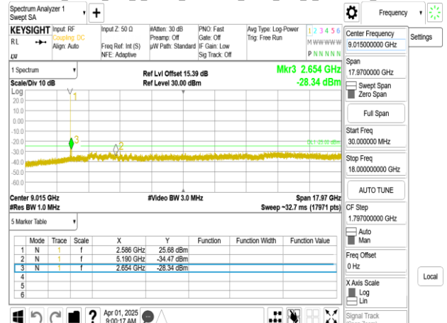
Band38_20MHz_DFT_s_OFDM_SCS15kHz_BPSK_RB1_1_CH522000_below 18G
