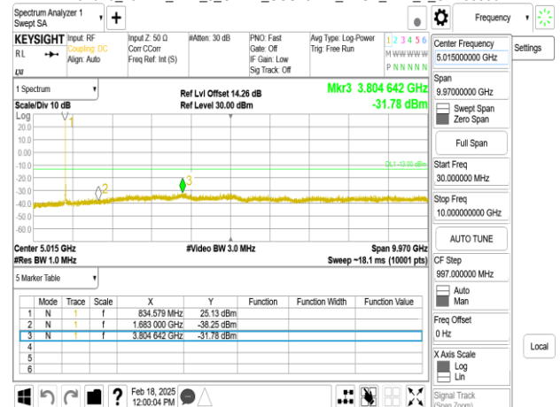
Band26_15MHz_DFT_s_OFDM_SCS30kHz_BPSK_RB1_1_CH166300
