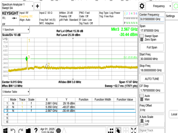
Band41_30MHz_DFT_s_OFDM_SCS15kHz_BPSK_RB1_1_CH534996_below 18G
