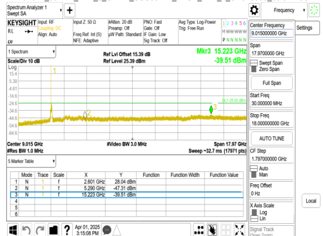
Band41_100MHz_DFT_s_OFDM_SCS30kHz_BPSK_RB1_1_CH509202_below 18G
