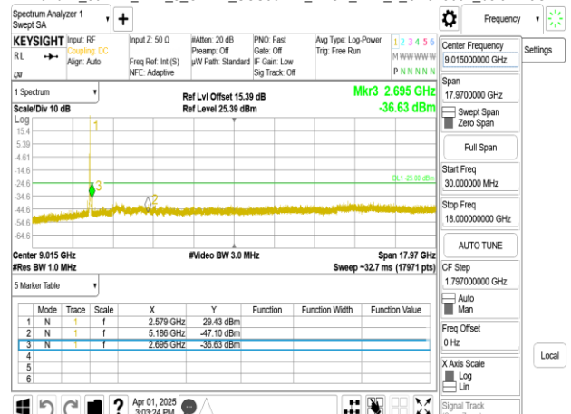
Band41_30MHz_DFT_s_OFDM_SCS30kHz_BPSK_RB1_1_CH518604_below 18G
