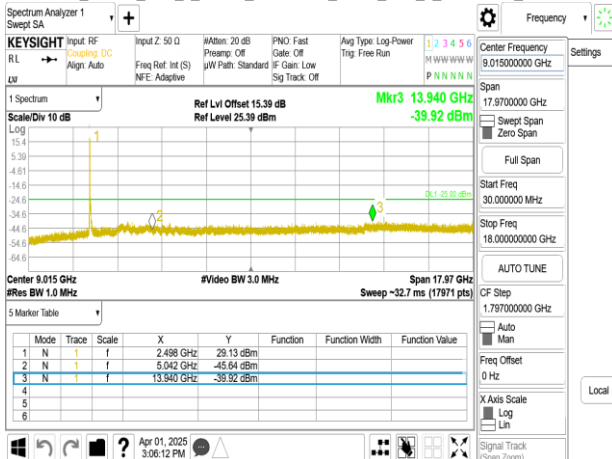
Band41_50MHz_DFT_s_OFDM_SCS30kHz_BPSK_RB1_1_CH505002_below 18G
