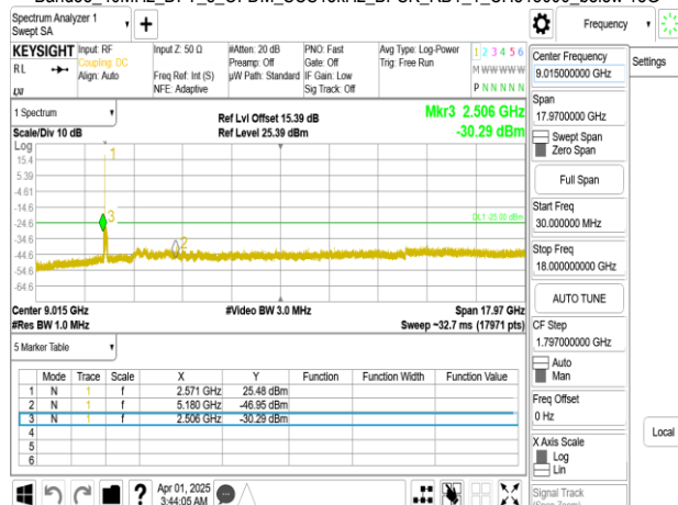
Band38_40MHz_DFT_s_OFDM_SCS15kHz_BPSK_RB1_1_CH519000_below 18G
