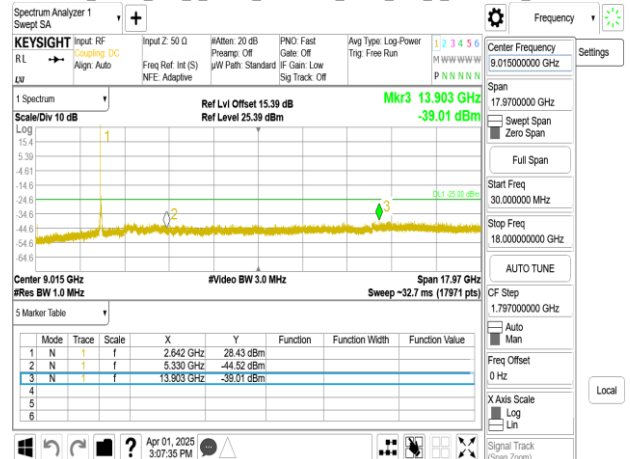
Band41_60MHz_DFT_s_OFDM_SCS30kHz_BPSK_RB1_1_CH505200_below 18G
