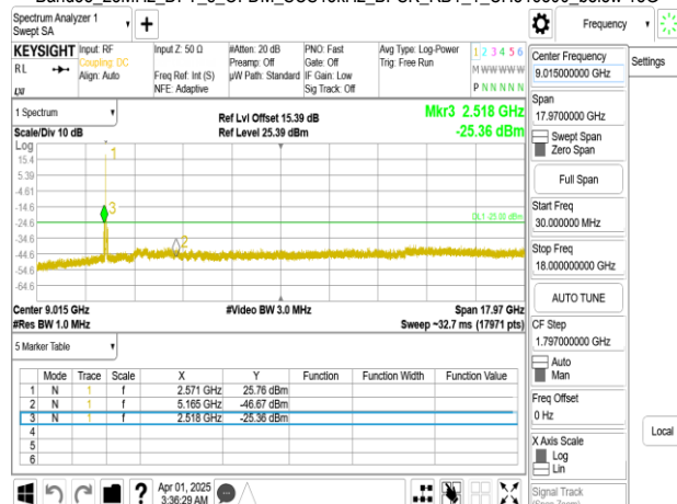
Band38_25MHz_DFT_s_OFDM_SCS15kHz_BPSK_RB1_1_CH519000_below 18G
