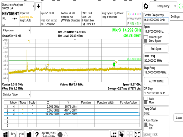
Band41_50MHz_DFT_s_OFDM_SCS30kHz_BPSK_RB1_1_CH505002_below 18G
