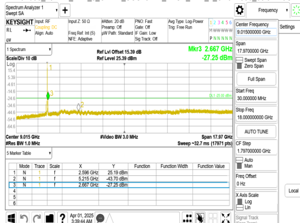
Band38_25MHz_DFT_s_OFDM_SCS15kHz_BPSK_RB1_1_CH521500_below 18G
