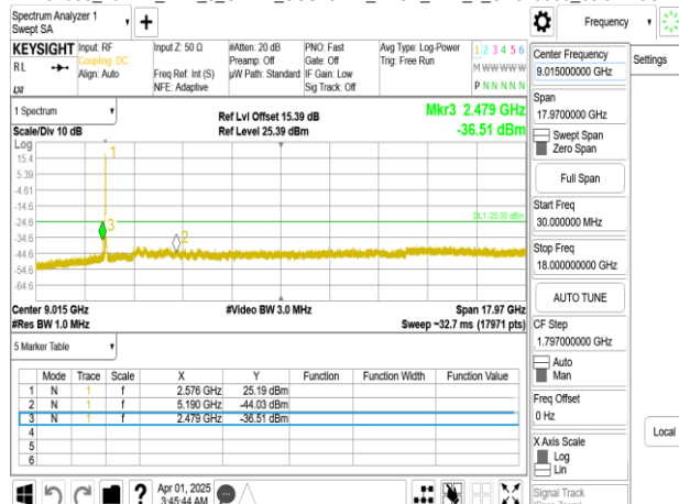
Band38_40MHz_DFT_s_OFDM_SCS15kHz_BPSK_RB1_1_CH520000_below 18G
