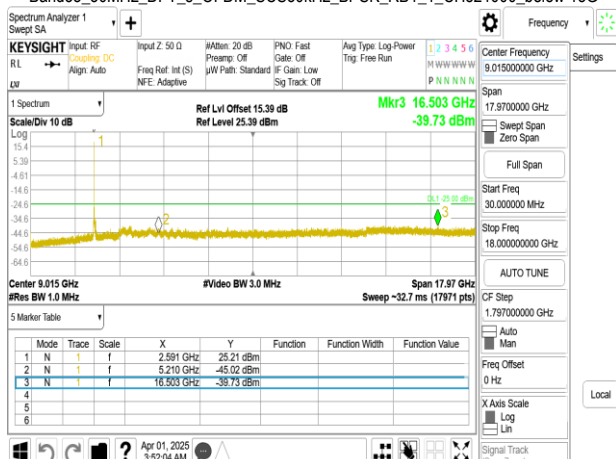
Band38_30MHz_DFT_s_OFDM_SCS30kHz_BPSK_RB1_1_CH521000_below 18G
