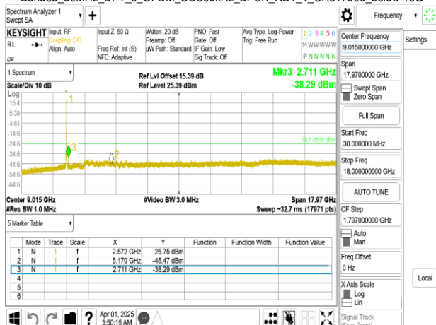
Band38_30MHz_DFT_s_OFDM_SCS30kHz_BPSK_RB1_1_CH519000_below 18G
