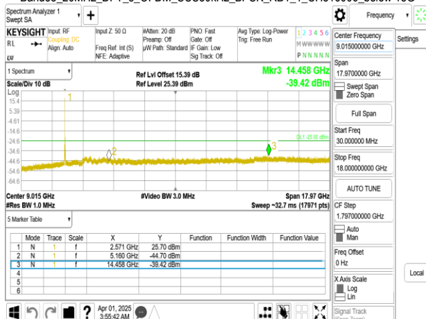
Band38_20MHz_DFT_s_OFDM_SCS30kHz_BPSK_RB1_1_CH519000_below 18G
