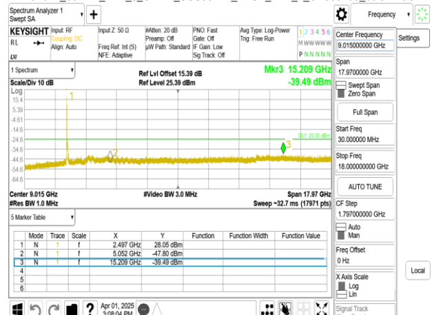
Band41_60MHz_DFT_s_OFDM_SCS30kHz_BPSK_RB1_1_CH505200_below 18G
