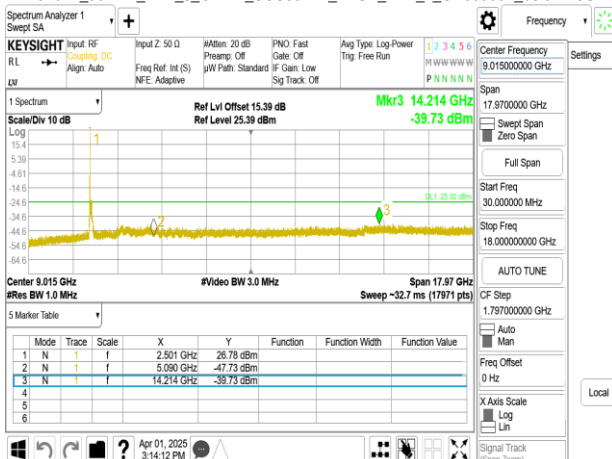
Band41_90MHz_DFT_s_OFDM_SCS30kHz_BPSK_RB1_1_CH509004_below 18G
