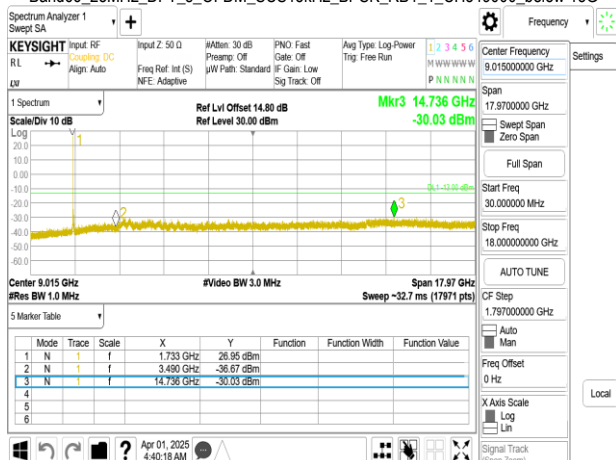
Band66_25MHz_DFT_s_OFDM_SCS15kHz_BPSK_RB1_1_CH353500
