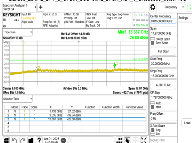
Band66_25MHz_DFT_s_OFDM_SCS15kHz_BPSK_RB1_1_CH353500_below 18G
