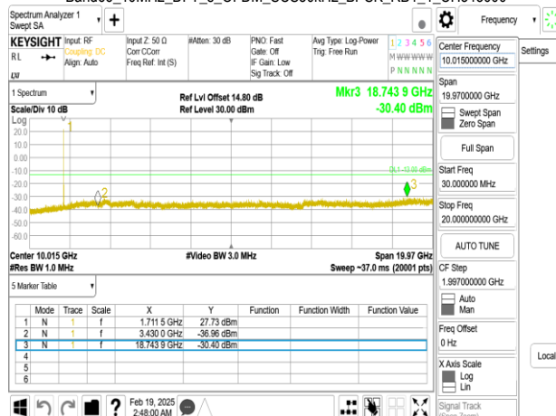
Band66_10MHz_DFT_s_OFDM_SCS30kHz_BPSK_RB1_1_CH343000_below 18G
