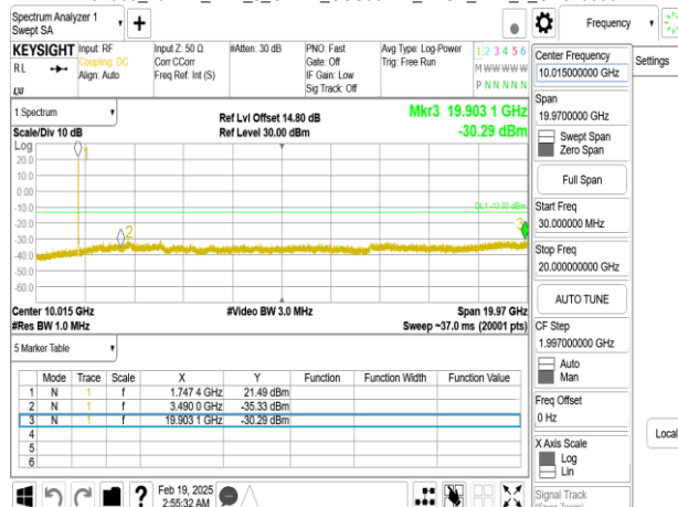
Band66_10MHz_DFT_s_OFDM_SCS30kHz_BPSK_RB1_1_CH349000
