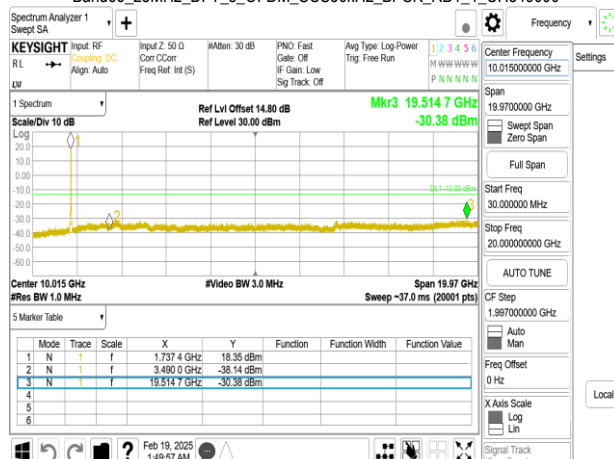
Band66_25MHz_DFT_s_OFDM_SCS30kHz_BPSK_RB1_1_CH349000
