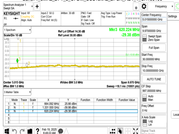
Band71_5MHz_DFT_s_OFDM_SCS15kHz_BPSK_RB1_1_CH136100
