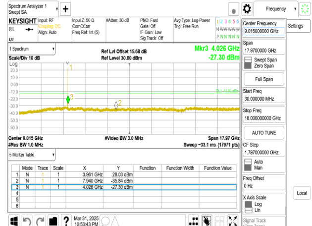
Band77-Part27_20MHz_DFT_s_OFDM_SCS15kHz_BPSK_RB1_1_CH646666_below 18G
