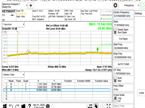
Band66_40MHz_DFT_s_OFDM_SCS30kHz_BPSK_RB1_1_CH352000_below 18G
