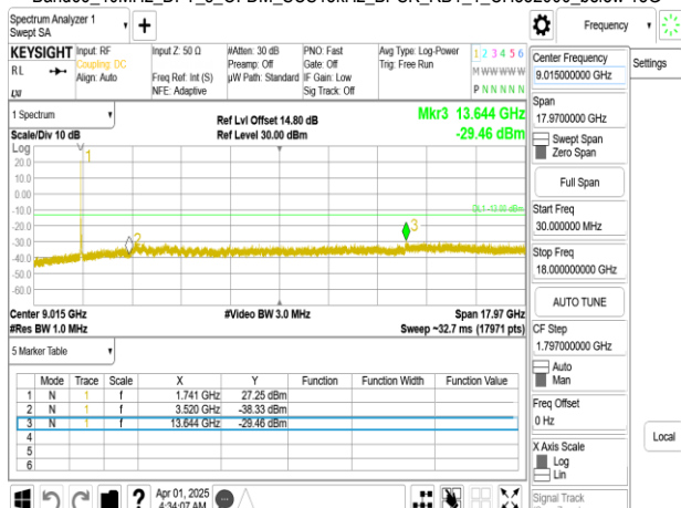
Band66_40MHz_DFT_s_OFDM_SCS15kHz_BPSK_RB1_1_CH352000_below 18G
