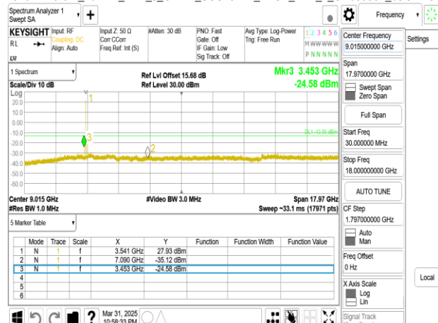
Band77-Part27_10MHz_DFT_s_OFDM_SCS15kHz_BPSK_RB1_1_CH636332_below 18G
