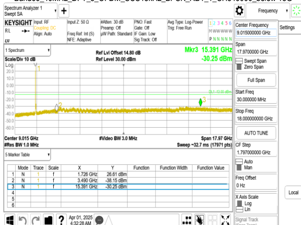
Band66_40MHz_DFT_s_OFDM_SCS15kHz_BPSK_RB1_1_CH352000
