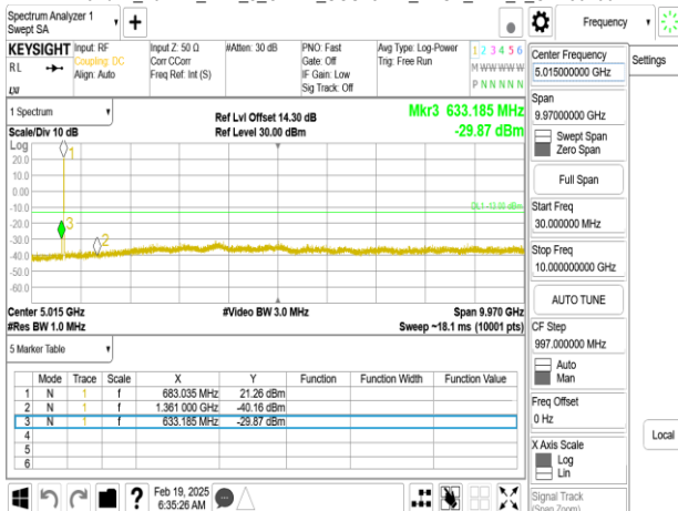
Band71_10MHz_DFT_s_OFDM_SCS15kHz_BPSK_RB1_1_CH138600
