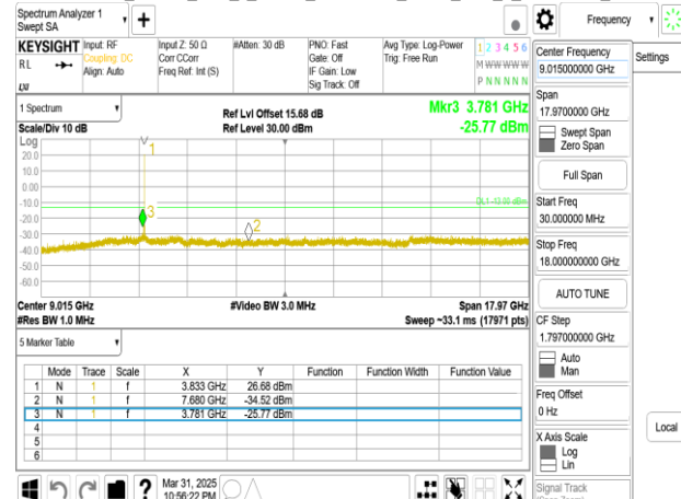
Band77-Part27_15MHz_DFT_s_OFDM_SCS15kHz_BPSK_RB1_1_CH664832_below 18G
