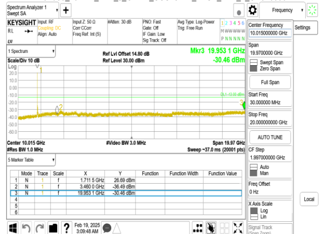
Band66_40MHz_DFT_s_OFDM_SCS15kHz_BPSK_RB1_1_CH346000_below 18G
