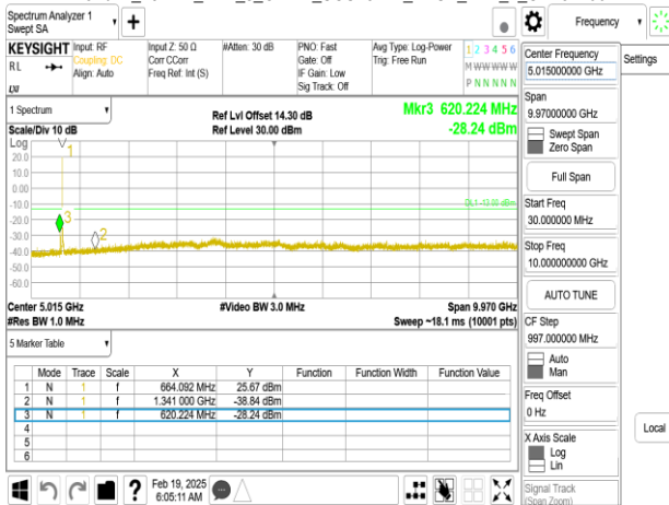
Band71_15MHz_DFT_s_OFDM_SCS15kHz_BPSK_RB1_1_CH136100
