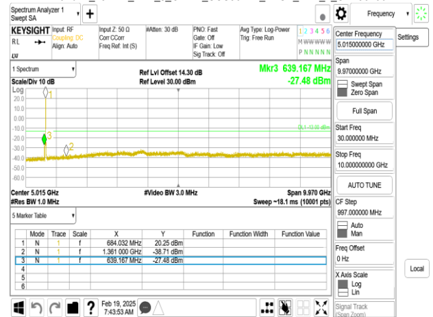
Band71_15MHz_DFT_s_OFDM_SCS30kHz_BPSK_RB1_1_CH138100
