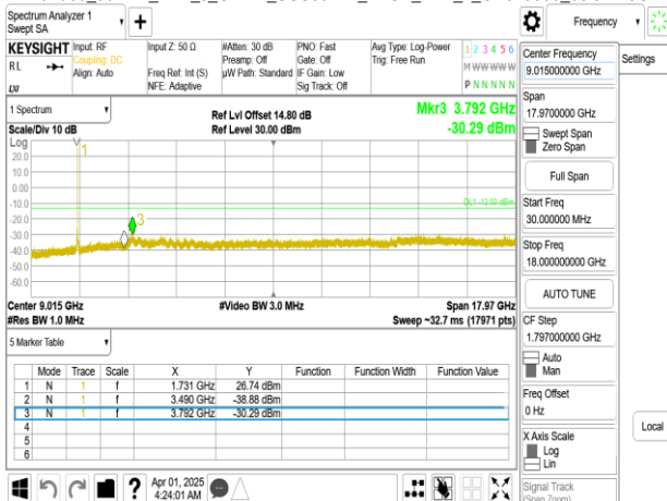
Band66_30MHz_DFT_s_OFDM_SCS30kHz_BPSK_RB1_1_CH353000
