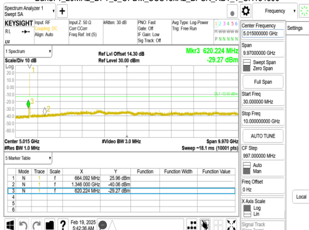
Band71_20MHz_DFT_s_OFDM_SCS15kHz_BPSK_RB1_1_CH136100
