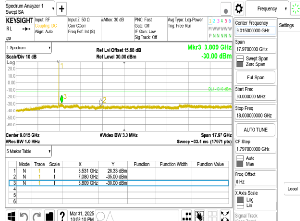
Band77-Part27_20MHz_DFT_s_OFDM_SCS15kHz_BPSK_RB1_1_CH636000_below 18G
