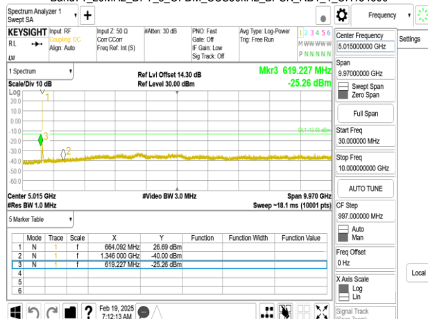
Band71_20MHz_DFT_s_OFDM_SCS30kHz_BPSK_RB1_1_CH136100
