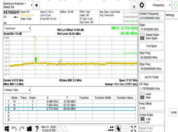
Band77-Part27_10MHz_DFT_s_OFDM_SCS30kHz_BPSK_RB1_1_CH636332_below 18G
