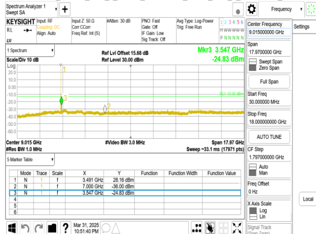
Band77-Part27_20MHz_DFT_s_OFDM_SCS15kHz_BPSK_RB1_1_CH636000_below 18G
