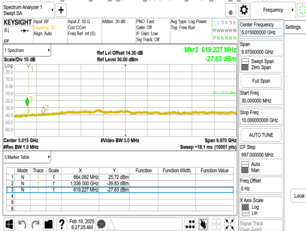
Band71_10MHz_DFT_s_OFDM_SCS15kHz_BPSK_RB1_1_CH136100
