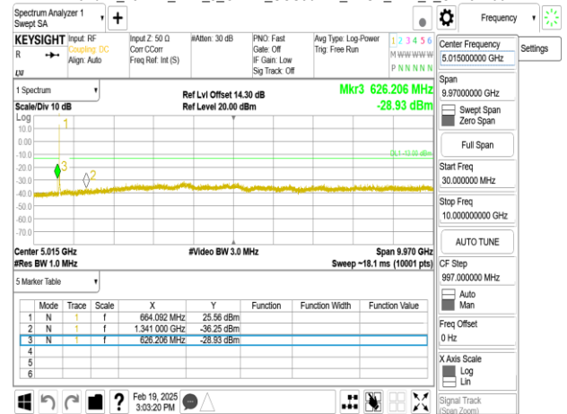
Band71_15MHz_DFT_s_OFDM_SCS30kHz_BPSK_RB1_1_CH136100
