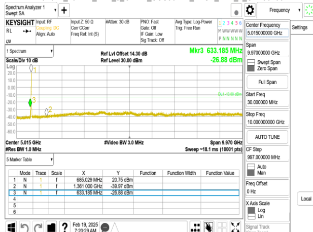
Band71_20MHz_DFT_s_OFDM_SCS30kHz_BPSK_RB1_1_CH137600
