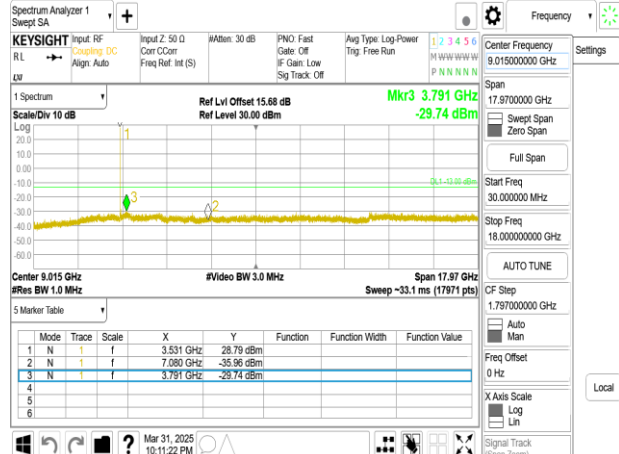
Band77-Part27_20MHz_DFT_s_OFDM_SCS30kHz_BPSK_RB1_1_CH636000_below 18G
