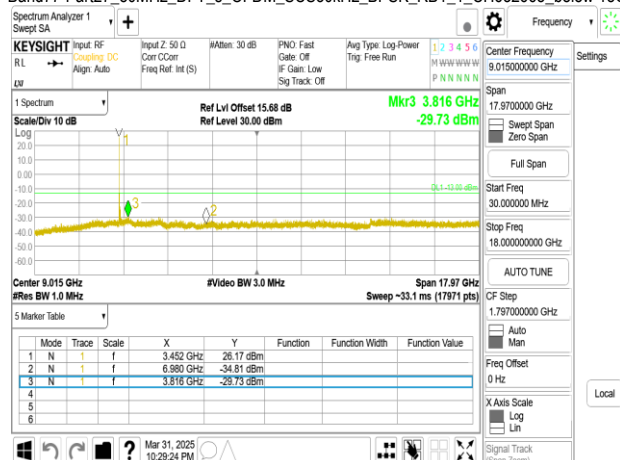
Band77-Part27 80MHz DFT s OFDM SCS30kHz BPSK RB1 1 CH633334 below 18G
