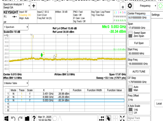
Band77-Part27 90MHz DFT s OFDM SCS30kHz BPSK RB1 1 CH633334 below 18G
