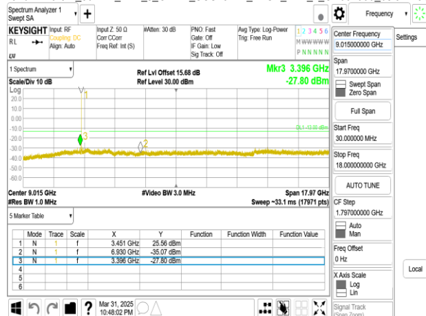
Band77-Part27_30MHz_DFT_s_OFDM_SCS15kHz_BPSK_RB1_1_CH633334_below 18G
