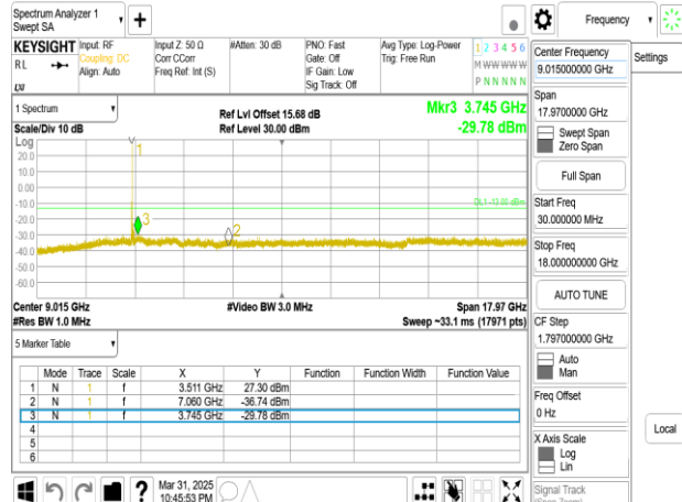
Band77-Part27_40MHz_DFT_s_OFDM_SCS15kHz_BPSK_RB1_1_CH635332_below 18G
