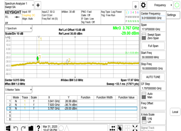
Band77-Part27_40MHz_DFT_s_OFDM_SCS15kHz_BPSK_RB1_1_CH664000_below 18G
