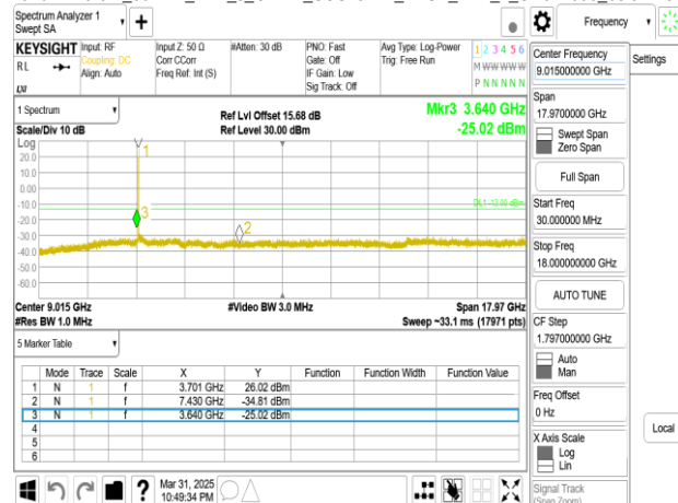
Band77-Part27_30MHz_DFT_s_OFDM_SCS15kHz_BPSK_RB1_1_CH656000_below 18G
