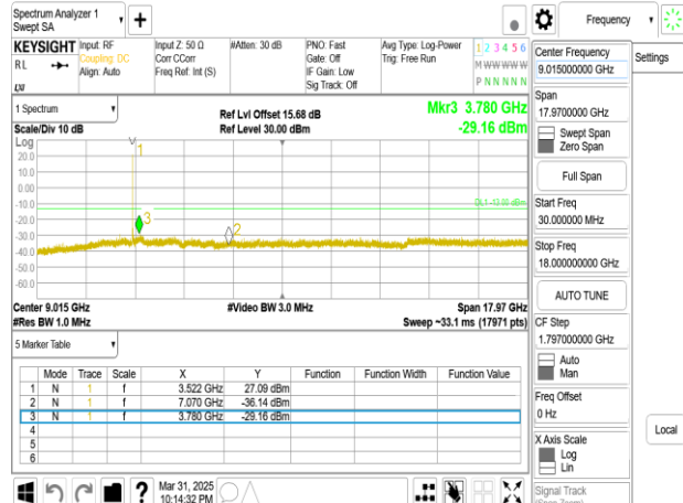
Band77-Part27_30MHz_DFT_s_OFDM_SCS30kHz_BPSK_RB1_1_CH635666_below 18G
