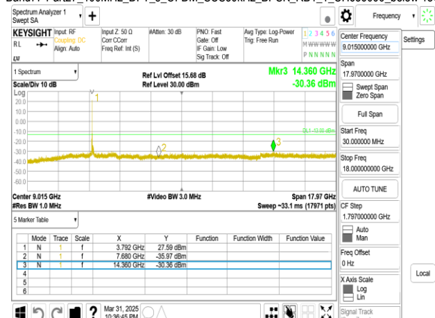
Band77-Part27 100MHz DFT s OFDM SCS30kHz BPSK RB1 1 CH656000 below 18G
