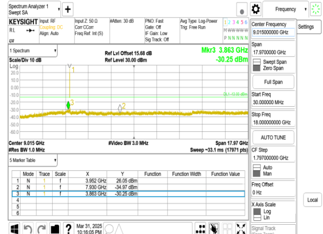
Band77-Part27_30MHz_DFT_s_OFDM_SCS30kHz_BPSK_RB1_1_CH664332_below 18G
