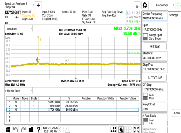
Band77-Part27_50MHz_DFT_s_OFDM_SCS30kHz_BPSK_RB1_1_CH636666_below 18G
