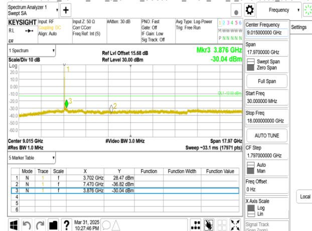
Band77-Part27_70MHz_DFT_s_OFDM_SCS30kHz_BPSK_RB1_1_CH656000_below 18G
