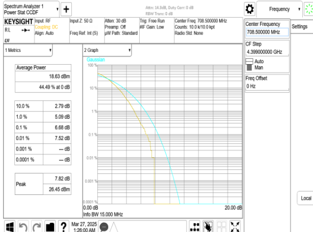
Band12_15MHz_DFT_s_OFDM_SCS15kHz_256QAM_RB75_0_CH141700
