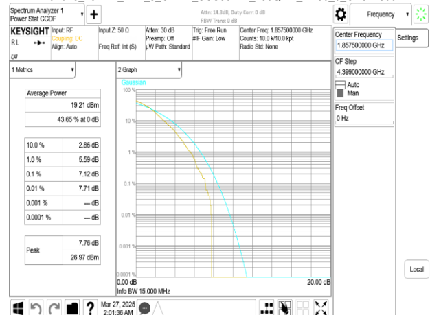
Band25_15MHz_DFT_s_OFDM_SCS30kHz_256QAM_RB36_0_CH371500
