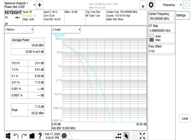
Band14_10MHz_DFT_s_OFDM_SCS30kHz_256QAM_RB24_0_CH158600
