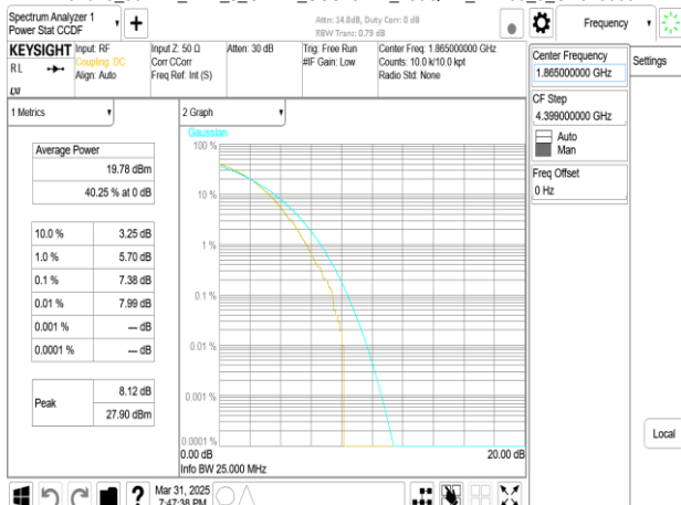
Band25_30MHz_DFT_s_OFDM_SCS15kHz_256QAM_RB160_0_CH373000
