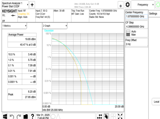
Band25_40MHz_DFT_s_OFDM_SCS15kHz_256QAM_RB216_0_CH374000
