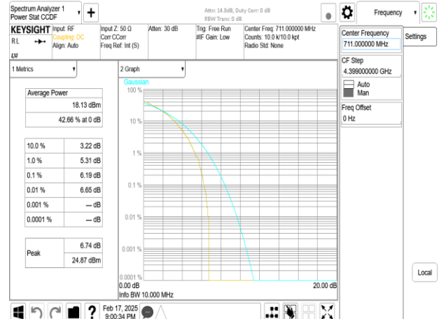
Band12_10MHz_DFT_s_OFDM_SCS30kHz_256QAM_RB24_0_CH142200
