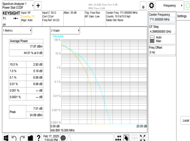
Band12_10MHz_DFT_s_OFDM_SCS15kHz_256QAM_RB50_0_CH142200
