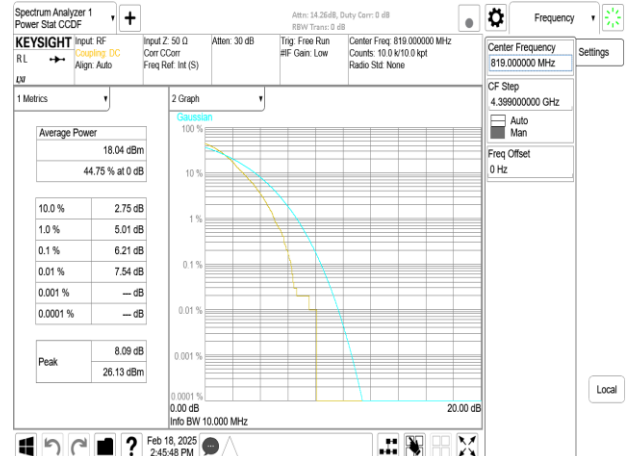
Band26-Part90s_10MHz_DFT_s_OFDM_SCS15kHz_256QAM_RB50_0_CH163800
