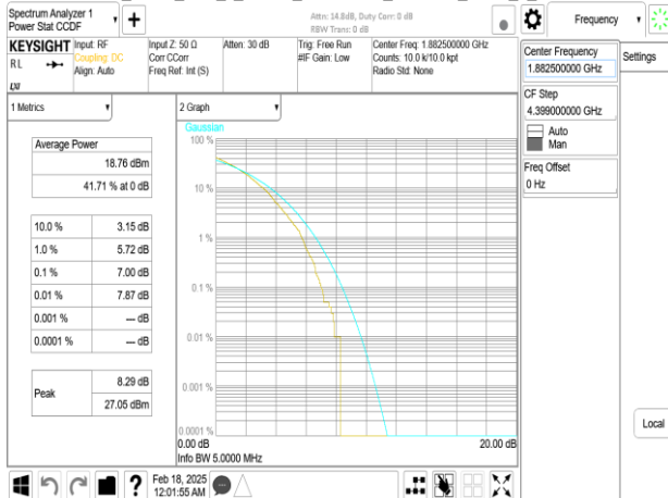
Band25_5MHz_DFT_s_OFDM_SCS15kHz_256QAM_RB25_0_CH382500
