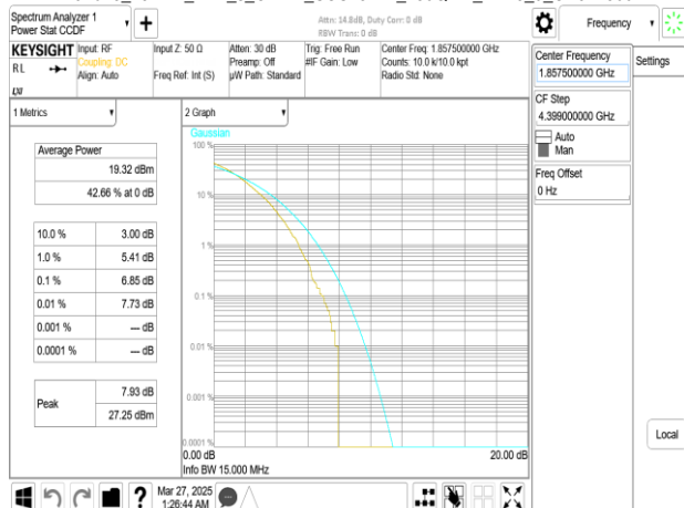
Band25_15MHz_DFT_s_OFDM_SCS15kHz_256QAM_RB75_0_CH371500
