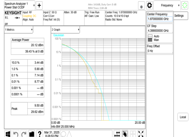
Band25_40MHz_DFT_s_OFDM_SCS30kHz_256QAM_RB100_0_CH374000
