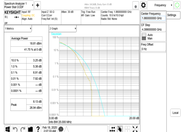
Band25_20MHz_DFT_s_OFDM_SCS30kHz_256QAM_RB50_0_CH372000
