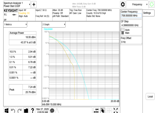
Band12_15MHz_DFT_s_OFDM_SCS30kHz_256QAM_RB36_0_CH141700
