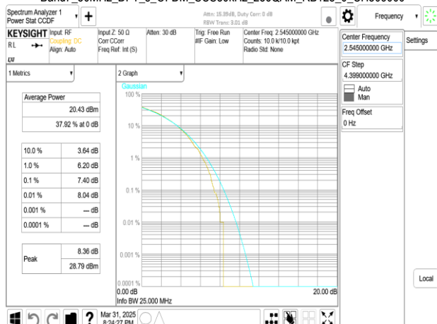
Band7_50MHz_DFT_s_OFDM_SCS30kHz_256QAM_RB128_0_CH509000
