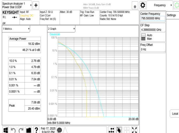
Band14_5MHz_DFT_s_OFDM_SCS15kHz_256QAM_RB25_0_CH159100
