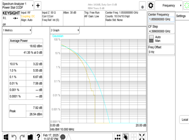
Band25_10MHz_DFT_s_OFDM_SCS15kHz_256QAM_RB50_0_CH371000
