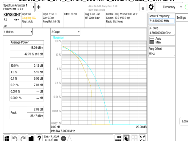
Band12_5MHz_DFT_s_OFDM_SCS15kHz_256QAM_RB25_0_CH142700
