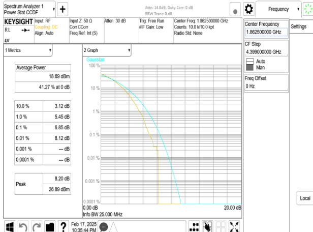
Band25_25MHz_DFT_s_OFDM_SCS15kHz_256QAM_RB128_0_CH372500
