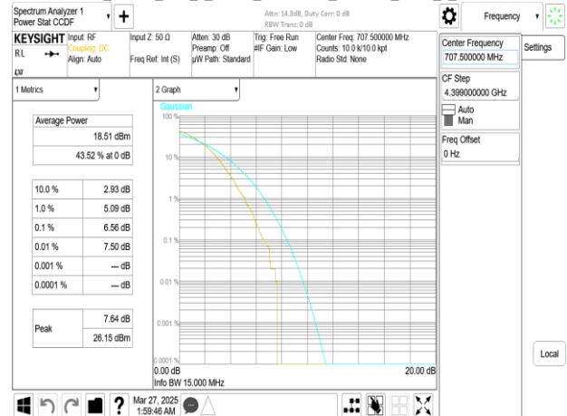
Band12_15MHz_DFT_s_OFDM_SCS30kHz_256QAM_RB36_0_CH141700
