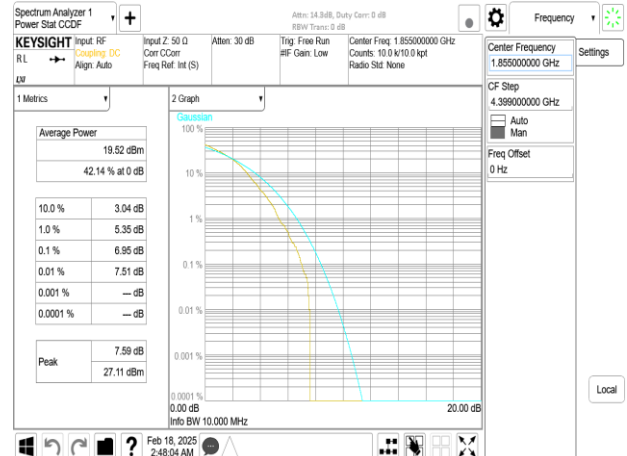
Band25_10MHz_DFT_s_OFDM_SCS30kHz_256QAM_RB24_0_CH371000
