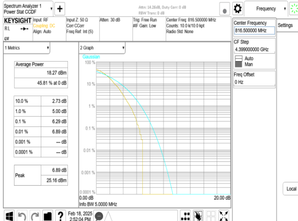
Band26-Part90s_5MHz_DFT_s_OFDM_SCS15kHz_256QAM_RB25_0_CH163300
