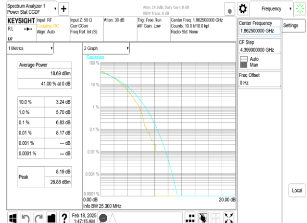
Band25_25MHz_DFT_s_OFDM_SCS30kHz_256QAM_RB64_0_CH372500
