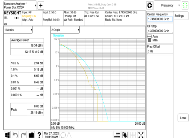
Band66_15MHz_DFT_s_OFDM_SCS15kHz_256QAM_RB75_0_CH349000
