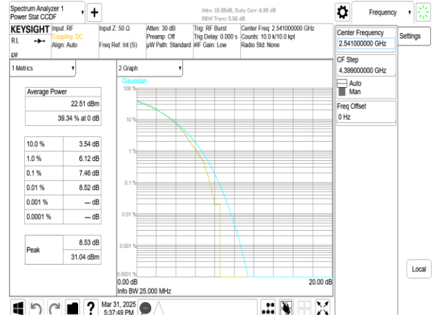
Band41_90MHz_DFT_s_OFDM_SCS30kHz_256QAM_RB243_0_CH508200
