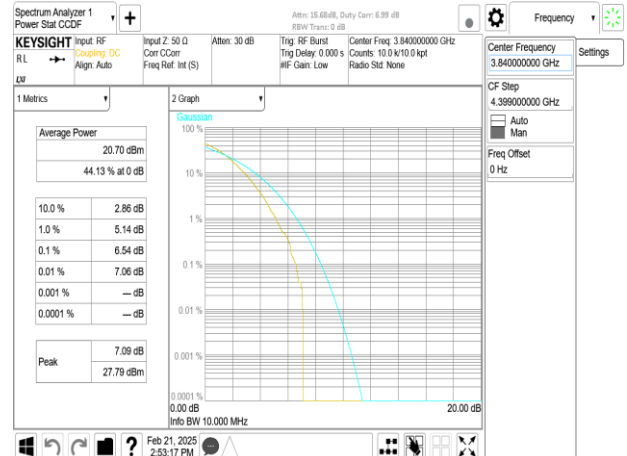
Band77-Part27_10MHz_DFT_s_OFDM_SCS15kHz_256QAM_RB50_0_CH656000
