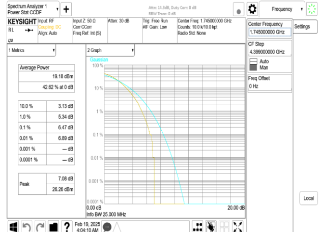
Band66_25MHz_DFT_s_OFDM_SCS15kHz_256QAM_RB128_0_CH349000
