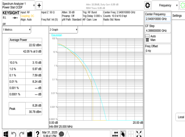
Band41_80MHz_DFT_s_OFDM_SCS30kHz_256QAM_RB216_0_CH508002
