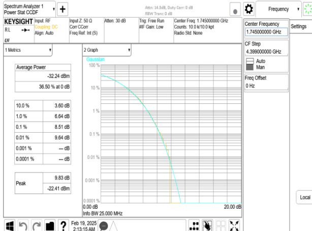
Band66_20MHz_DFT_s_OFDM_SCS30kHz_256QAM_RB50_0_CH349000
