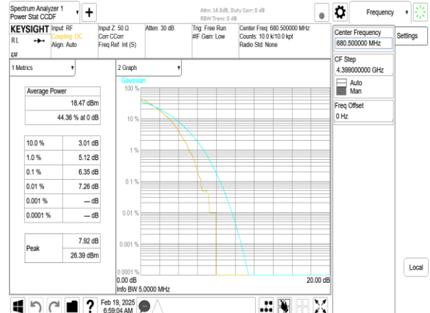
Band71_5MHz_DFT_s_OFDM_SCS15kHz_256QAM_RB25_0_CH136100
