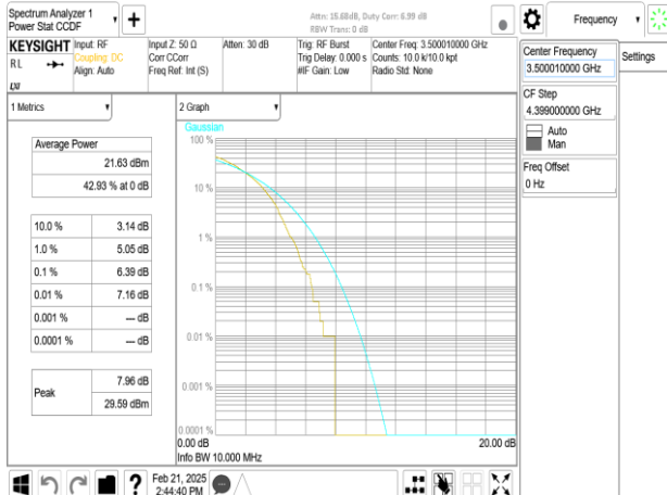
Band77-Part27_10MHz_DFT_s_OFDM_SCS15kHz_256QAM_RB50_0_CH633334
