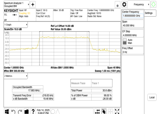
Band2_20MHz_DFT_s_OFDM_SCS30kHz_QPSK_RB50_0_CH380000
