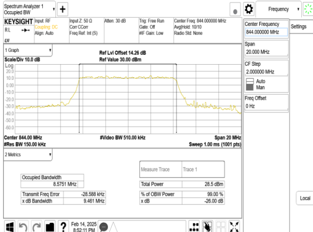
Band5_10MHz_DFT_s_OFDM_SCS30kHz_64QAM_RB24_0_CH168800
