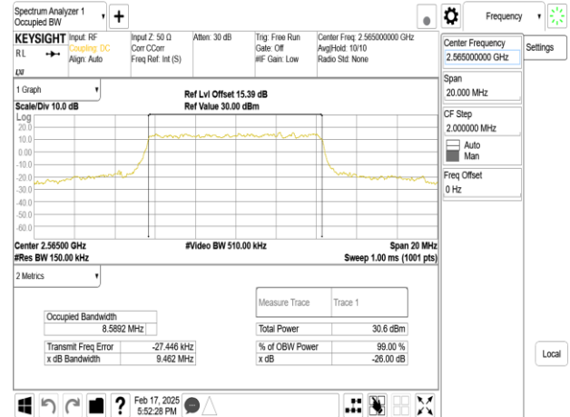
Band7_10MHz_DFT_s_OFDM_SCS30kHz_QPSK_RB24_0_CH513000
