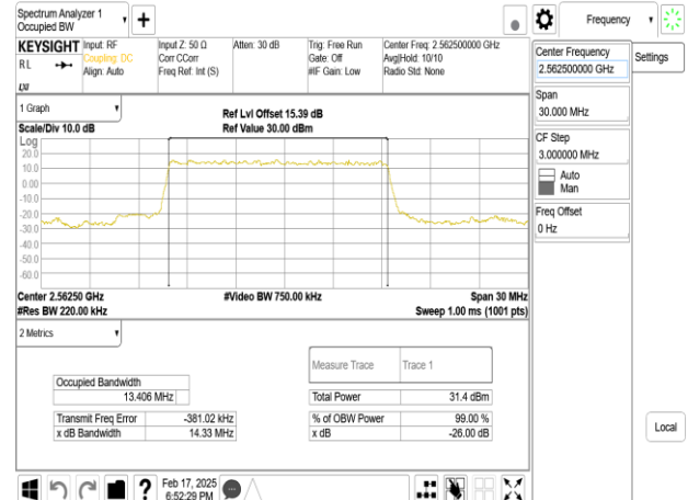
Band7_15MHz_DFT_s_OFDM_SCS15kHz_BPSK_RB75_0_CH512500
