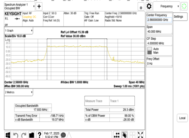
Band7_20MHz_DFT_s_OFDM_SCS30kHz_64QAM_RB50_0_CH512000
