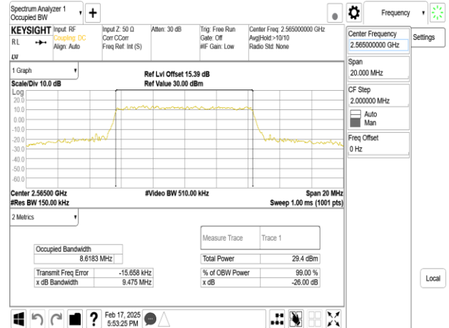
Band7_10MHz_DFT_s_OFDM_SCS30kHz_64QAM_RB24_0_CH513000
