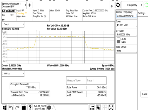
Band7_20MHz_DFT_s_OFDM_SCS30kHz_16QAM_RB50_0_CH512000
