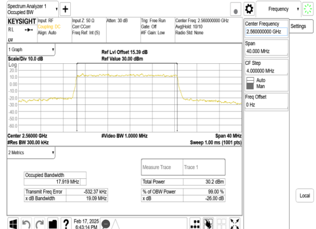
Band7_20MHz_DFT_s_OFDM_SCS15kHz_16QAM_RB100_0_CH512000
