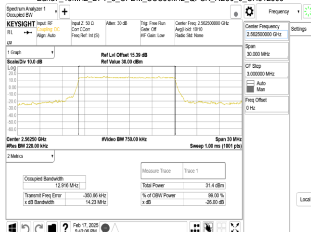
Band7_15MHz_DFT_s_OFDM_SCS30kHz_QPSK_RB36_0_CH512500
