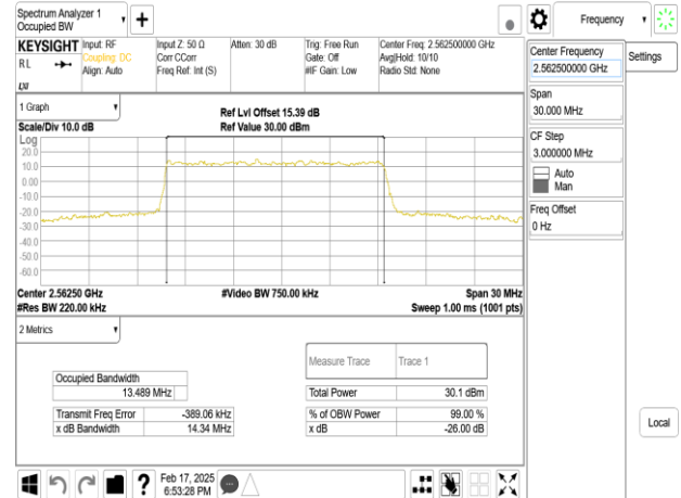
Band7_15MHz_DFT_s_OFDM_SCS15kHz_16QAM_RB75_0_CH512500
