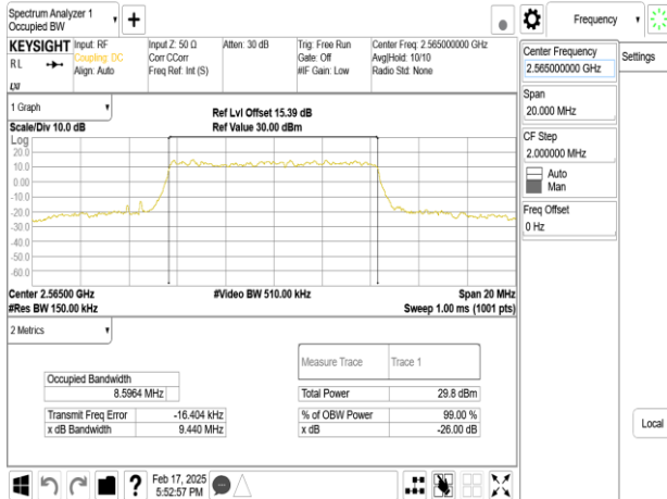
Band7_10MHz_DFT_s_OFDM_SCS30kHz_16QAM_RB24_0_CH513000
