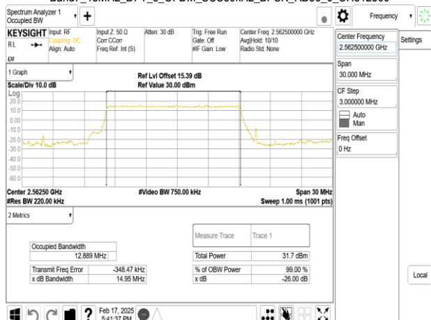
Band7_15MHz_DFT_s_OFDM_SCS30kHz_BPSK_RB36_0_CH512500
