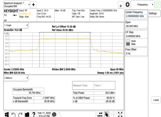
Band7_40MHz_DFT_s_OFDM_SCS30kHz_64QAM_RB100_0_CH510000
