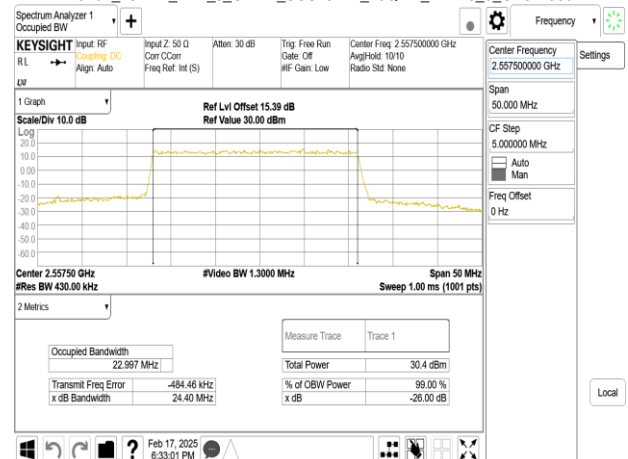
Band7_25MHz_DFT_s_OFDM_SCS15kHz_16QAM_RB128_0_CH511500
