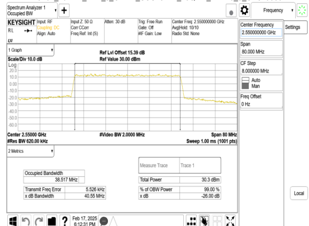
Band7_40MHz_DFT_s_OFDM_SCS15kHz_16QAM_RB216_0_CH510000
