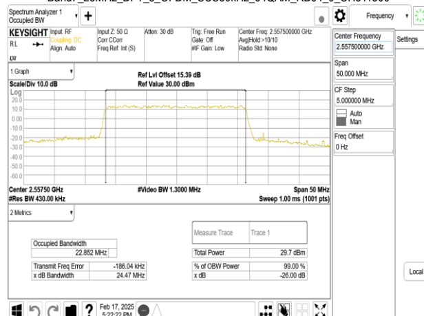
Band7_25MHz_DFT_s_OFDM_SCS30kHz_64QAM_RB64_0_CH511500
