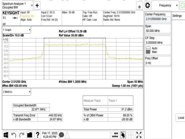
Band7_25MHz_DFT_s_OFDM_SCS15kHz_QPSK_RB128_0_CH057000
