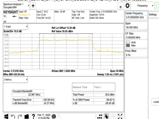
Band7_25MHz_DFT_s_OFDM_SCS30kHz_64QAM_RB64_0_CH057000
