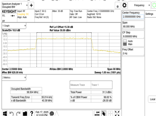
Band7_40MHz_DFT_s_OFDM_SCS15kHz_QPSK_RB216_0_CH510000
