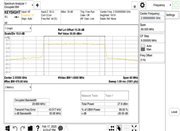
Band7_30MHz_DFT_s_OFDM_SCS15kHz_256QAM_RB160_0_CH511000
