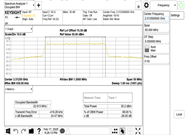
Band7_25MHz_DFT_s_OFDM_SCS15kHz_16QAM_RB128_0_CH057000
