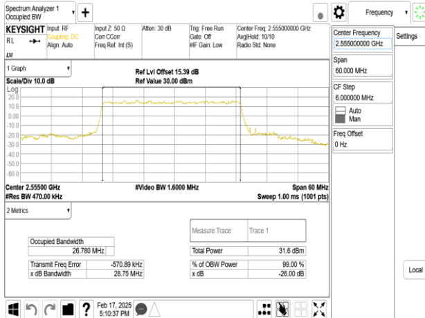
Band7_30MHz_DFT_s_OFDM_SCS30kHz_BPSK_RB75_0_CH511000
