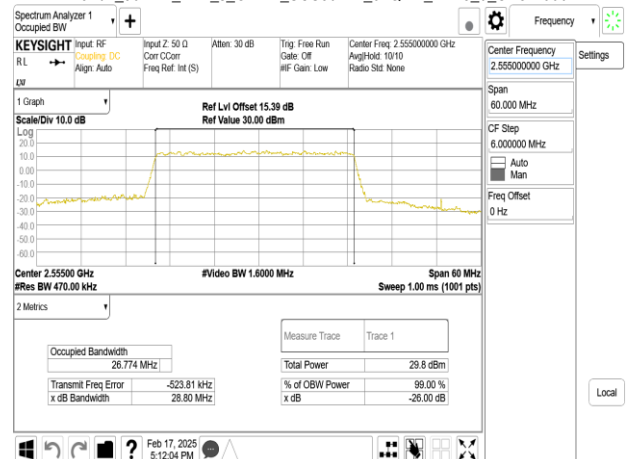
Band7_30MHz_DFT_s_OFDM_SCS30kHz_64QAM_RB75_0_CH511000
