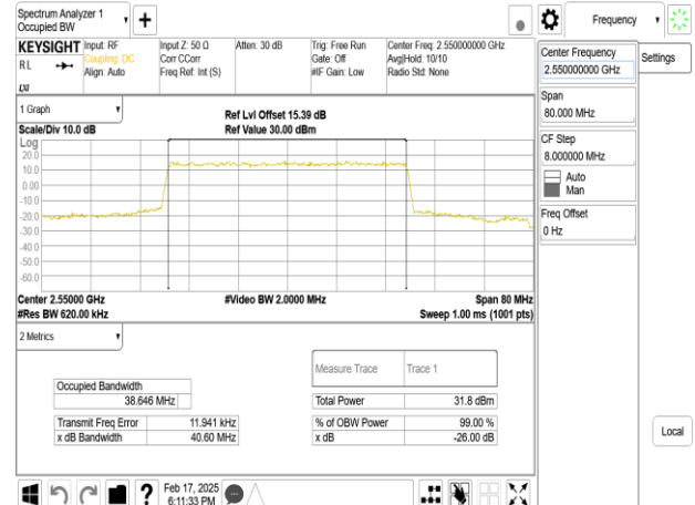
Band7_40MHz_DFT_s_OFDM_SCS15kHz_BPSK_RB216_0_CH510000
