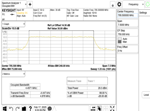
Band14_5MHz_DFT_s_OFDM_SCS15kHz_16QAM_RB25_0_CH159100
