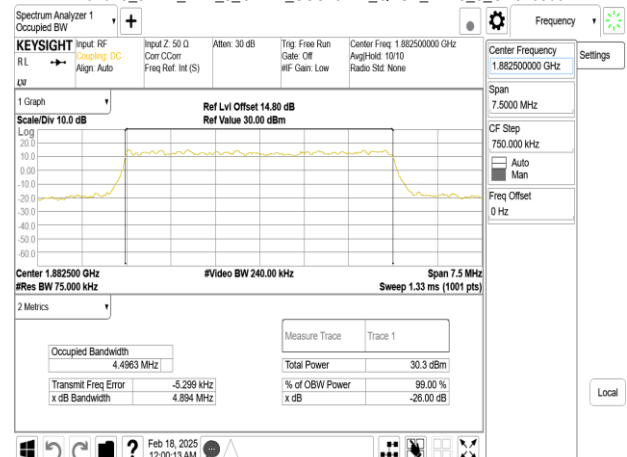
Band25_5MHz_DFT_s_OFDM_SCS15kHz_QPSK_RB25_0_CH376500
