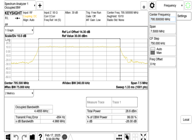
Band14_5MHz_DFT_s_OFDM_SCS15kHz_64QAM_RB25_0_CH159100
