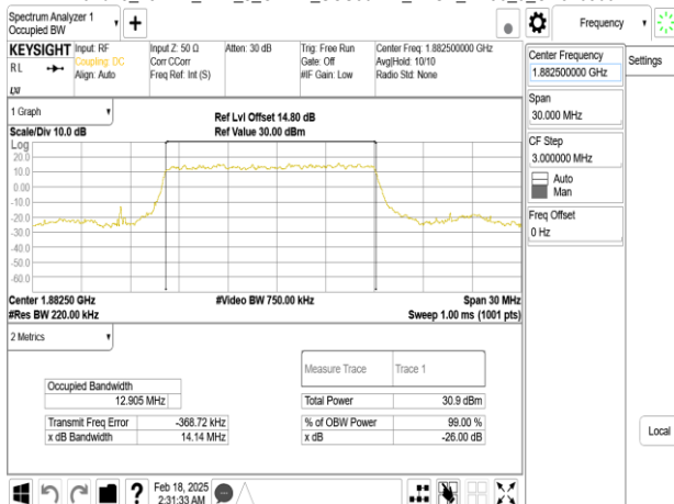
Band25_15MHz_DFT_s_OFDM_SCS30kHz_BPSK_RB36_0_CH376500
