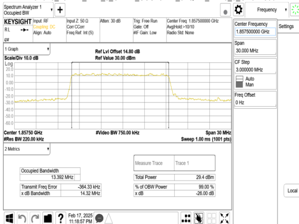
Band25_15MHz_DFT_s_OFDM_SCS15kHz_64QAM_RB75_0_CH376500
