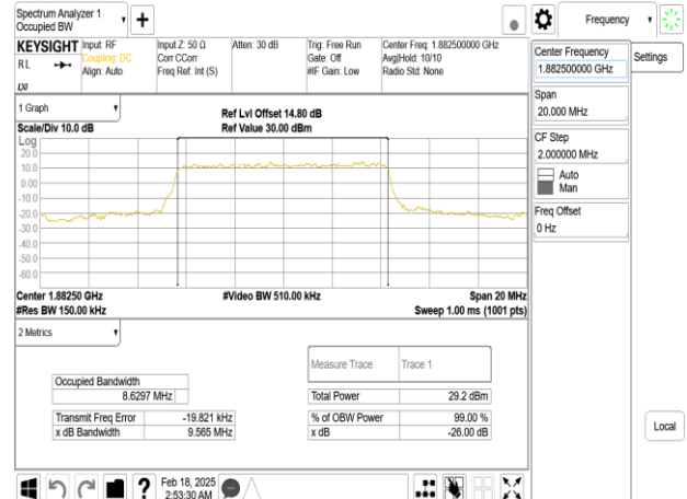
Band25_10MHz_DFT_s_OFDM_SCS30kHz_64QAM_RB24_0_CH376500
