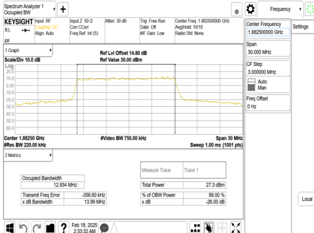
Band25_15MHz_DFT_s_OFDM_SCS30kHz_256QAM_RB36_0_CH376500
