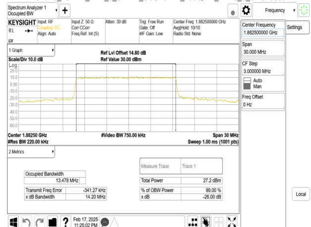
Band25_15MHz_DFT_s_OFDM_SCS15kHz_256QAM_RB75_0_CH376500
