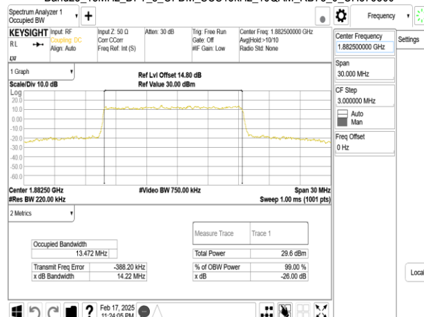
Band25_15MHz_DFT_s_OFDM_SCS15kHz_16QAM_RB75_0_CH376500
