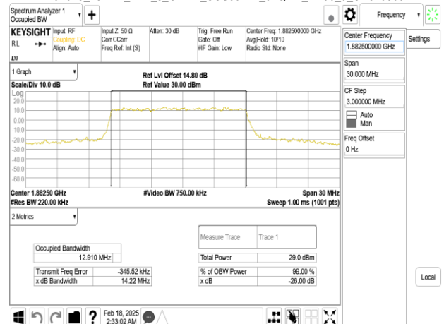
Band25_15MHz_DFT_s_OFDM_SCS30kHz_64QAM_RB36_0_CH376500
