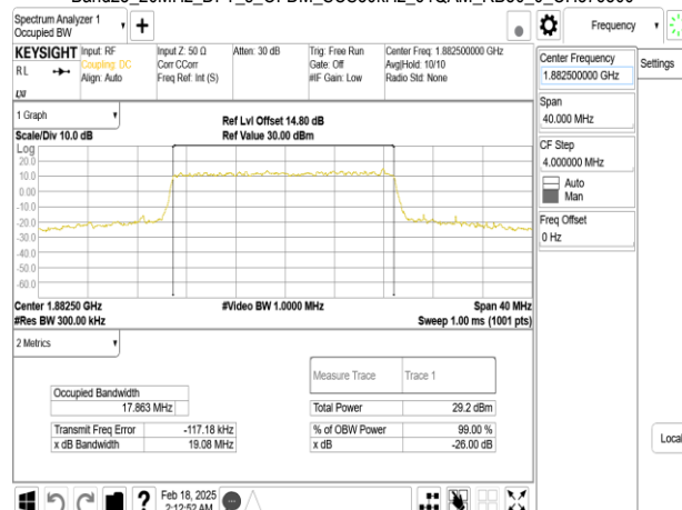
Band25_20MHz_DFT_s_OFDM_SCS30kHz_64QAM_RB50_0_CH376500
