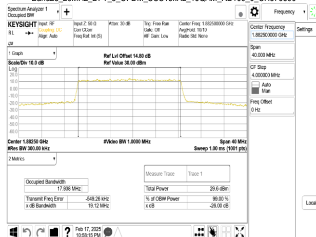
Band25_20MHz_DFT_s_OFDM_SCS15kHz_16QAM_RB100_0_CH376500
