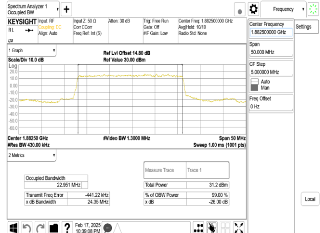
Band25_25MHz_DFT_s_OFDM_SCS15kHz_BPSK_RB128_0_CH376500
