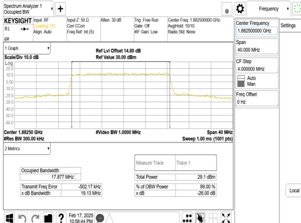
Band25_20MHz_DFT_s_OFDM_SCS15kHz_64QAM_RB100_0_CH376500
