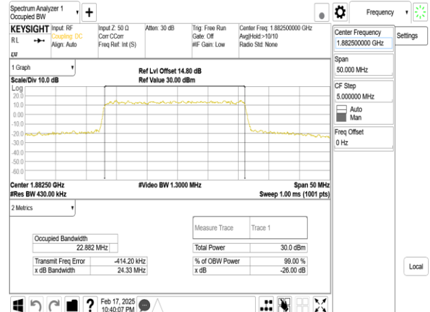
Band25_25MHz_DFT_s_OFDM_SCS15kHz_16QAM_RB128_0_CH376500
