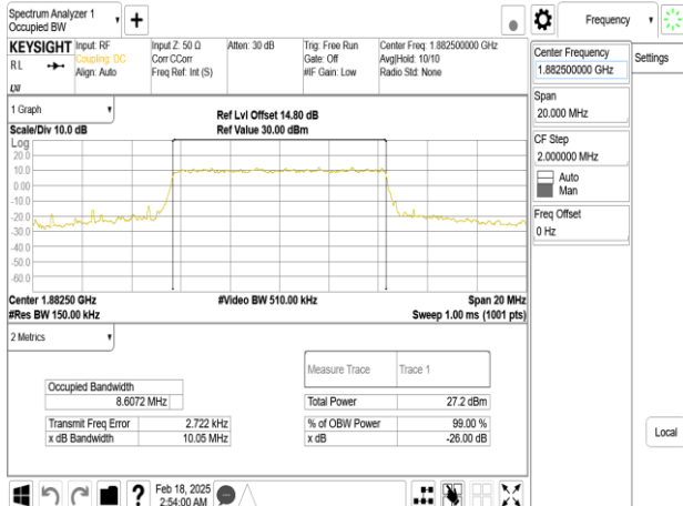
Band25_10MHz_DFT_s_OFDM_SCS30kHz_256QAM_RB24_0_CH376500
