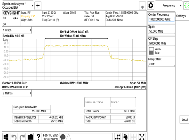
Band25_25MHz_DFT_s_OFDM_SCS15kHz_QPSK_RB128_0_CH376500
