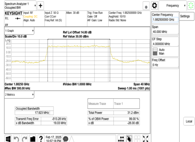
Band25_20MHz_DFT_s_OFDM_SCS15kHz_BPSK_RB100_0_CH376500
