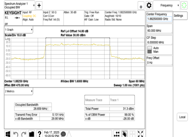
Band25_30MHz_DFT_s_OFDM_SCS15kHz_BPSK_RB160_0_CH376500
