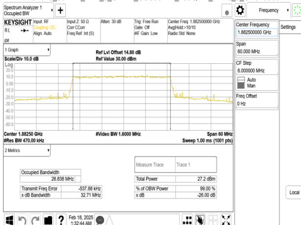
Band25_30MHz_DFT_s_OFDM_SCS30kHz_256QAM_RB75_0_CH376500
