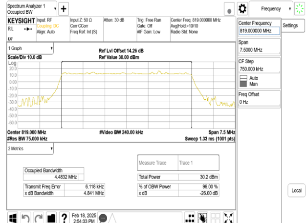
Band26-Part90s_5MHz_DFT_s_OFDM_SCS15kHz_BPSK_RB25_0_CH163800
