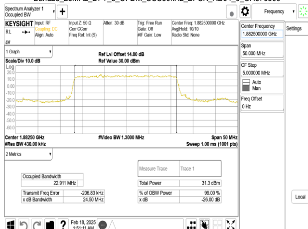
Band25_25MHz_DFT_s_OFDM_SCS30kHz_BPSK_RB64_0_CH376500
