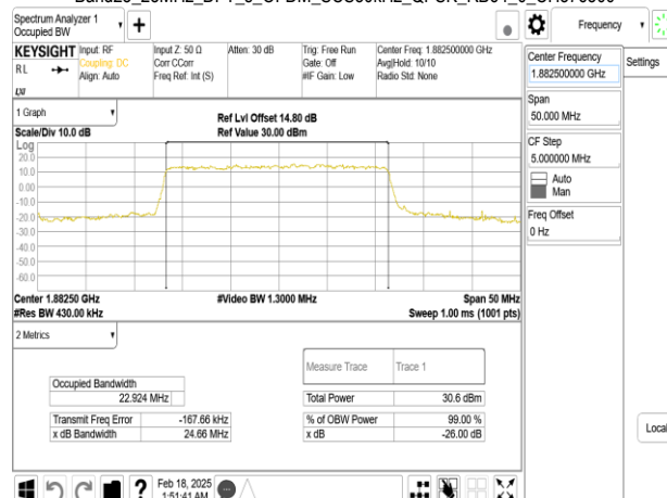
Band25_25MHz_DFT_s_OFDM_SCS30kHz_QPSK_RB64_0_CH376500
