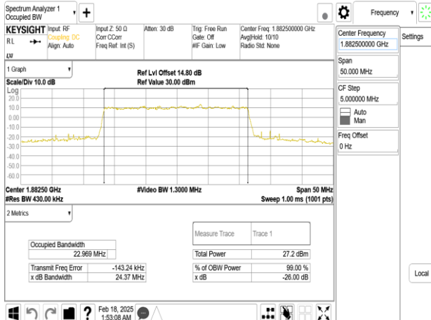
Band25_25MHz_DFT_s_OFDM_SCS30kHz_256QAM_RB64_0_CH376500
