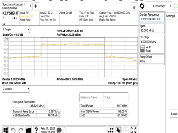
Band25_40MHz_DFT_s_OFDM_SCS15kHz_QPSK_RB216_0_CH376500
