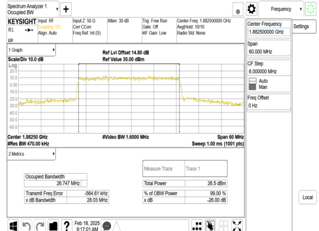
Band25_30MHz_DFT_s_OFDM_SCS30kHz_64QAM_RB75_0_CH376500
