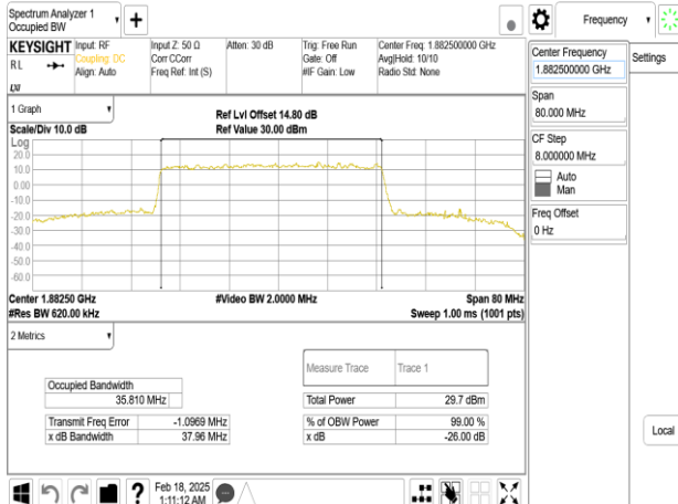
Band25_40MHz_DFT_s_OFDM_SCS30kHz_16QAM_RB100_0_CH376500
