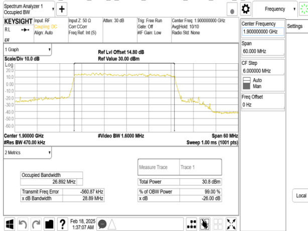
Band25_30MHz_DFT_s_OFDM_SCS30kHz_16QAM_RB75_0_CH373000
