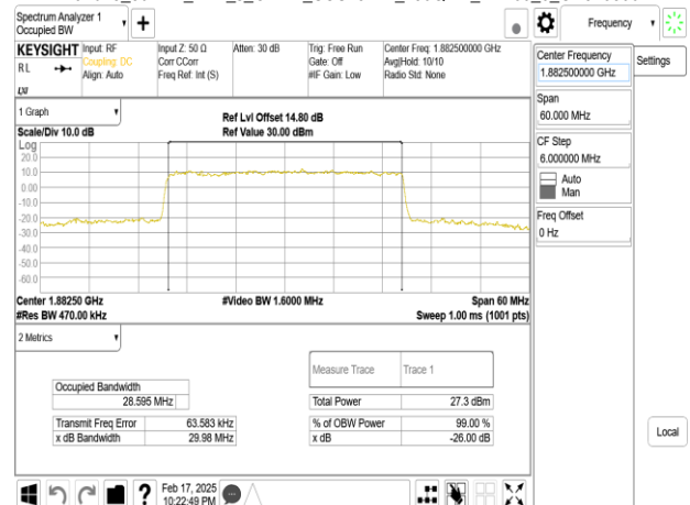
Band25_30MHz_DFT_s_OFDM_SCS15kHz_256QAM_RB160_0_CH376500
