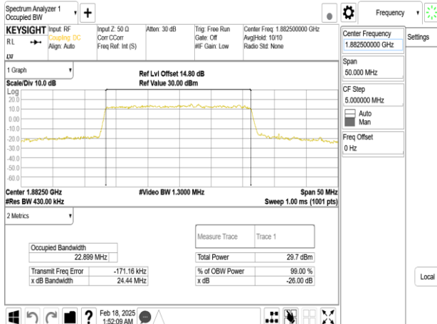
Band25_25MHz_DFT_s_OFDM_SCS30kHz_16QAM_RB64_0_CH376500
