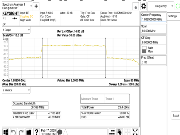
Band25_40MHz_DFT_s_OFDM_SCS15kHz_64QAM_RB216_0_CH376500
