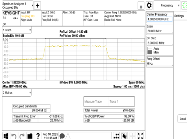
Band25_30MHz_DFT_s_OFDM_SCS30kHz_16QAM_RB75_0_CH376500
