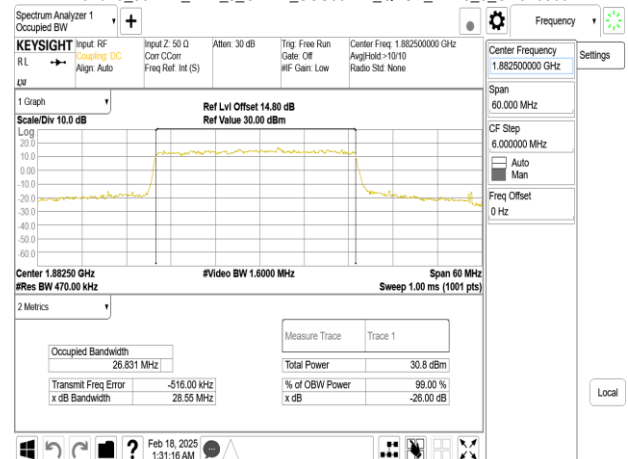
Band25_30MHz_DFT_s_OFDM_SCS30kHz_QPSK_RB75_0_CH376500
