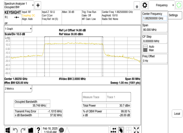
Band25_40MHz_DFT_s_OFDM_SCS30kHz_QPSK_RB100_0_CH376500
