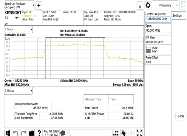
Band25_40MHz_DFT_s_OFDM_SCS30kHz_64QAM_RB100_0_CH376500
