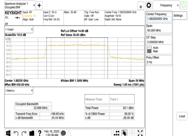
Band25_25MHz_DFT_s_OFDM_SCS30kHz_64QAM_RB64_0_CH376500
