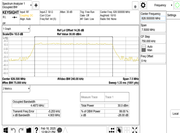
Band26_5MHz_DFT_s_OFDM_SCS15kHz_QPSK_RB25_0_CH165300
