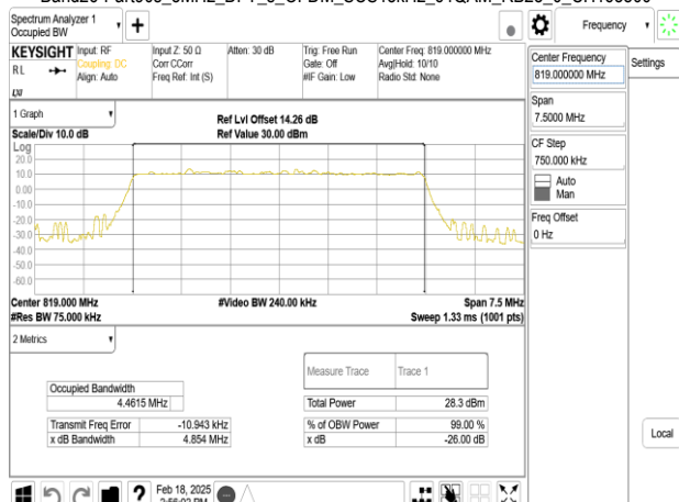
Band26-Part90s_5MHz_DFT_s_OFDM_SCS15kHz_64QAM_RB25_0_CH163800
