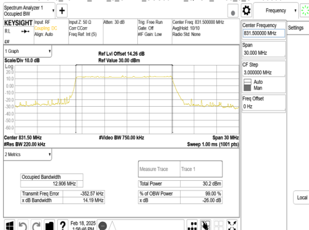
Band26_15MHz_DFT_s_OFDM_SCS30kHz_QPSK_RB36_0_CH166300
