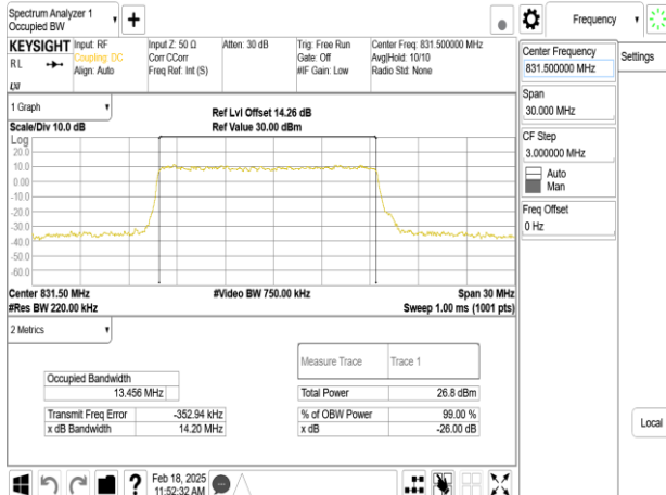
Band26_15MHz_DFT_s_OFDM_SCS15kHz_256QAM_RB75_0_CH166300
