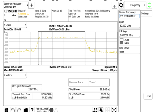
Band26_15MHz_DFT_s_OFDM_SCS30kHz_16QAM_RB36_0_CH166300
