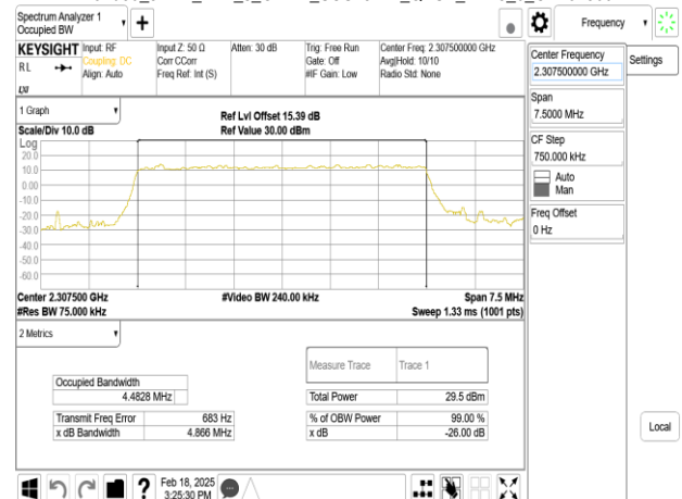
Band30_5MHz_DFT_s_OFDM_SCS15kHz_QPSK_RB25_0_CH461500
