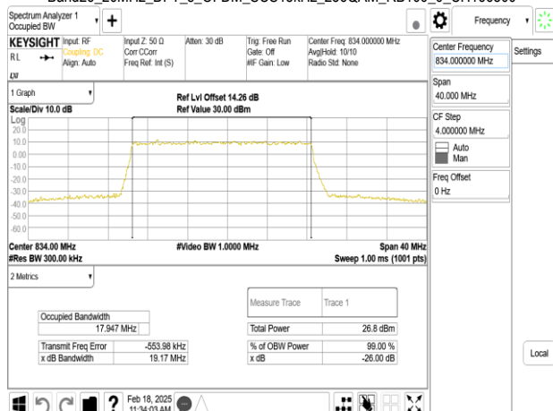
Band26_20MHz_DFT_s_OFDM_SCS15kHz_256QAM_RB100_0_CH166800
