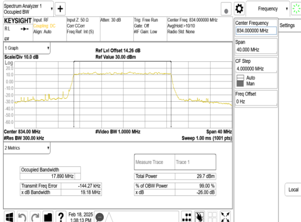
Band26_20MHz_DFT_s_OFDM_SCS30kHz_QPSK_RB50_0_CH166800
