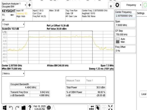
Band30_5MHz_DFT_s_OFDM_SCS15kHz_BPSK_RB25_0_CH461500
