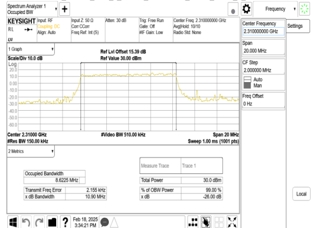
Band30_10MHz_DFT_s_OFDM_SCS30kHz_QPSK_RB24_0_CH462000
