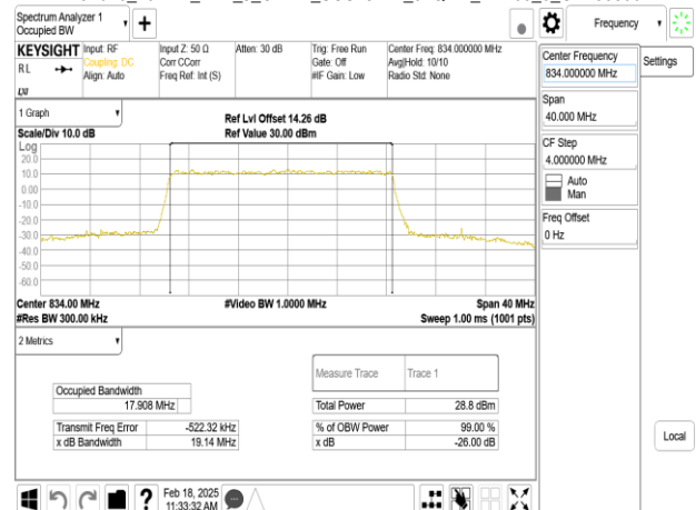
Band26_20MHz_DFT_s_OFDM_SCS15kHz_64QAM_RB100_0_CH166800
