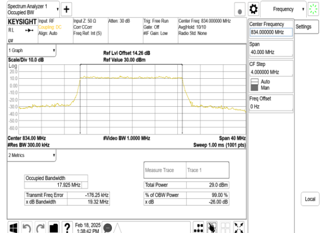
Band26_20MHz_DFT_s_OFDM_SCS30kHz_16QAM_RB50_0_CH166800
