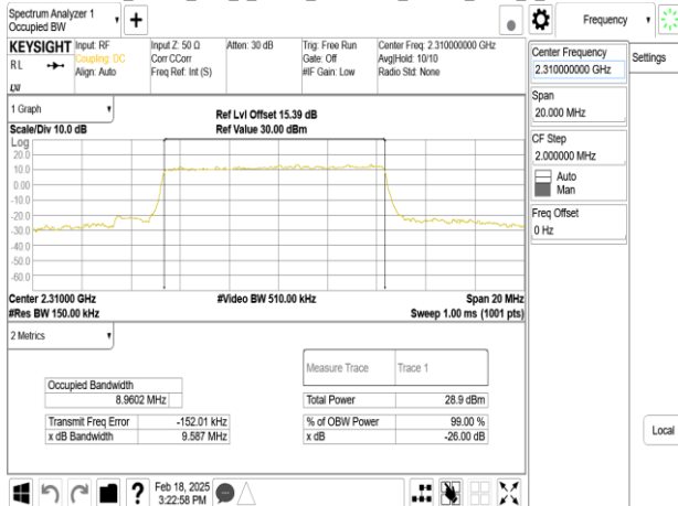
Band30_10MHz_DFT_s_OFDM_SCS15kHz_64QAM_RB50_0_CH462000
