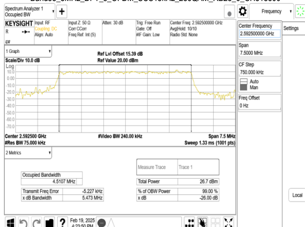
Band38_5MHz_DFT_s_OFDM_SCS15kHz_256QAM_RB25_0_CH518500
