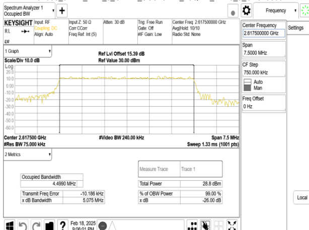
Band38_5MHz_DFT_s_OFDM_SCS15kHz_16QAM_RB25_0_CH523500
