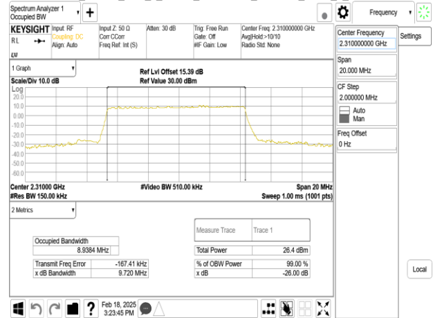
Band30_10MHz_DFT_s_OFDM_SCS30kHz_BPSK_RB24_0_CH462000
