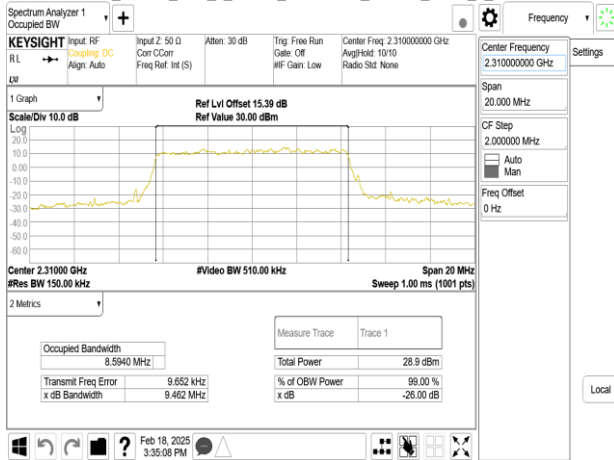
Band30_10MHz_DFT_s_OFDM_SCS30kHz_64QAM_RB24_0_CH462000
