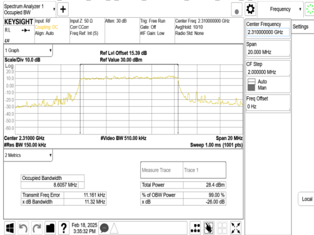
Band30_10MHz_DFT_s_OFDM_SCS30kHz_256QAM_RB24_0_CH462000
