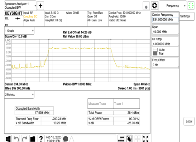
Band26_20MHz_DFT_s_OFDM_SCS30kHz_256QAM_RB50_0_CH166800
