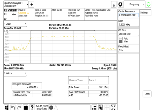
Band30_5MHz_DFT_s_OFDM_SCS15kHz_64QAM_RB25_0_CH461500
