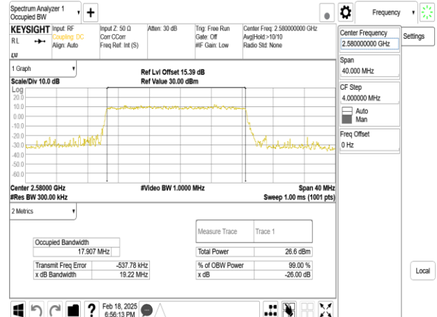
Band38_20MHz_DFT_s_OFDM_SCS15kHz_256QAM_RB100_0_CH516000
