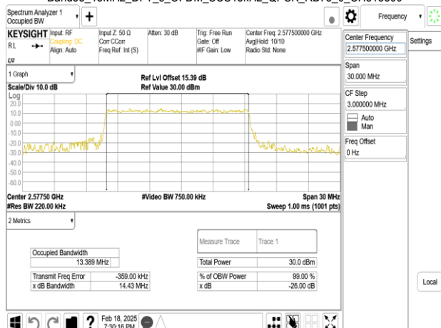
Band38_15MHz_DFT_s_OFDM_SCS15kHz_QPSK_RB75_0_CH515500
