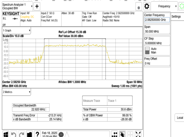
Band38_25MHz_DFT_s_OFDM_SCS30kHz_BPSK_RB64_0_CH516500
