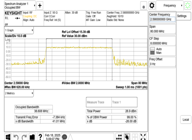
Band38_40MHz_DFT_s_OFDM_SCS15kHz_256QAM_RB216_0_CH518000
