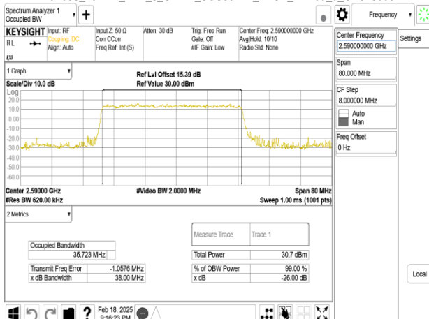
Band38_40MHz_DFT_s_OFDM_SCS30kHz_BPSK_RB100_0_CH518000
