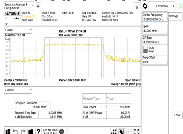
Band38_40MHz_DFT_s_OFDM_SCS30kHz_QPSK_RB100_0_CH518000
