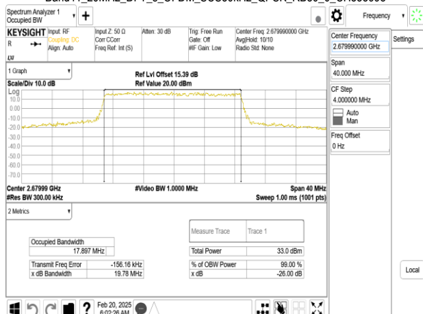
Band41_20MHz_DFT_s_OFDM_SCS30kHz_QPSK_RB50_0_CH535998
