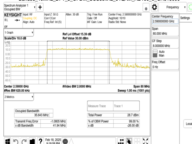
Band38_40MHz_DFT_s_OFDM_SCS30kHz_64QAM_RB100_0_CH518000
