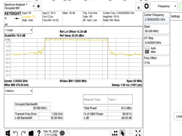
Band41_30MHz_DFT_s_OFDM_SCS15kHz_BPSK_RB160_0_CH518604
