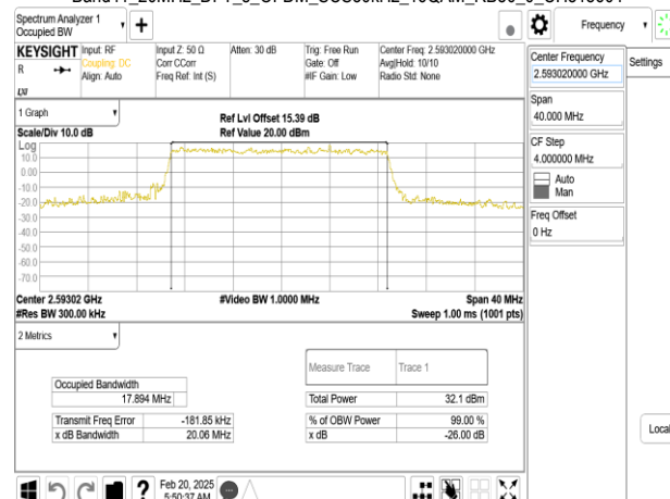
Band41_20MHz_DFT_s_OFDM_SCS30kHz_16QAM_RB50_0_CH518604
