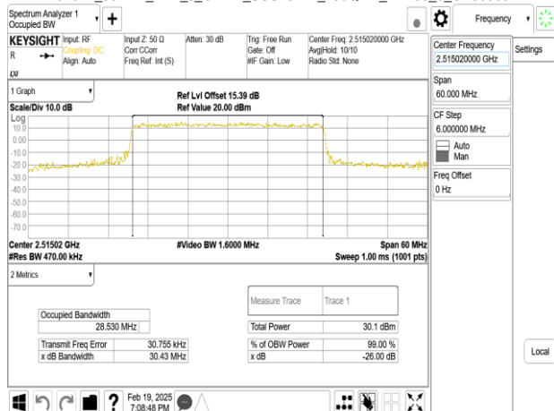
Band41_30MHz_DFT_s_OFDM_SCS15kHz_256QAM_RB160_0_CH503004
