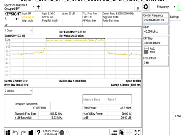
Band41_20MHz_DFT_s_OFDM_SCS30kHz_QPSK_RB50_0_CH501204
