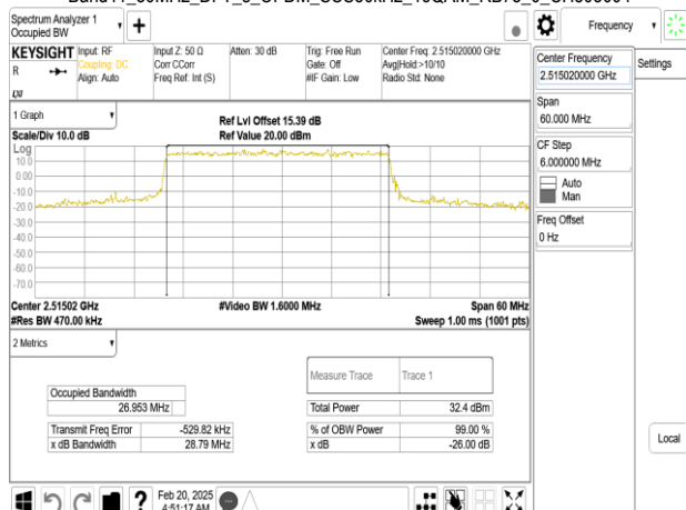
Band41_30MHz_DFT_s_OFDM_SCS30kHz_16QAM_RB75_0_CH503004
