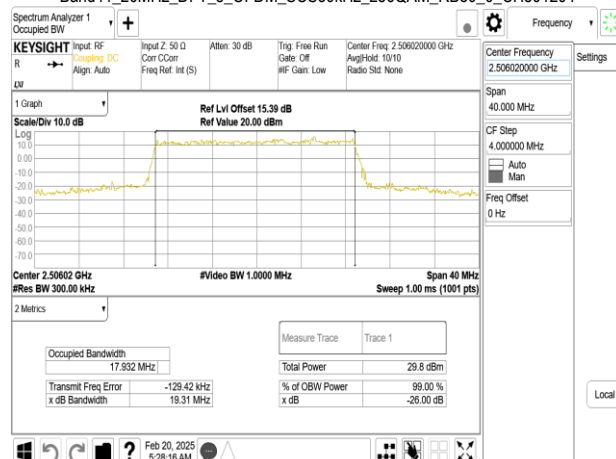
Band41_20MHz_DFT_s_OFDM_SCS30kHz_256QAM_RB50_0_CH501204
