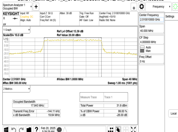
Band41_20MHz_DFT_s_OFDM_SCS30kHz_64QAM_RB50_0_CH502002
