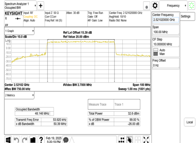
Band41_50MHz_DFT_s_OFDM_SCS15kHz_64QAM_RB270_0_CH504204
