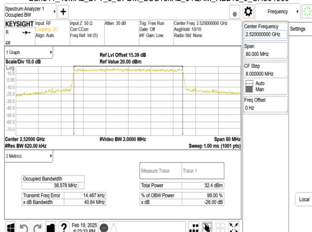
Band41_40MHz_DFT_s_OFDM_SCS15kHz_64QAM_RB216_0_CH504000
