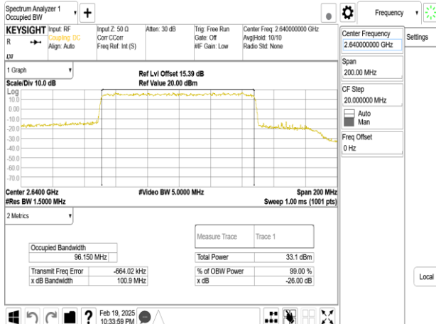
Band41_100MHz_DFT_s_OFDM_SCS30kHz_16QAM_RB270_0_CH528000
