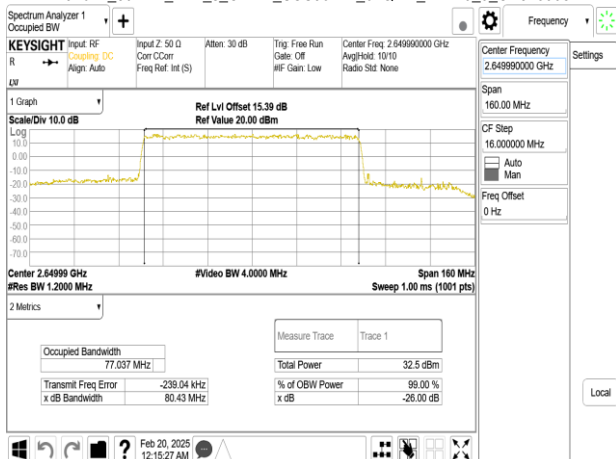
Band41_80MHz_DFT_s_OFDM_SCS30kHz_64QAM_RB216_0_CH529998
