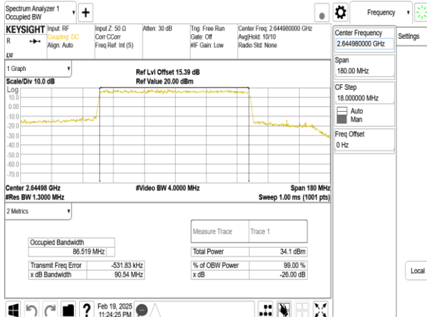
Band41_90MHz_DFT_s_OFDM_SCS30kHz_QPSK_RB243_0_CH528996
