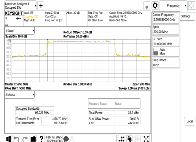
Band41_100MHz_DFT_s_OFDM_SCS30kHz_64QAM_RB270_0_CH518604
