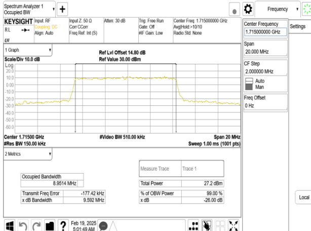
Band66_10MHz_DFT_s_OFDM_SCS15kHz_256QAM_RB50_0_CH343000
