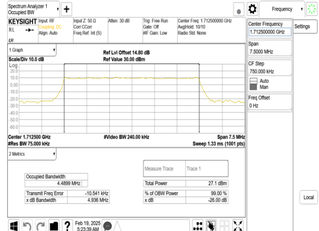
Band66_5MHz_DFT_s_OFDM_SCS15kHz_256QAM_RB25_0_CH342500
