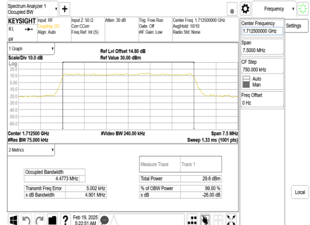
Band66_5MHz_DFT_s_OFDM_SCS15kHz_16QAM_RB25_0_CH342500
