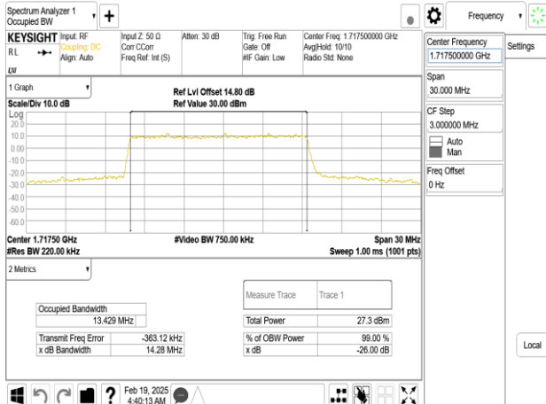
Band66_15MHz_DFT_s_OFDM_SCS15kHz_256QAM_RB75_0_CH343500
