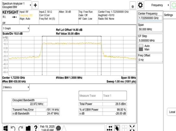
Band66_25MHz_DFT_s_OFDM_SCS30kHz_64QAM_RB64_0_CH344500
