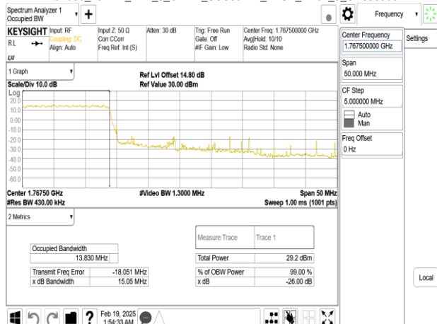
Band66_25MHz_DFT_s_OFDM_SCS30kHz_QPSK_RB64_0_CH34500
