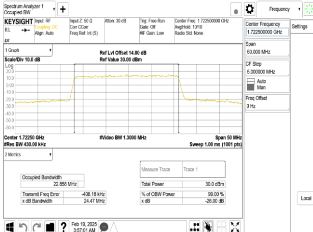
Band66_25MHz_DFT_s_OFDM_SCS15kHz_16QAM_RB128_0_CH344500
