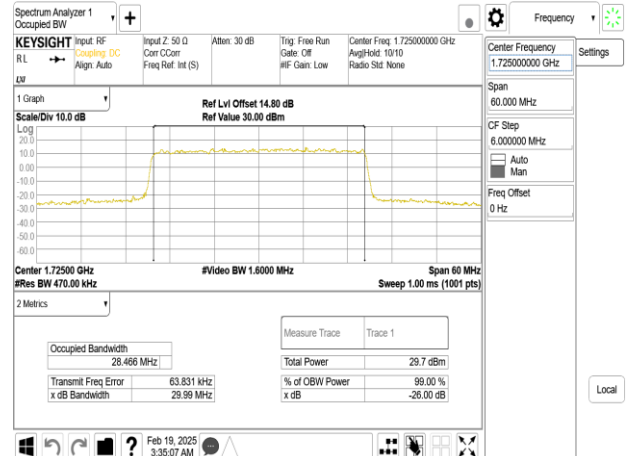
Band66_30MHz_DFT_s_OFDM_SCS15kHz_64QAM_RB160_0_CH345000
