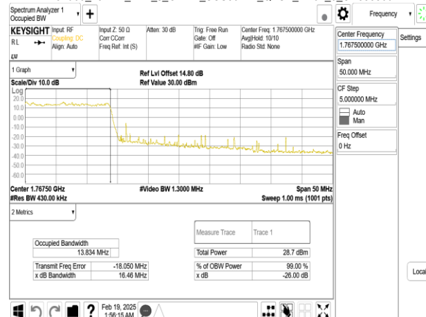
Band66_25MHz_DFT_s_OFDM_SCS30kHz_16QAM_RB64_0_CH34500
