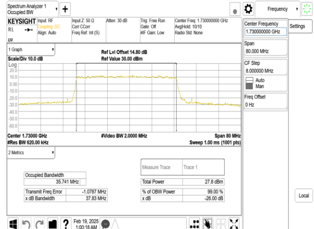
Band66_40MHz_DFT_s_OFDM_SCS30kHz_256QAM_RB100_0_CH346000
